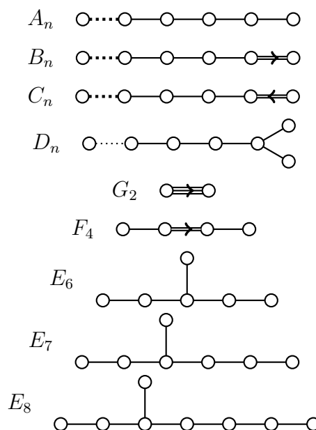
Figure 1: Dynkin diagrams of the Chevalley groups
