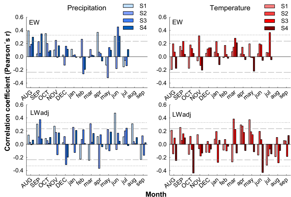
Fig. 4 Correlations (Pearson's coefficient) between earlywood (EW) and latewood adjusted ( LW_{adj} ) chronologies of Larix cajanderi with total precipitation and minimum temperature for the period 1966–2015. Correlations were calculated from August of the previous year (uppercase letters) to September of the current growth year (lowercase letters). Dashed lines indicated P < 0.05 , and dotted lines indicate P < 0.01 . Bar colors indicate the four sampled sites
