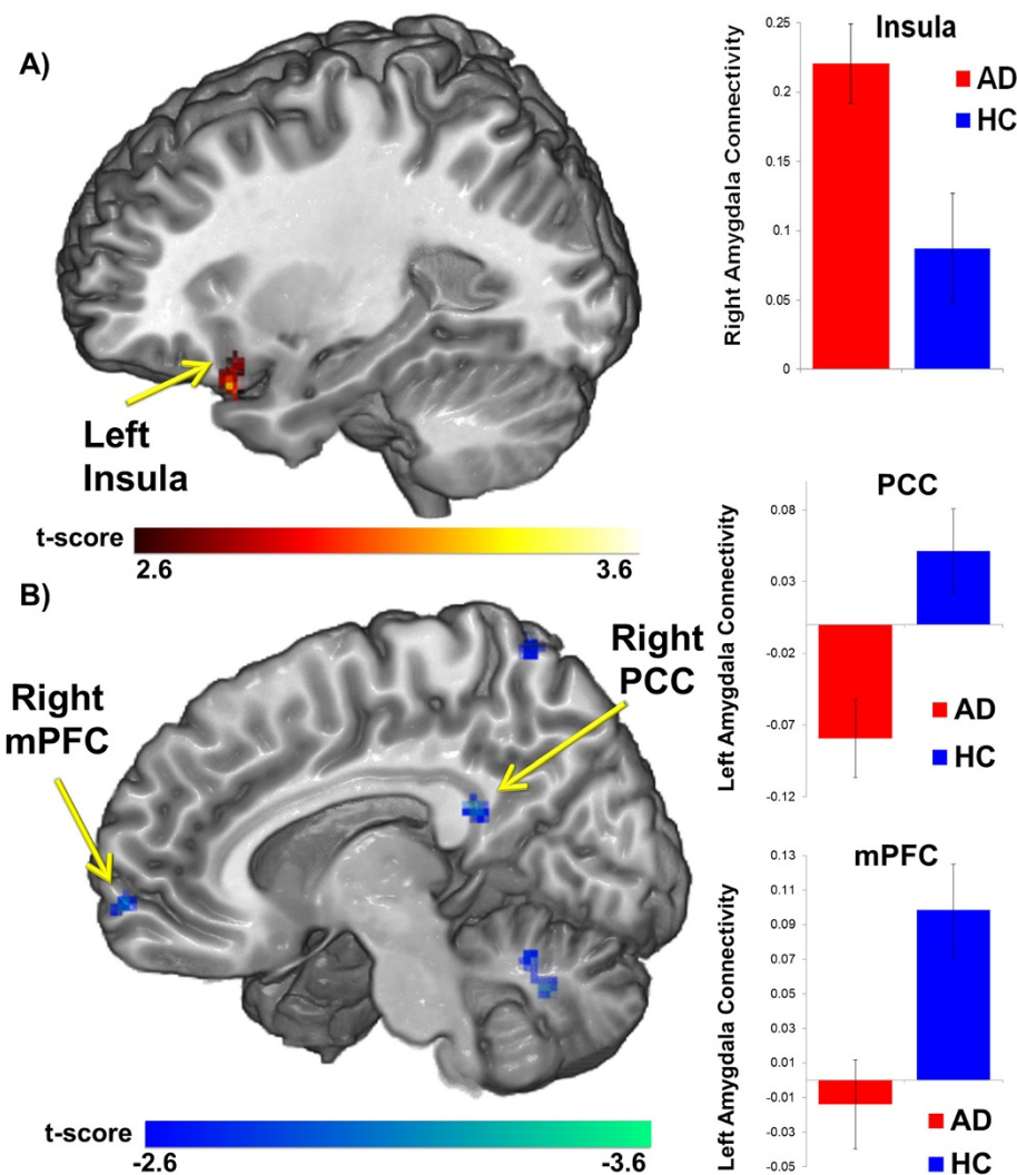
Figure 1 Between-group whole-brain voxel-wise statistical t map of a priori hypothesized group differences overlaid on a canonical brain rendering showing: (A) greater right amygdala connectivity to the insula (anxiety disorder (AD) group > healthy control (HC) group; and (B) decreased amygdala connectivity to the medial prefrontal cortex (mPFC) and posterior cingulate cortex (PCC) (AD < HC). Statistical t map thresholded at whole-brain voxel-wise ( p < 0.005 , cluster volume > 352 \text{ mm}^3 , representing corrected \alpha < 0.05 ); color bar represents statistical t scores. Bar graph shows mean extracted parameter estimate \beta weights in arbitrary units ( \pm SEM) within each group from 10 mm spherical region of interest surrounding peak.
