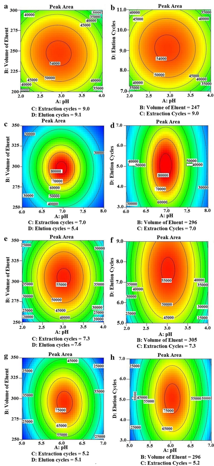
Fig. 3 Response surface -2D contours showing the effect of independent variable on the extraction efficiency of dyes. a and b for MG, c and d for MO, e and f for RB and g and h for AR
