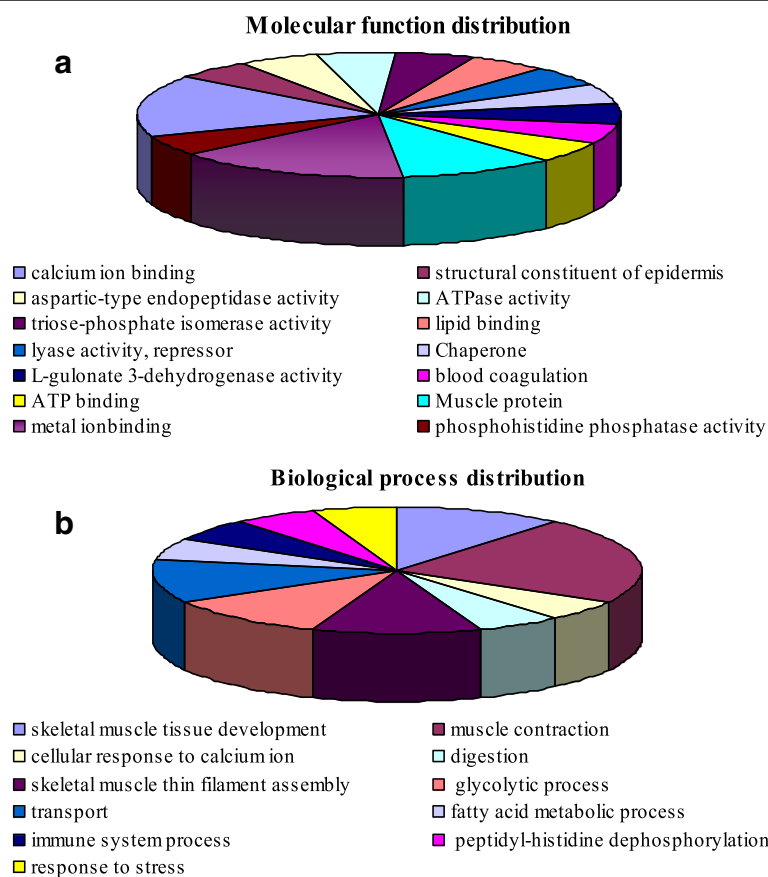
Fig. 2 GO annotation of different proteinic spots ( a : molecular function distribution, b : Biological process distribution)
