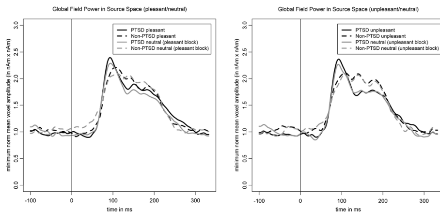
Figure 2 This figure presents the global field power in source space averaged separately for the PTSD (solid lines) and Non-PTSD (dashed lines) group and separately for the picture category (black lines = high arousing emotional stimuli; grey lines = neutral stimuli). Stimulus onset is the time point 0, indicated by the vertical line. PTSD = Posttraumatic Stress Disorder.
