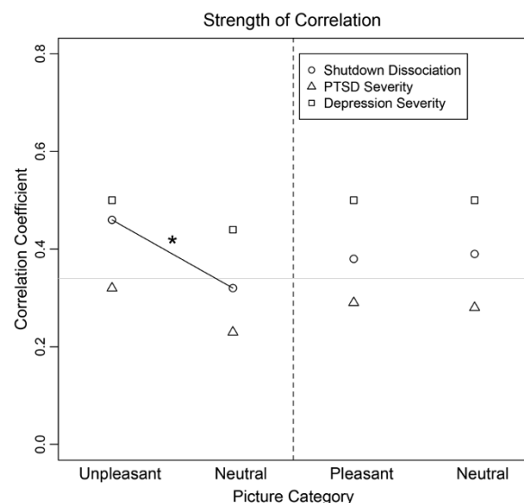
Figure 3 This figure presents the Pearson correlation coefficient between the surface minimum-norm estimate in source space and the psychopathological scale (circle: Shutdown dissociation; triangle: Posttraumatic Stress Disorder (PTSD) symptom severity; rectangle: Depression symptom severity) as a function of picture category. The grey horizontal line presents the significance level indicating significant correlations above the line. The dashed line separates the blocks presenting the results of the unpleasant/neutral block at the left side and the results of the pleasant/neutral block at the right side. The black solid line and * indicate the significant difference between the correlation coefficient.
