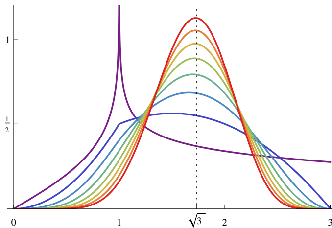
Figure 1: p_3(\nu; x) for \nu = 0, \frac{1}{2}, 1, \dots, \frac{7}{2}
