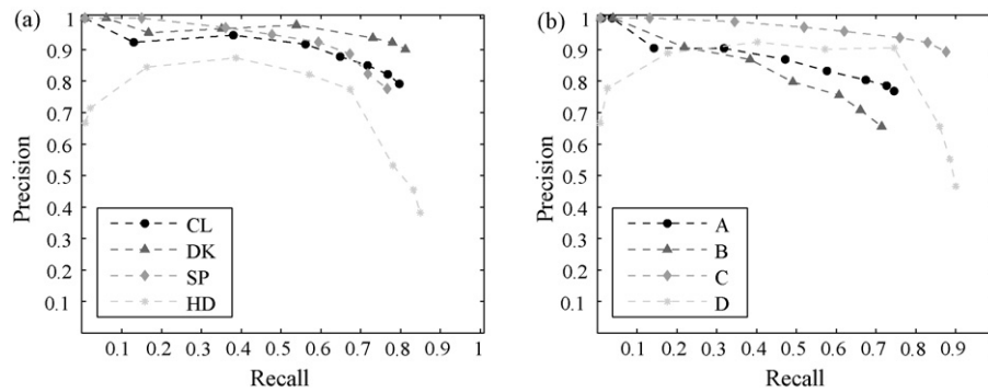
Figure 4 Movement study: user-specific PR analysis (confidence threshold sweep) of the event fusion results using the COMP method. Best performance is found towards the top-right corner (high precision, high recall). (a) Analysis for every category (CL: cutlery, DK: drink, SP: spoon, HD: hand only). (b) Analysis for every study participant (A–D).
