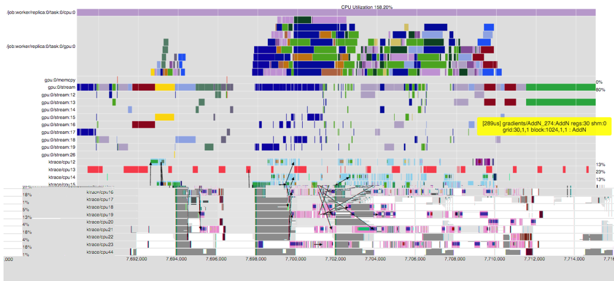
Figure 14: Timeline of multi-stream GPU execution.
