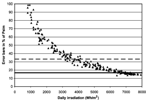
Fig. 17. Minimum required energy loss for daily values for a reliable detection of the example inverter failure.
