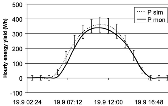
Fig. 19. Shading example at a Dutch system.
