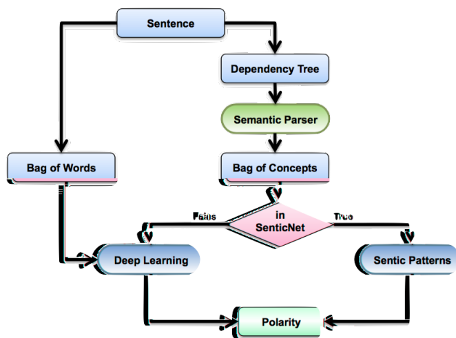
Figure 7: Sentic computing framework.
