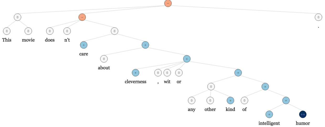
Figure 9: RNTN applied on the dependency tree of the sentence “This movie doesn’t care about cleverness, wit or any other kind of intelligent humor”.
