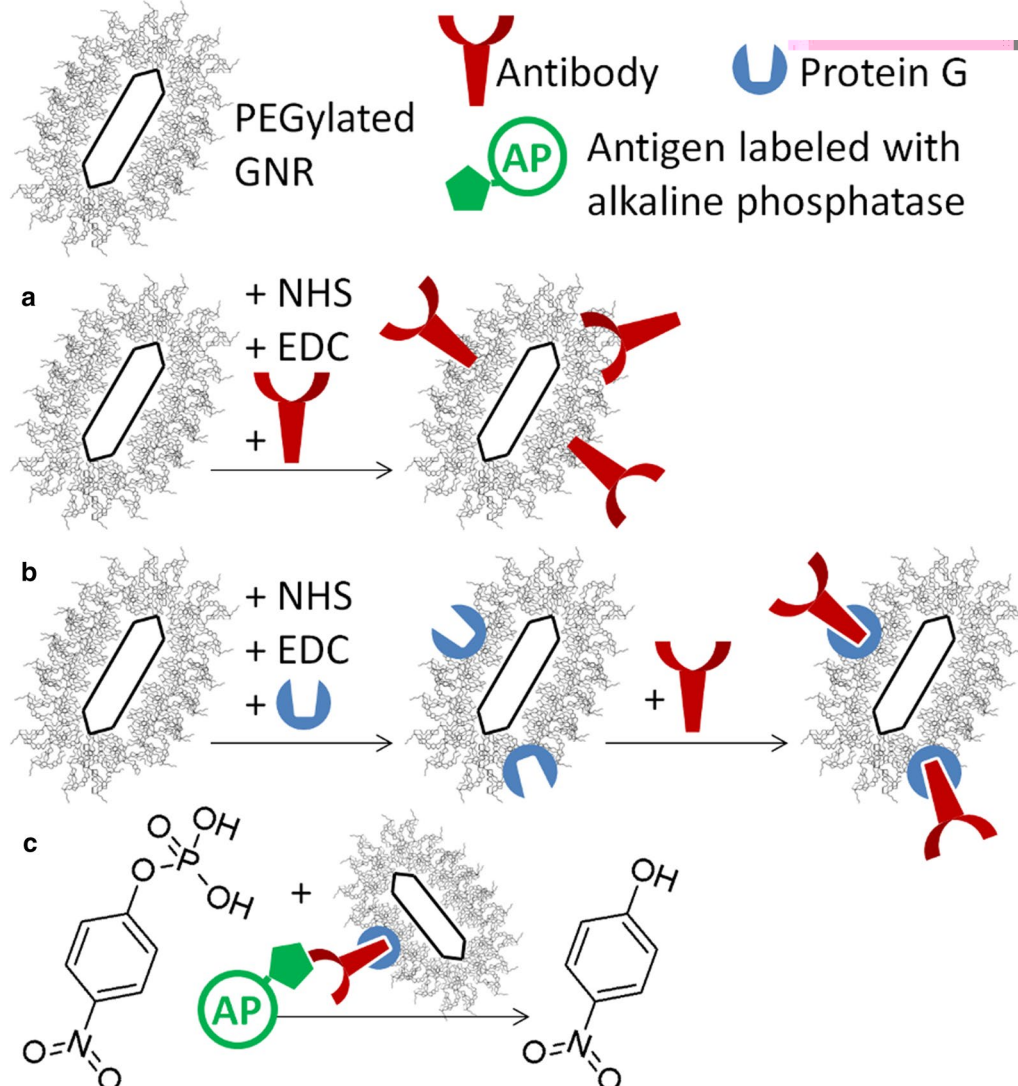
Fig. 1 Schematic representation of covalent and oriented immobilization of antibodies onto PEGylated GNRs in a and b , respectively. The hydrolysis of the enzymatic substrate 4-NPP to 4-NP catalysed by the enzyme bound to the particles after the antibody-antigen recognition is pictured in c
