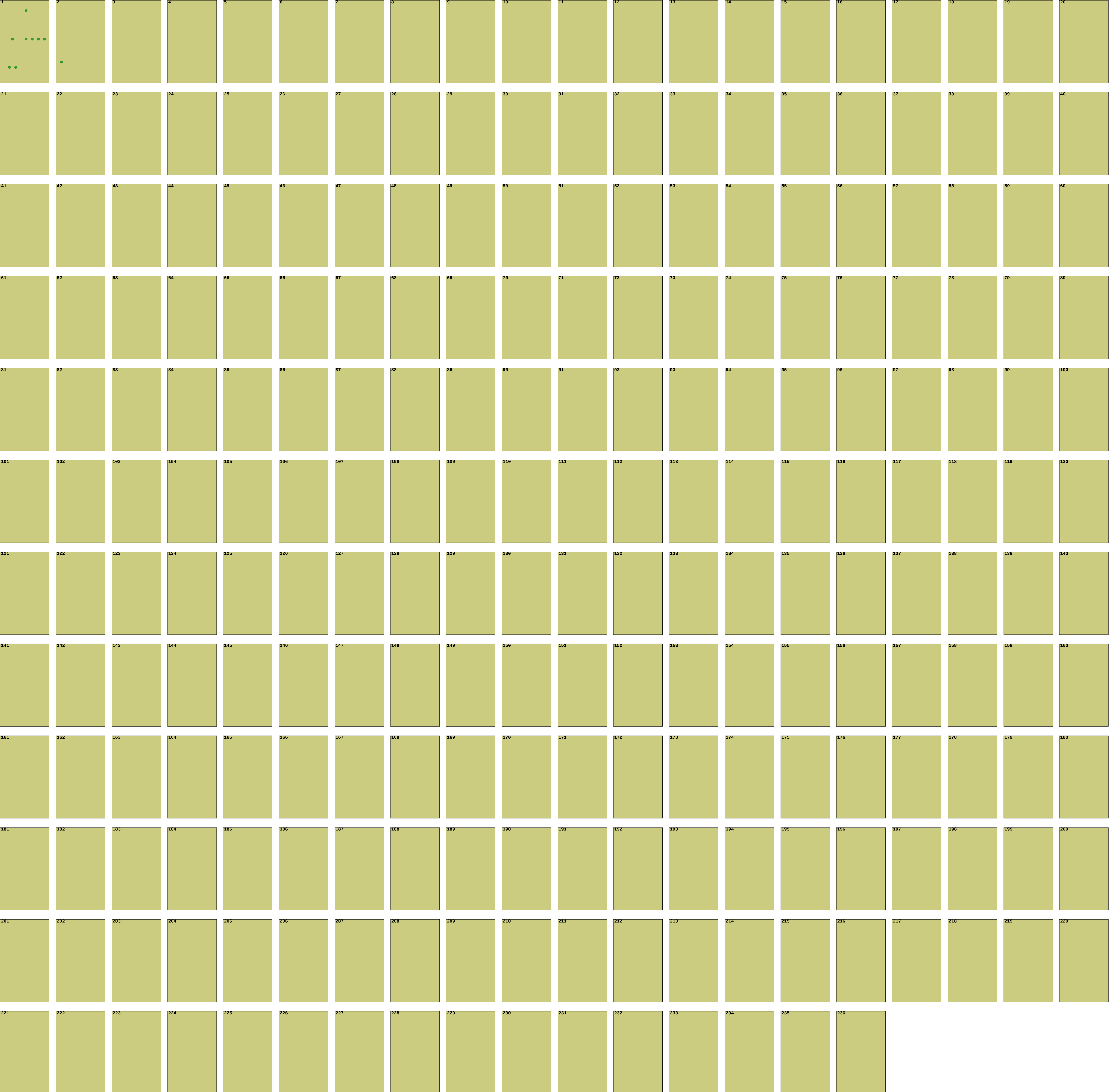
Connected graphs - 8 nodes, 9 edges Keith Briggs 2004 Jan 22 11:32
