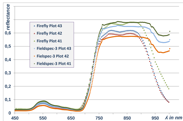
Figure 7-6: FieldSpec3 spectra versus UHD185 spectra for plots 41, 42, and 43 on 14 June 2013.
