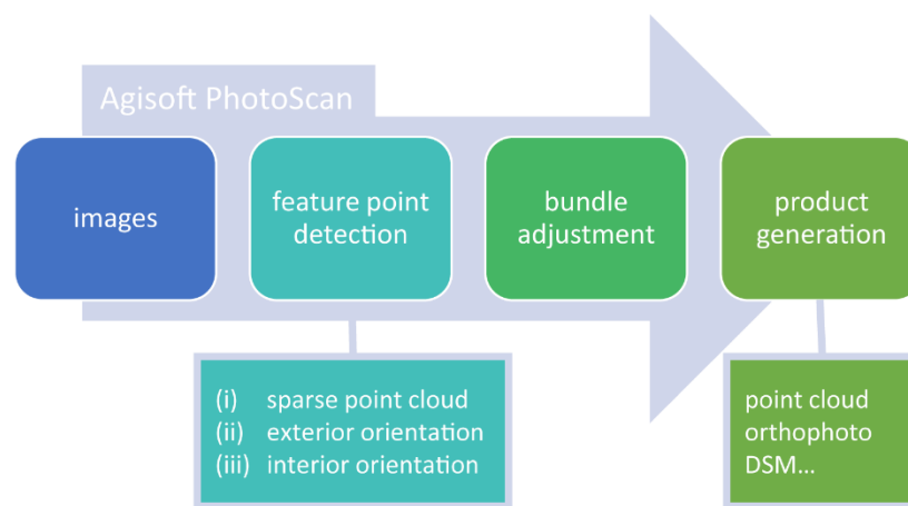
Figure 2-3: Image processing workflow with Agisoft PhotoScan.
