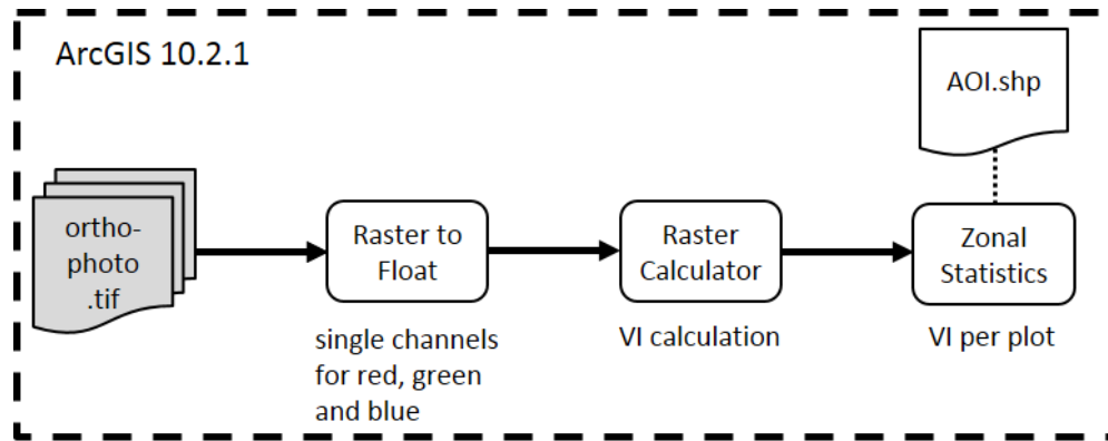
Figure 6-2: Workflow for VI_{VIS} calculation. (AOI = old and new cultivars in Table 6-2).
