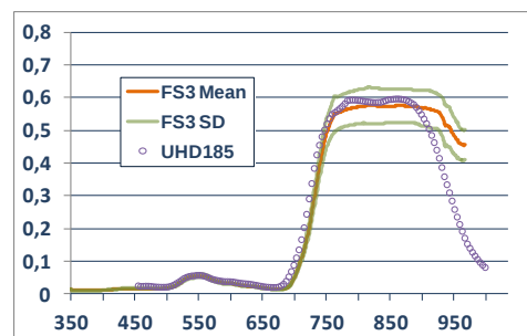
Figure 7-8: Mean FieldSpec3 spectrum for plot 42 with standard deviation (SD) and mean UHD185 spectrum for 14 June 2013.
