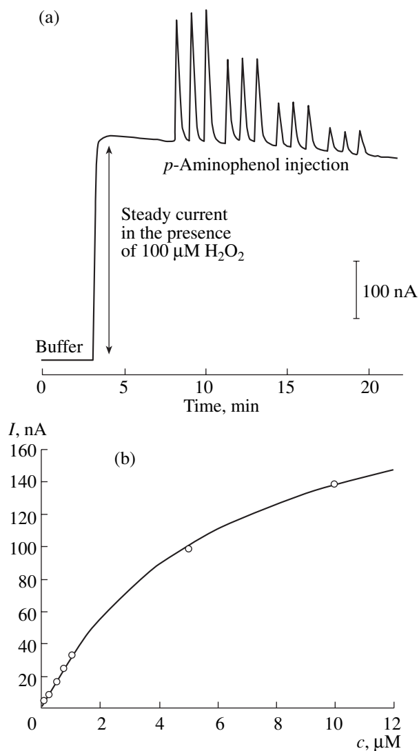
Fig. 4. Determination of aromatic phenols and amines in a flow-injection cell using HRP immobilized on a graphite electrode [18]: (a) shape of primary experimental data; (b) approximation by the Michaelis-Menten equation for p -aminophenol. Hydrogen peroxide concentration of 100 \mu M.
