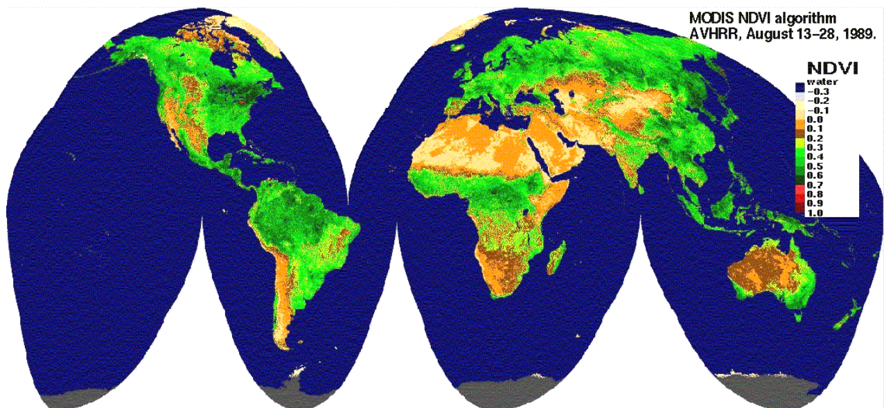
Figure 3.2.11: Global NDVI image (pseudo color) using the MODIS VI composite algorithm (BRDF/ CV-MVC/ MVC approach).
