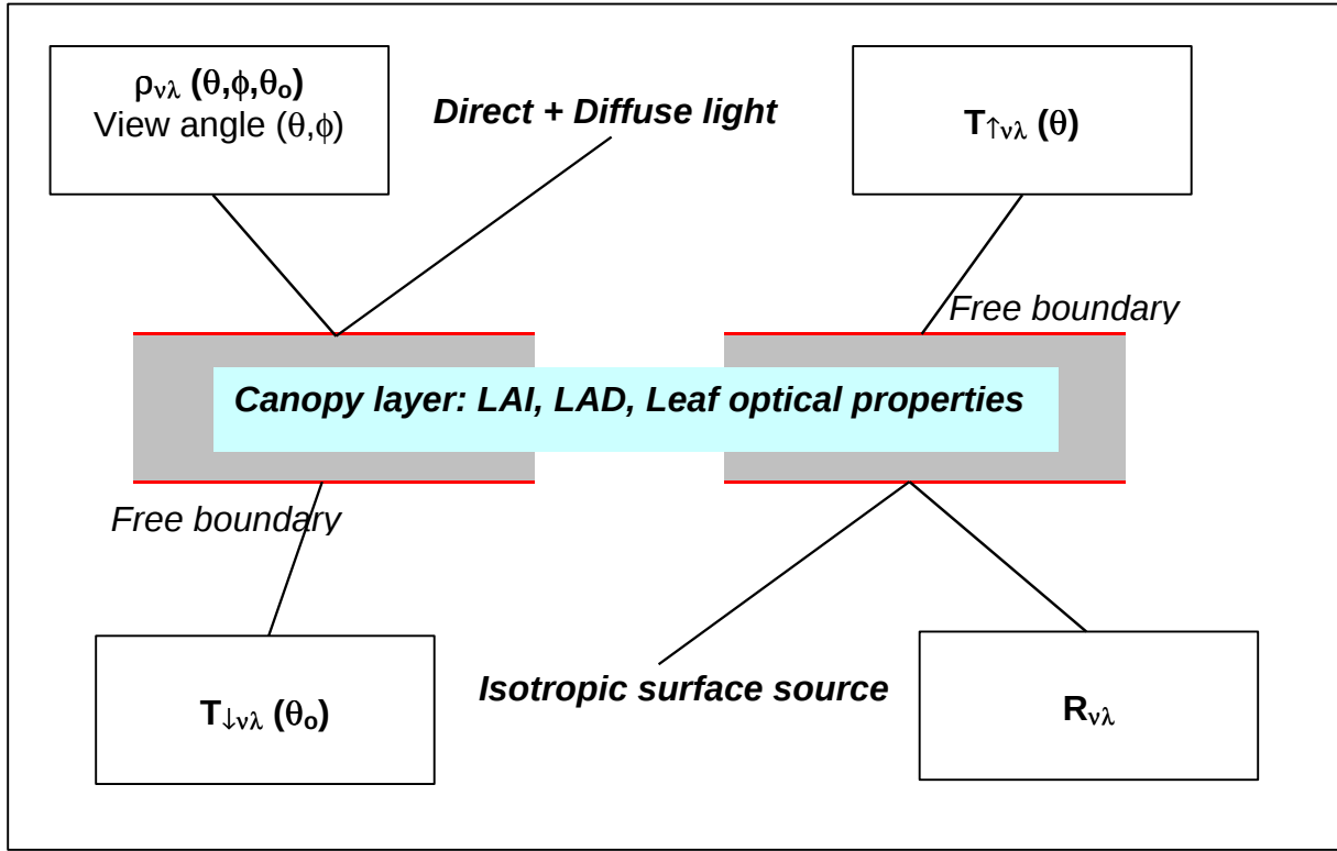
Figure 3.1.4: Illustration of canopy optical properties r_{vl} , R_{vl} , T_{-vl}(q_0) and T_{-vl}(q)
