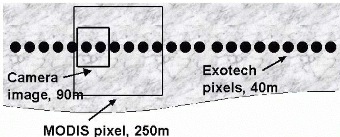
Figure 3.5.2: Diagram of Exotech and camera airborne data acquisitions in relation to a MODIS pixel for 150 m AGL and 15^\circ field-of-view Exotech.
