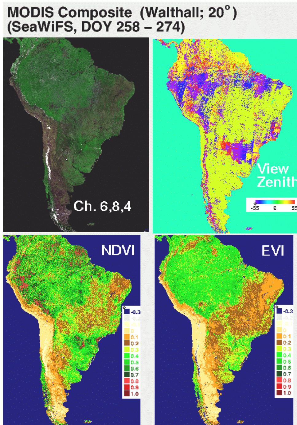
Figure 3.2.15: SEAWIFS color composite, NDVI, EVI and view angle distribution for South America.
