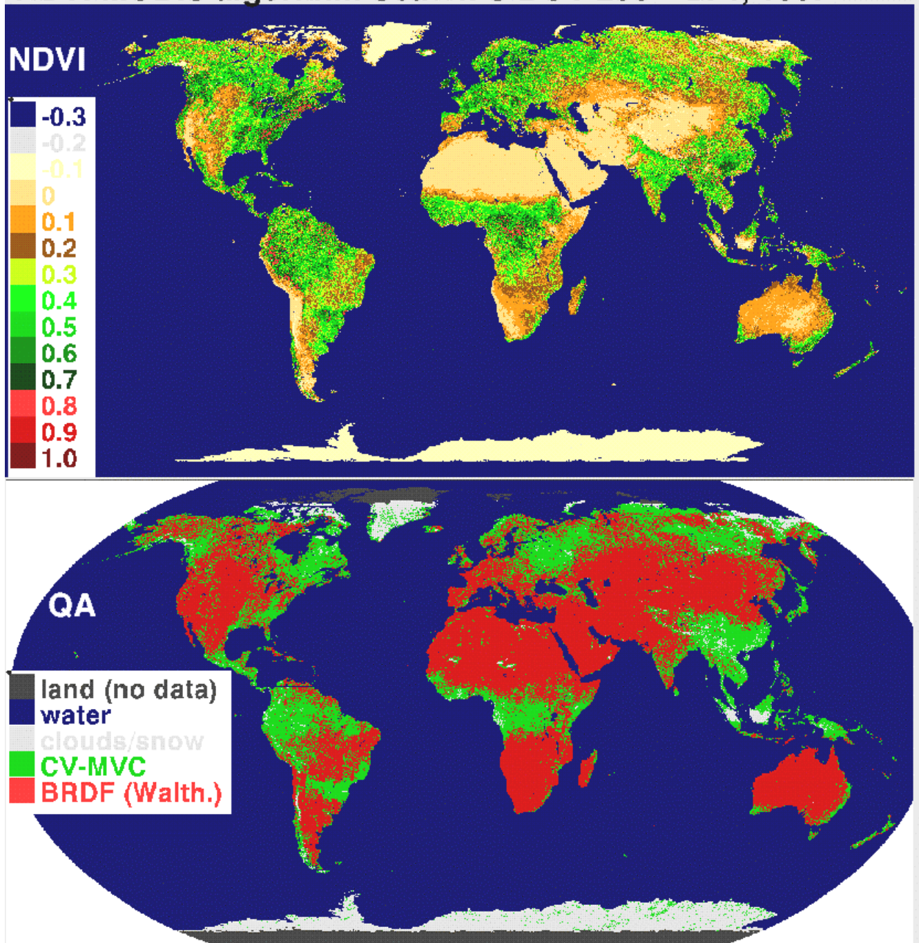
Figure 3.2.14: Global EVI (a) and NDVI (b) image (pseudo color) using the MODIS VI composite algorithm (BRDF/ CV-MVC/ MVC approach). (c) Color coded quality assurance flags for a Global NDVI composite (very similar for EVI) using the MODIS approach (BRDF/CV-MVC/MVC)
