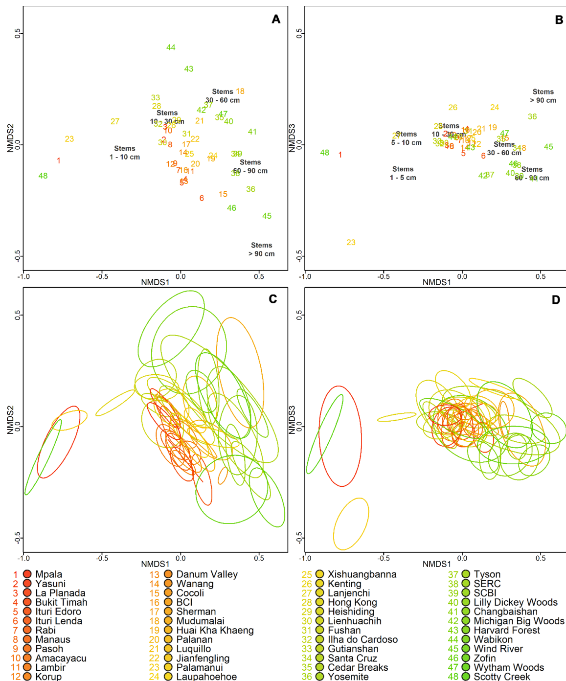
Fig. 4. Three-dimensional nonmetric multidimensional scaling (NMDS) results for density of trees organized into six diameter classes in 1260, 100 m × 100 m hectares of 48 forest plots in the ForestGEO network (A, B). The structural classes (diameter bins) used in the NMDS ordination are superimposed in black text (A, B). The within plot variation of structure for each plot is shown by depiction of the standard deviation ellipses of the individual 100 m × 100 m hectares within each plot (C, D; where C reflects the variation of NMDS1 vs. NMDS2 (A) and D reflects the variation of NMDS1 vs. NMDS3 (B). Ordination stress = 0.047. Colours indicate
