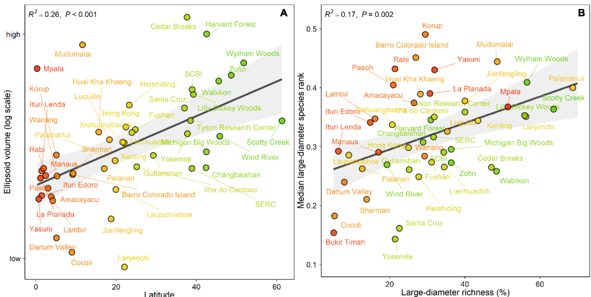
Fig. 5. The 1-ha scale structural complexity of 48 forest plots in the ForestGEO network as a function of absolute latitude (A). The metric of structural complexity is the volume of the three-dimensional ellipsoid generated from the NMDS ordination of abundance in structural classes (see Fig. 4 for two dimensional projections and the Supplementary Material S2 for a three-dimensional animation). The rank order of large-diameter species in 48 forest plots (B). Rank order is normalized to the range from zero to one to compare plots with differing species richness. Lower proportions of large-diameter species rank correspond to more abundant species (median large-diameter species rank < 0.5 for all 48 forest plots). Species attaining large-diameters were the more common species in the forest plots. Colours indicate increasing absolute latitude from red to green.
