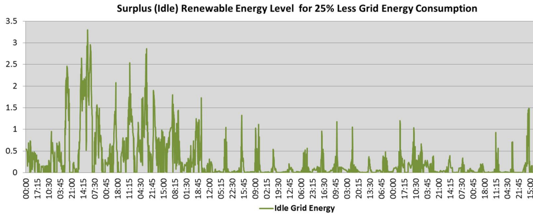
Figure 18. The surplus renewable energy amount after the optimised schedule for 25% less grid energy consumption level for one month (weekly0).
