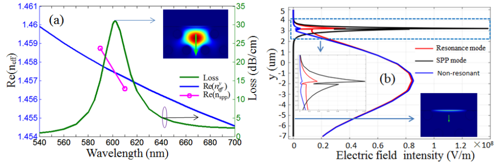
Fig. 2. (a). Real part of effective refractive index of the y-polarized fiber core mode and SPP mode, and the loss spectra of the D-shaped PCF SPR sensor with \Lambda = 7.8 \mu\text{m} , d = 3.6 \mu\text{m} , h = 0.4\Lambda , and n_a = 1.33 . (b) Electric field distributions of the y-polarized core modes at \lambda = 520 \text{ nm} , \lambda = 602 \text{ nm} (phase matching point), and the SPP mode at \lambda = 540 \text{ nm} along the y axis.
