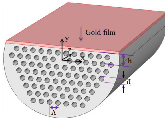
Fig. 1. Schematic diagram of the SPR sensor based on D-shaped photonic crystal fiber in 3D model. The PCF polished surface is perpendicular to the y axis.
