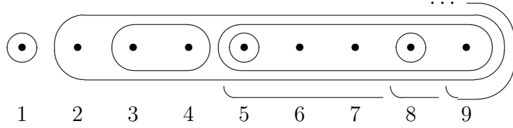
Figure 4: Example. Possible choices for MN(9) if MN(2) and MN(6) are expanded to include 9.
