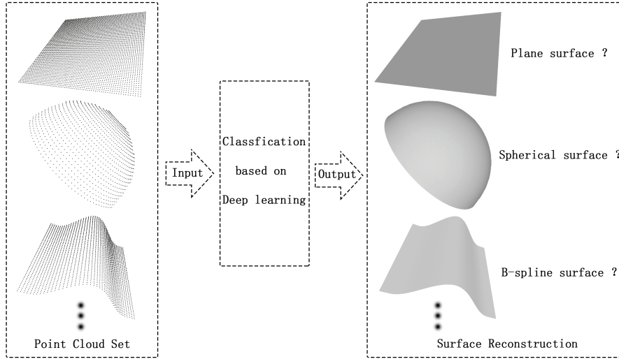
Figure 2: Classification model.
