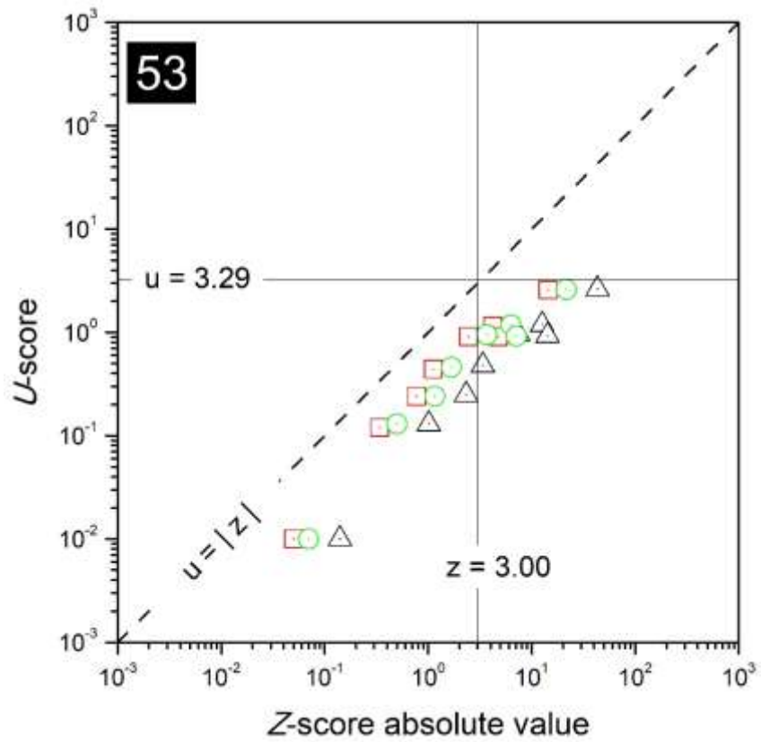
FIG. 57. Combined plots of z- and u-scores for the laboratory with code 53.
