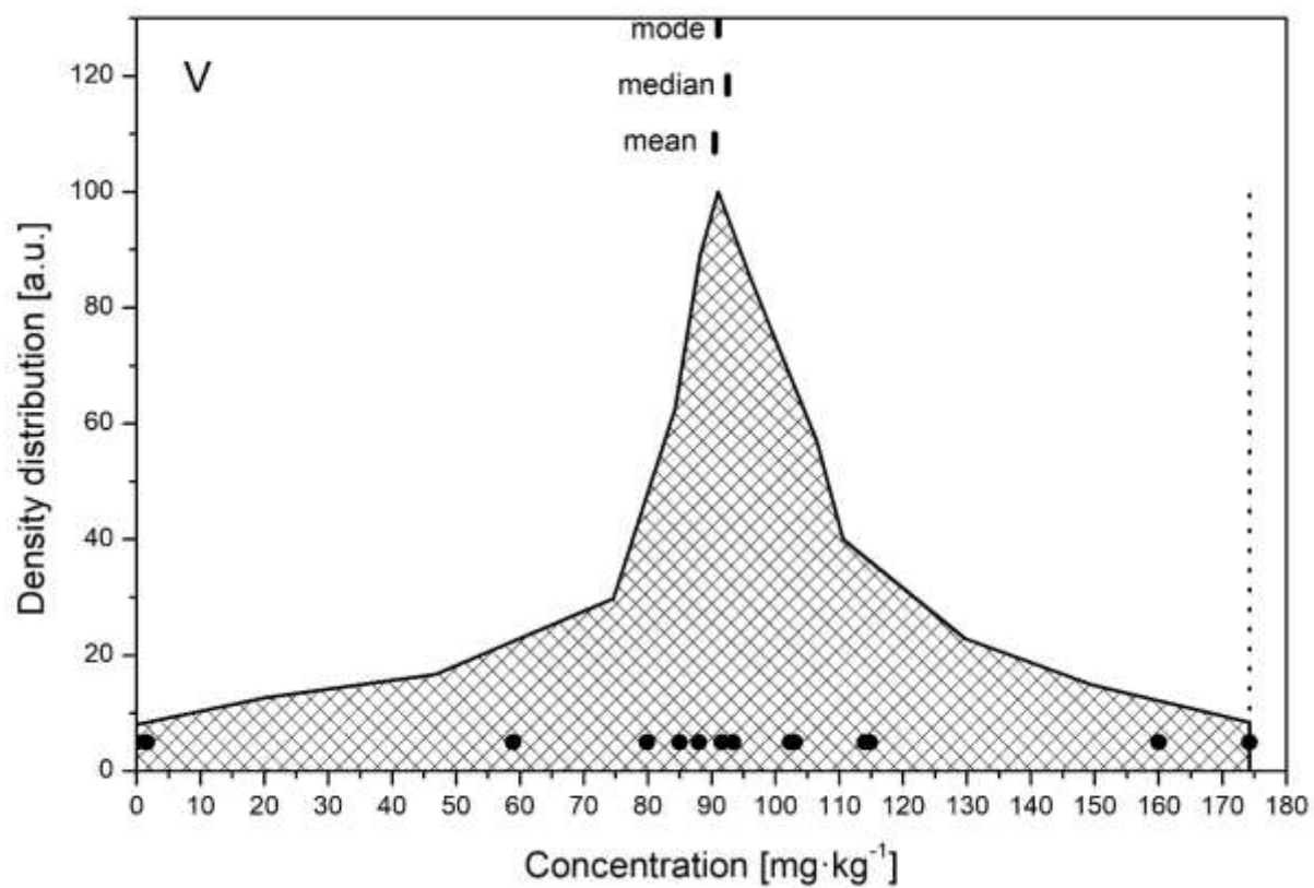
FIG. 26. The density distribution function for the analyte V.
