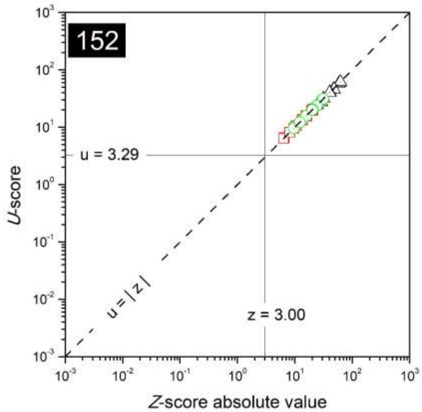
FIG. 87. Combined plots of z- and u-scores for the laboratory with code 152.
