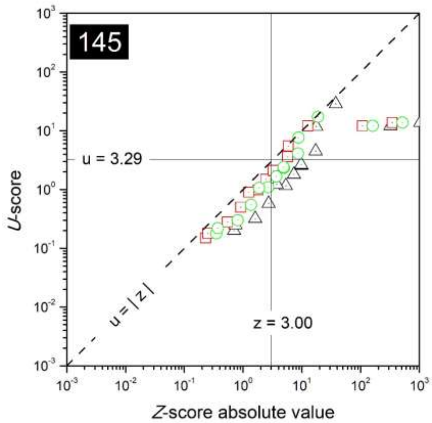
FIG. 82. Combined plots of z- and u-scores for the laboratory with code 145.
