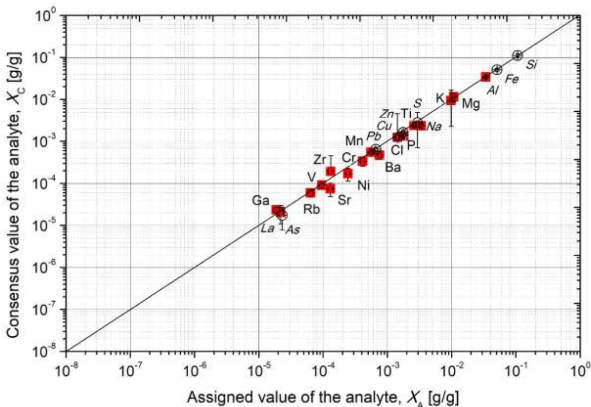
FIG. 2. Correlation between assigned, X_A , and consensus values of analytes, X_C 1 .
