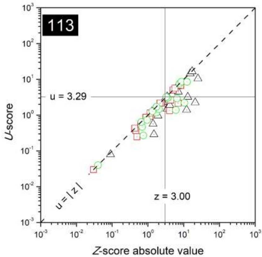
FIG. 73. Combined plots of z- and u-scores for the laboratory with code 113.
