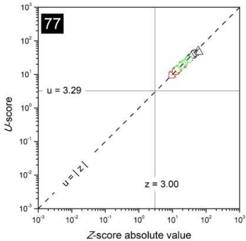
FIG. 63. Combined plots of z- and u-scores for the laboratory with code 77.
