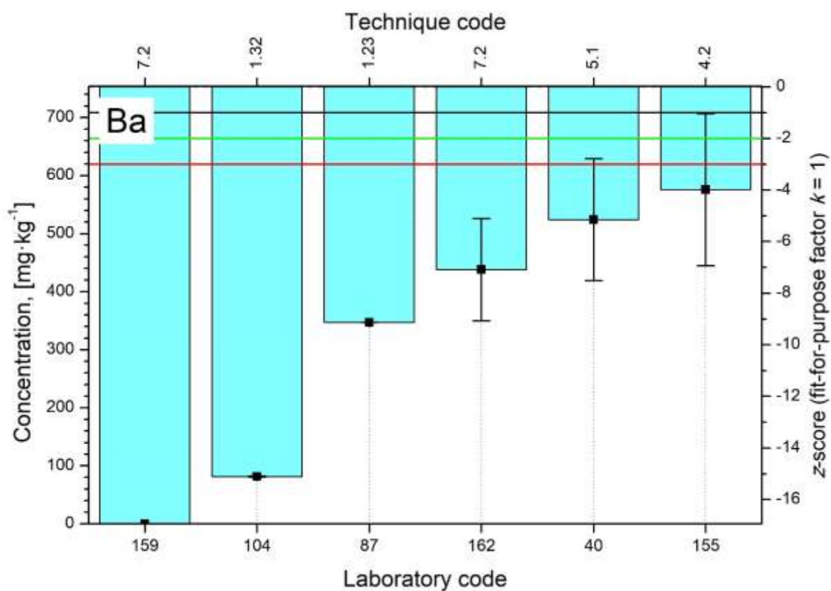
FIG. 31. Distributions of z-scores for analyte Ba.
