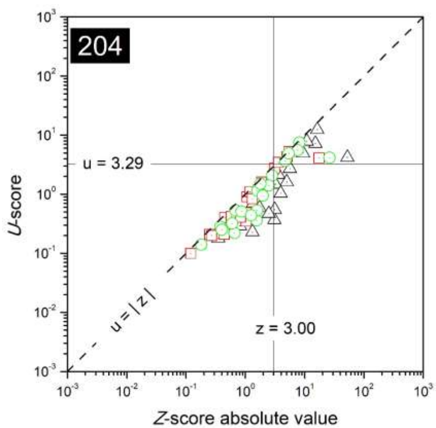
FIG. 94. Combined plots of z - and u -scores for the laboratory with code 204.
