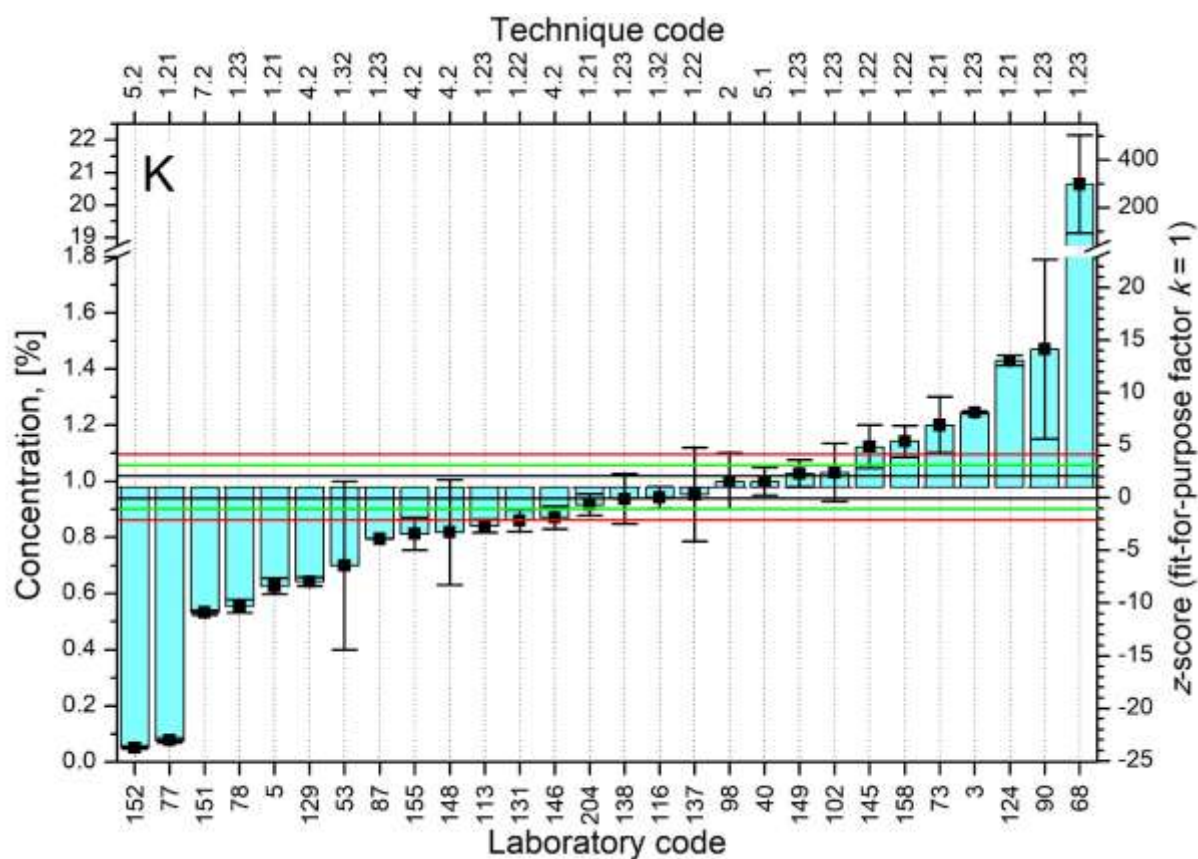
FIG. 36. Distributions of z-scores for analyte K.
