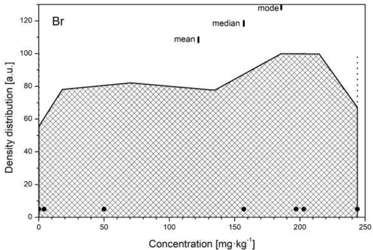
FIG. 5. The density distribution function for the analyte Br.
