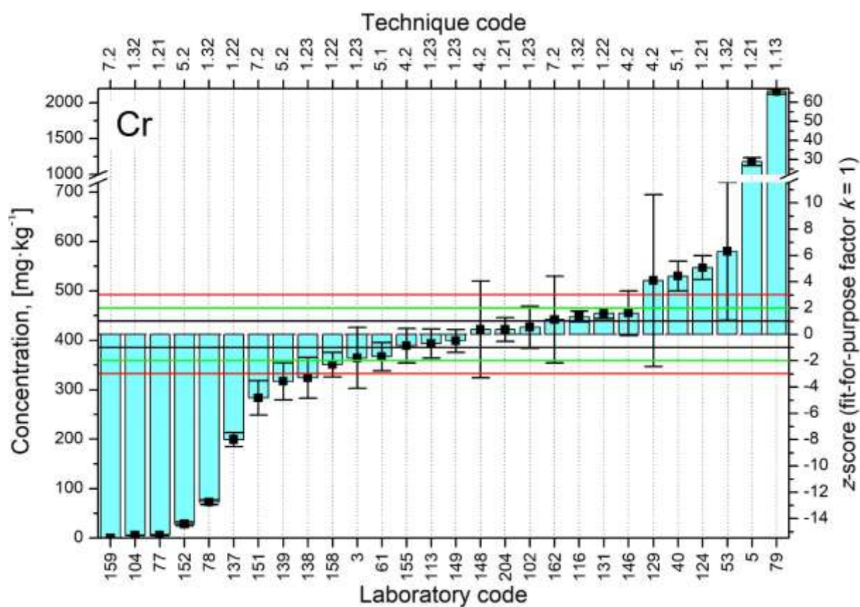
FIG. 33. Distributions of z-scores for analyte Cr.
