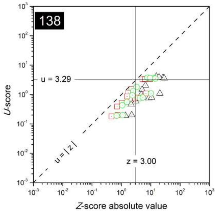
FIG. 79. Combined plots of z- and u-scores for the laboratory with code 138.
