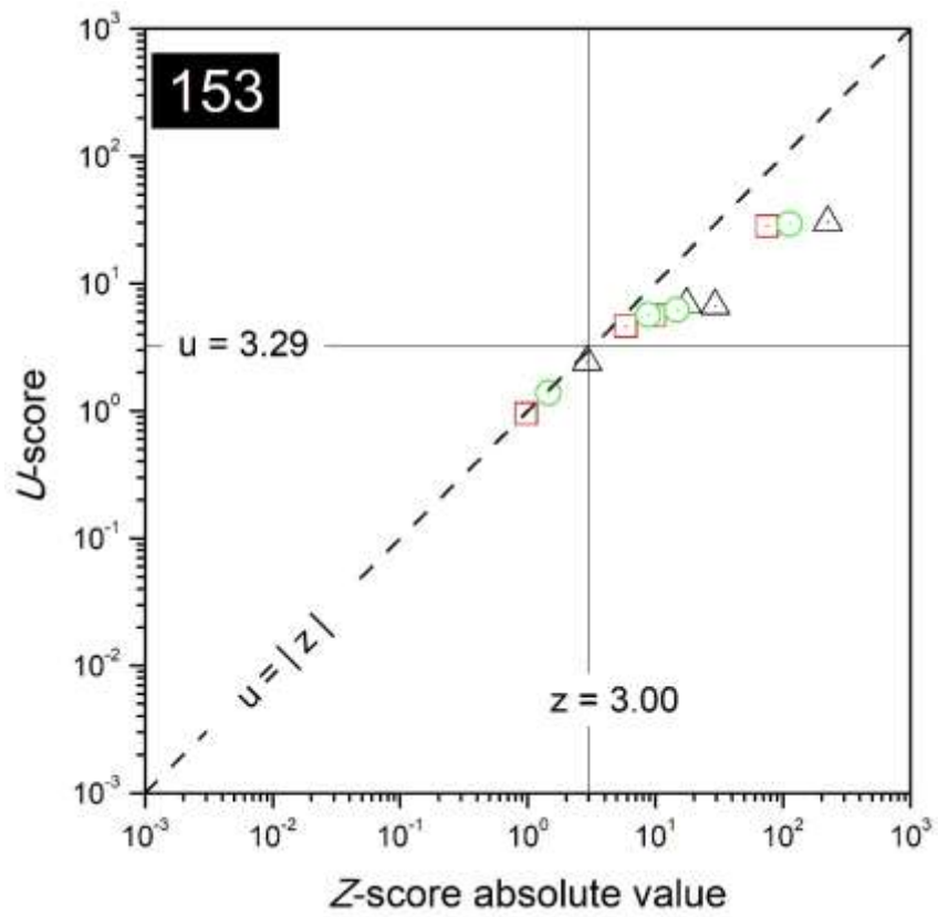
FIG. 88. Combined plots of z- and u-scores for the laboratory with code 153.
