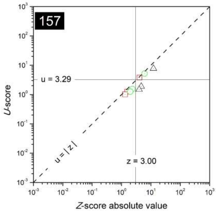
FIG. 90. Combined plots of z - and u -scores for the laboratory with code 157.
