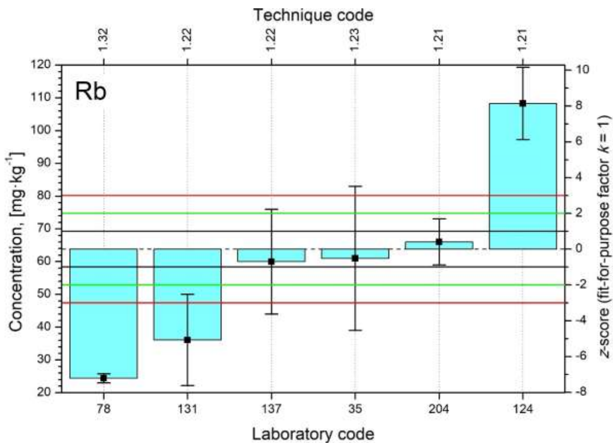
FIG. 44. Distributions of z-scores for analyte Rb.
