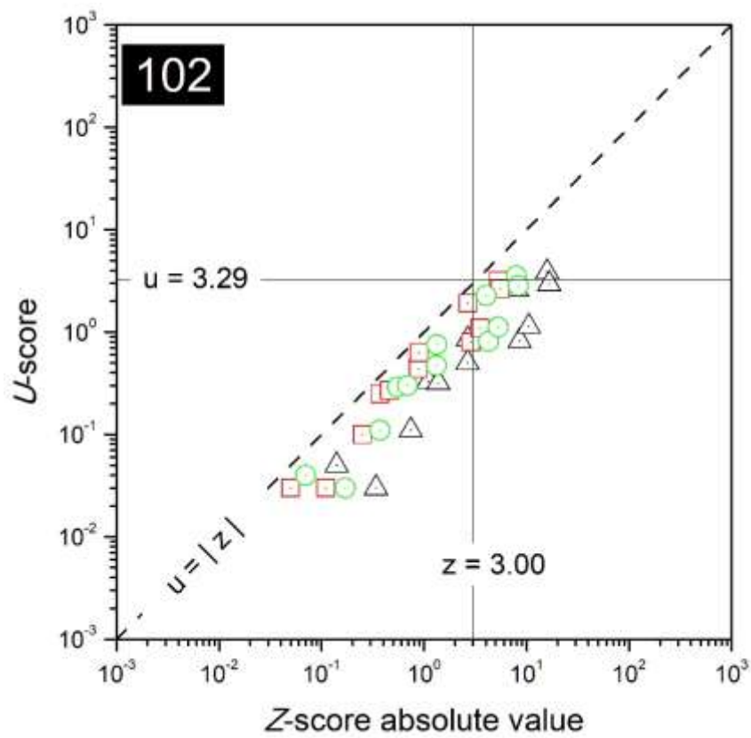
FIG. 71. Combined plots of z- and u-scores for the laboratory with code 102.
