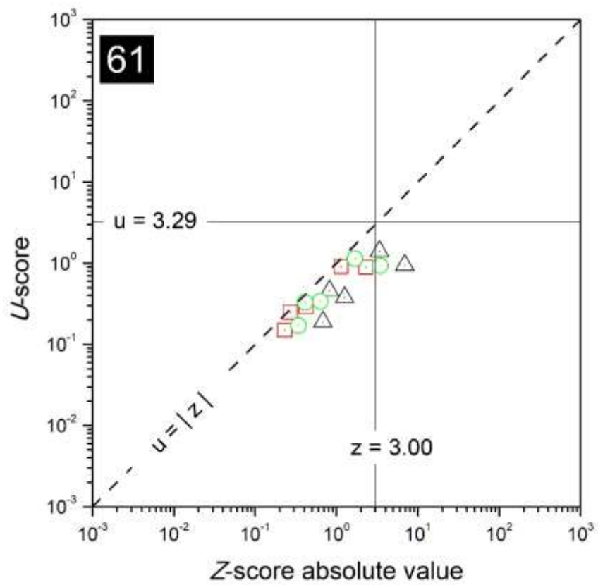
FIG. 59. Combined plots of z- and u-scores for the laboratory with code 61.
