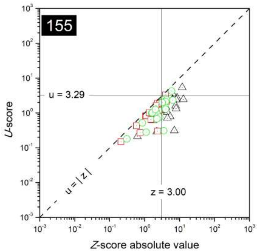
FIG. 89. Combined plots of z- and u-scores for the laboratory with code 155.
