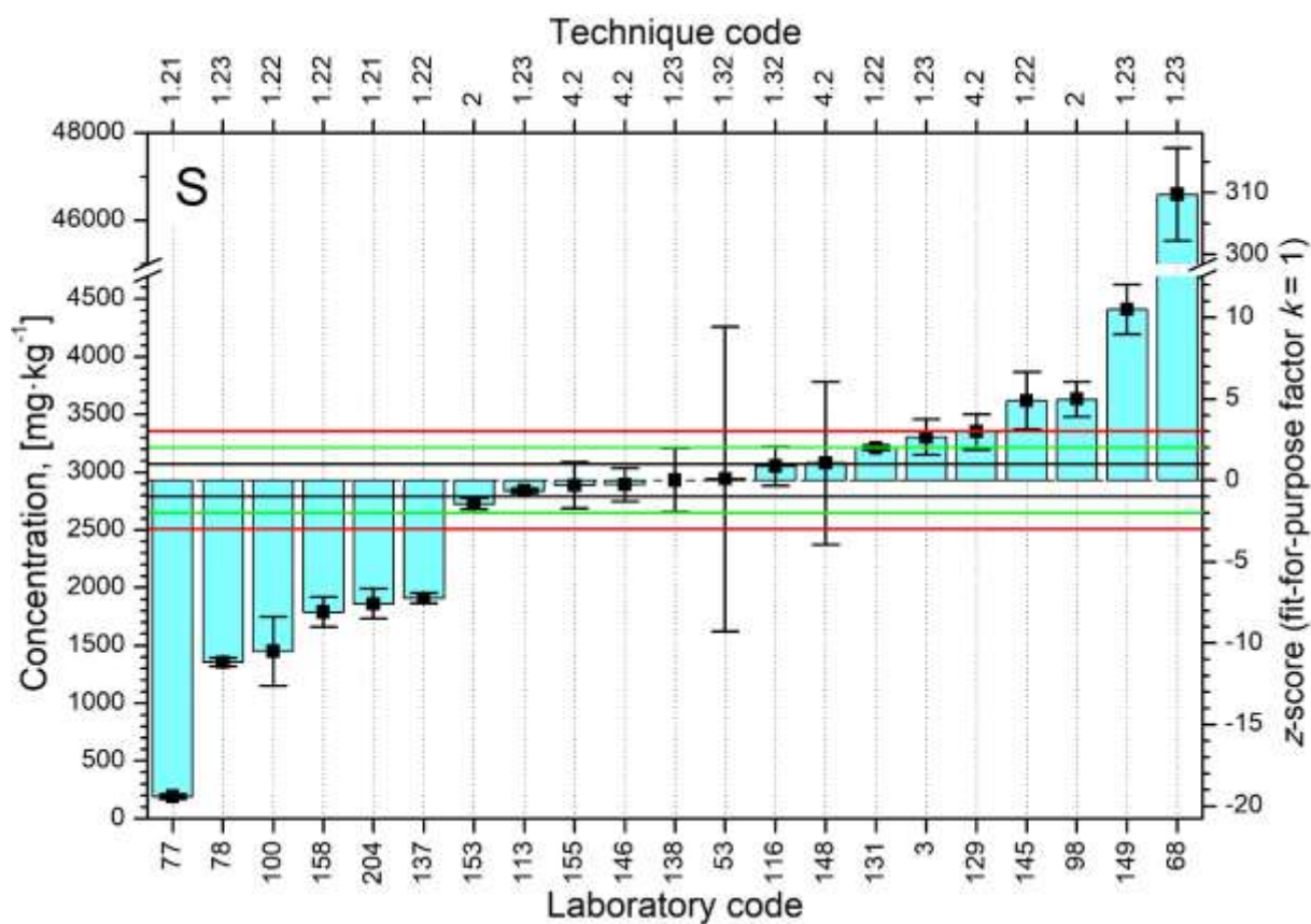
FIG. 45. Distributions of z-scores for analyte S.
