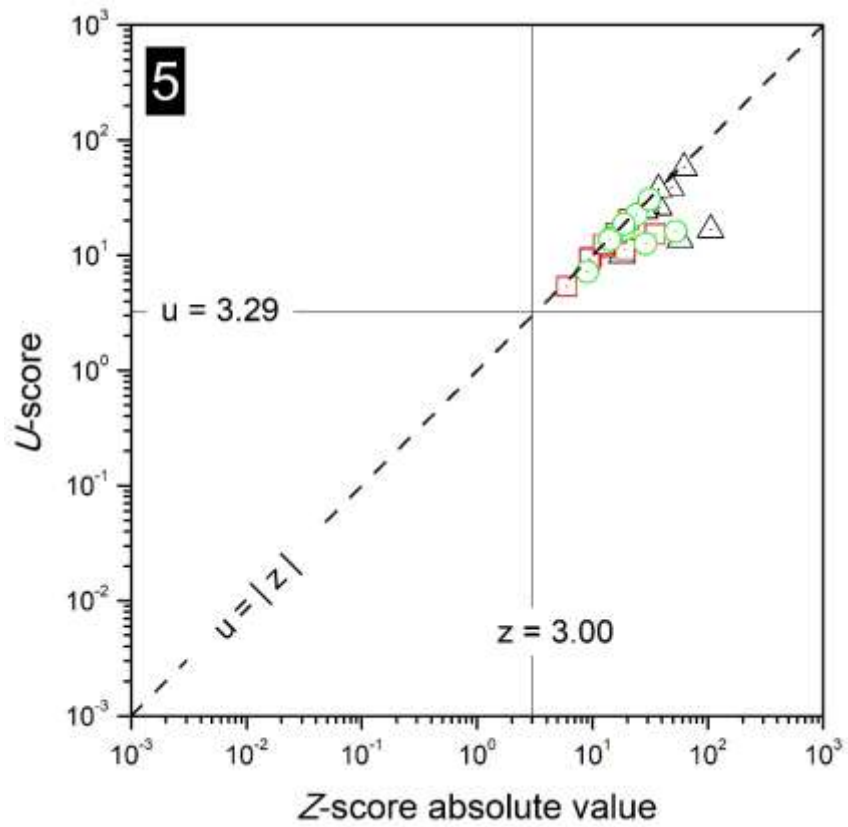
FIG. 53. Combined plots of z- and u-scores for the laboratory with code 5.
