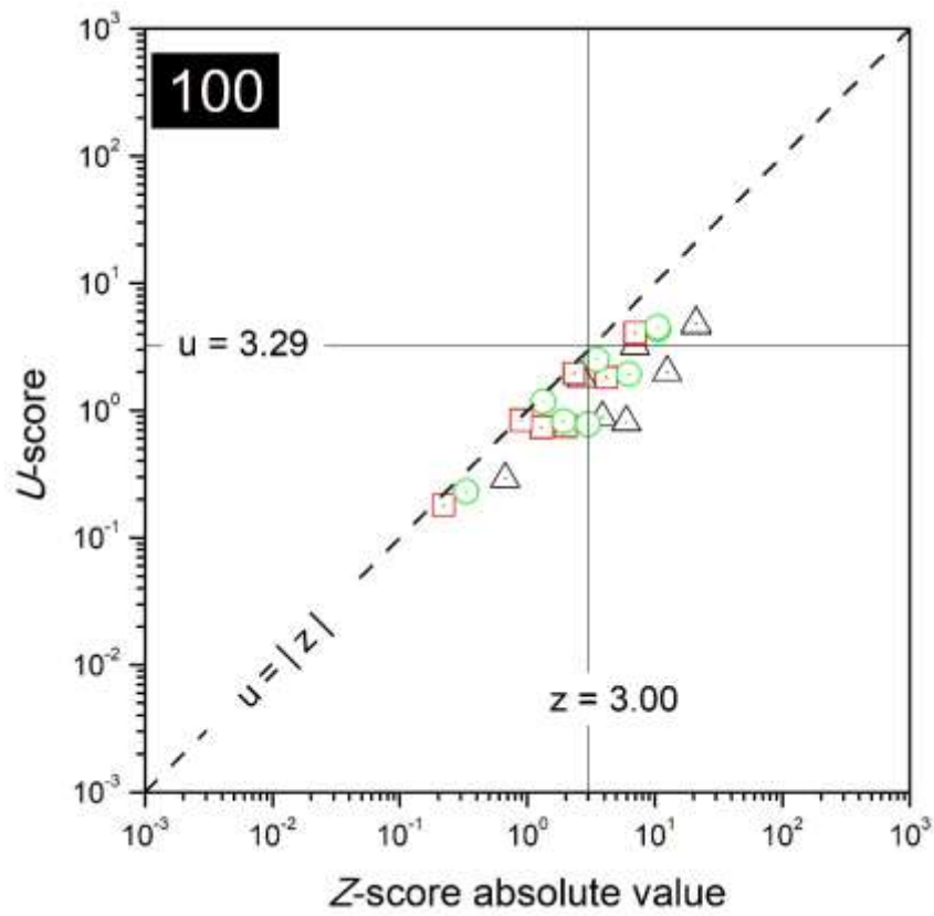
FIG. 70. Combined plots of z- and u-scores for the laboratory with code 100.
