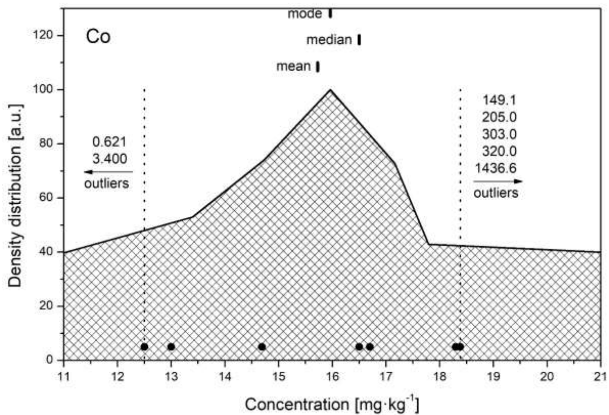
FIG. 8. The density distribution function for the analyte Co.
