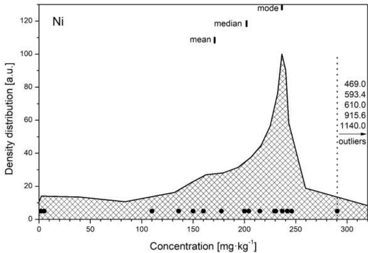
FIG. 17. The density distribution function for the analyte Ni.
