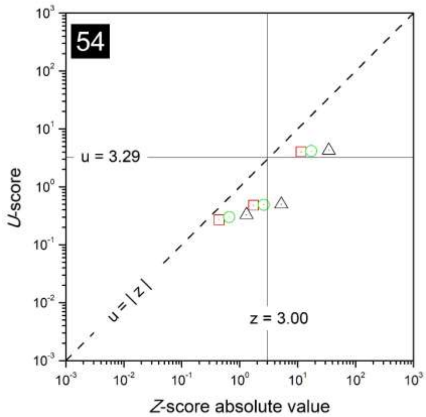
FIG. 58. Combined plots of z- and u-scores for the laboratory with code 54.
