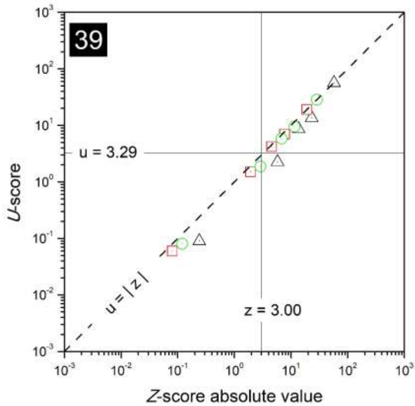
FIG. 55. Combined plots of z- and u-scores for the laboratory with code 39.
