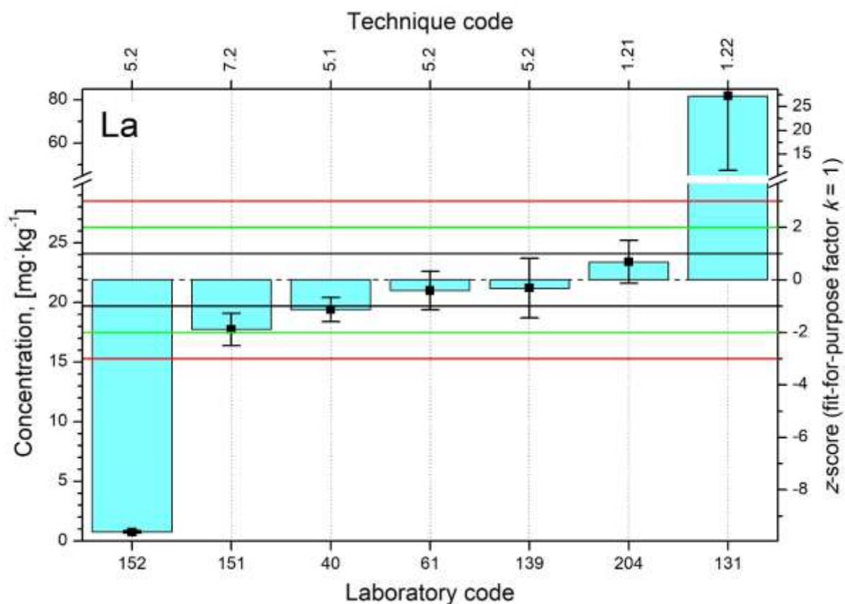
FIG. 37. Distributions of z-scores for analyte La.
