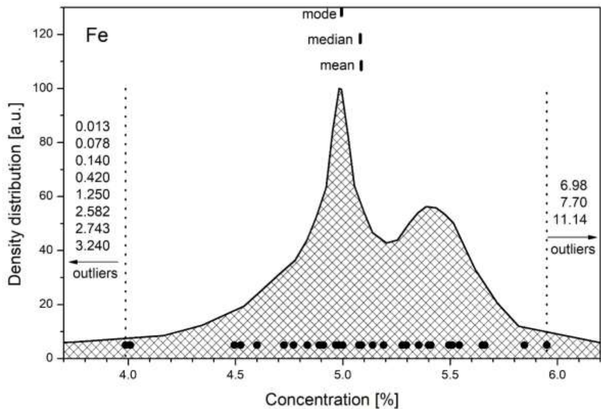
FIG. 11. The density distribution function for the analyte Fe.
