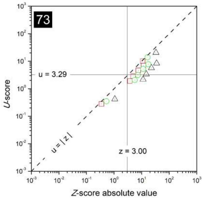
FIG. 62. Combined plots of z- and u-scores for the laboratory with code 73.
