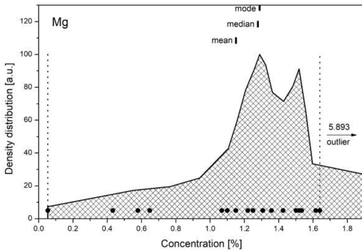
FIG. 14. The density distribution function for the analyte Mg.
