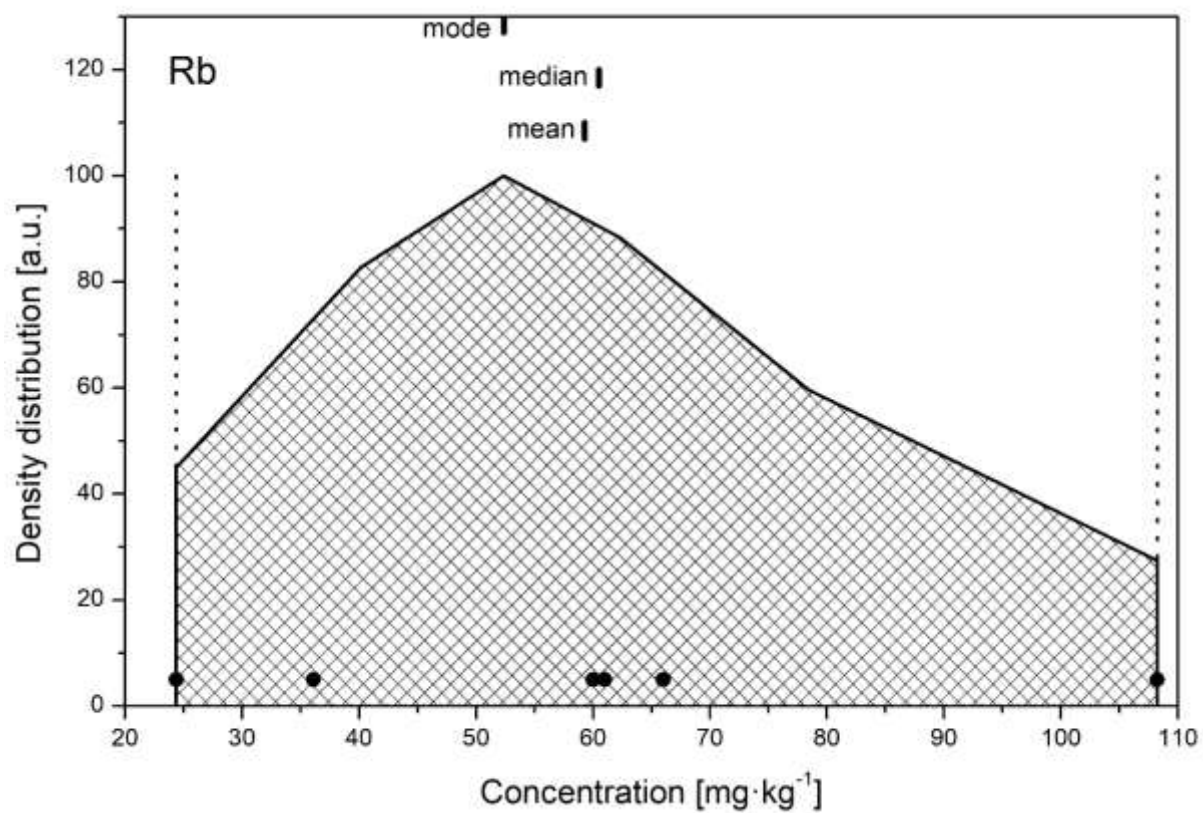
FIG. 20. The density distribution function for the analyte Rb.
