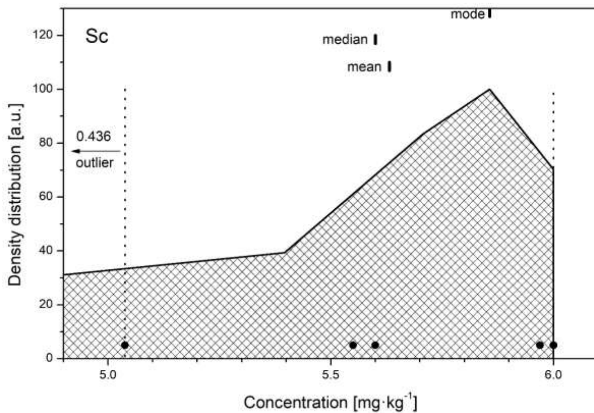
FIG. 22. The density distribution function for the analyte Sc.
