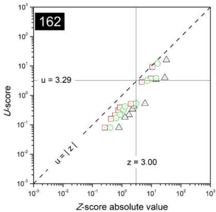
FIG. 93. Combined plots of z - and u -scores for the laboratory with code 162.
