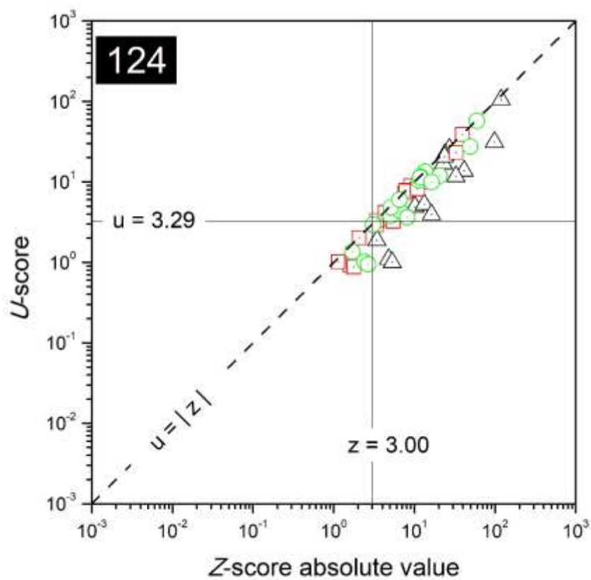
FIG. 75. Combined plots of z - and u -scores for the laboratory with code 124.
