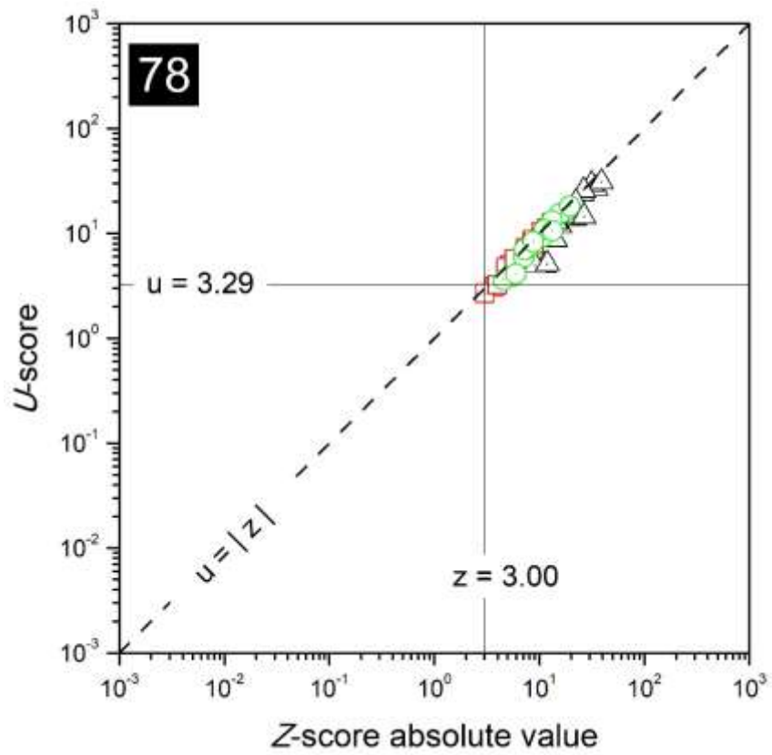
FIG. 64. Combined plots of z - and u -scores for the laboratory with code 78.
