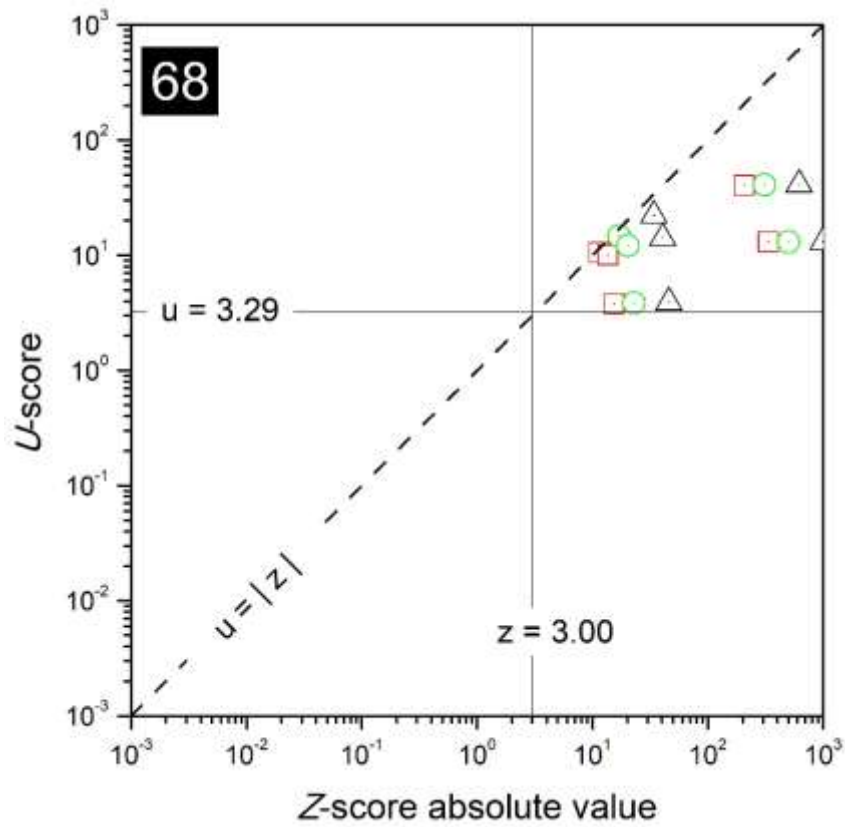
FIG. 61. Combined plots of z- and u-scores for the laboratory with code 68.
