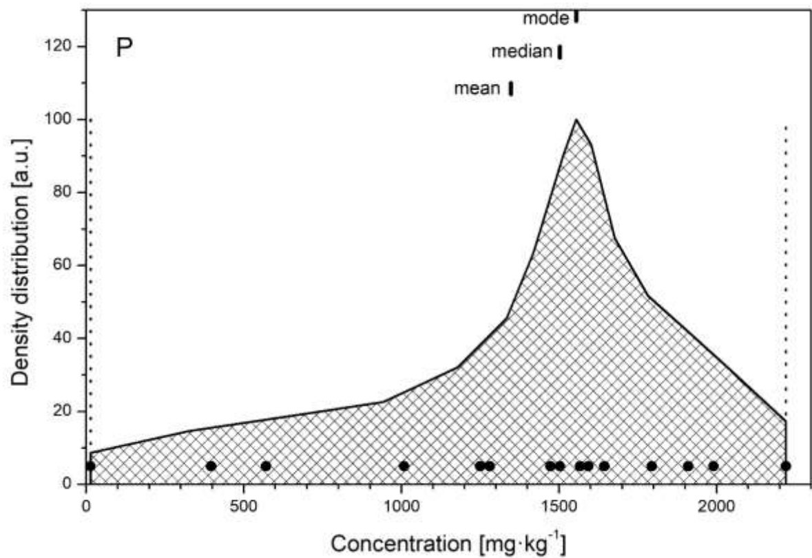
FIG. 18. The density distribution function for the analyte P.
