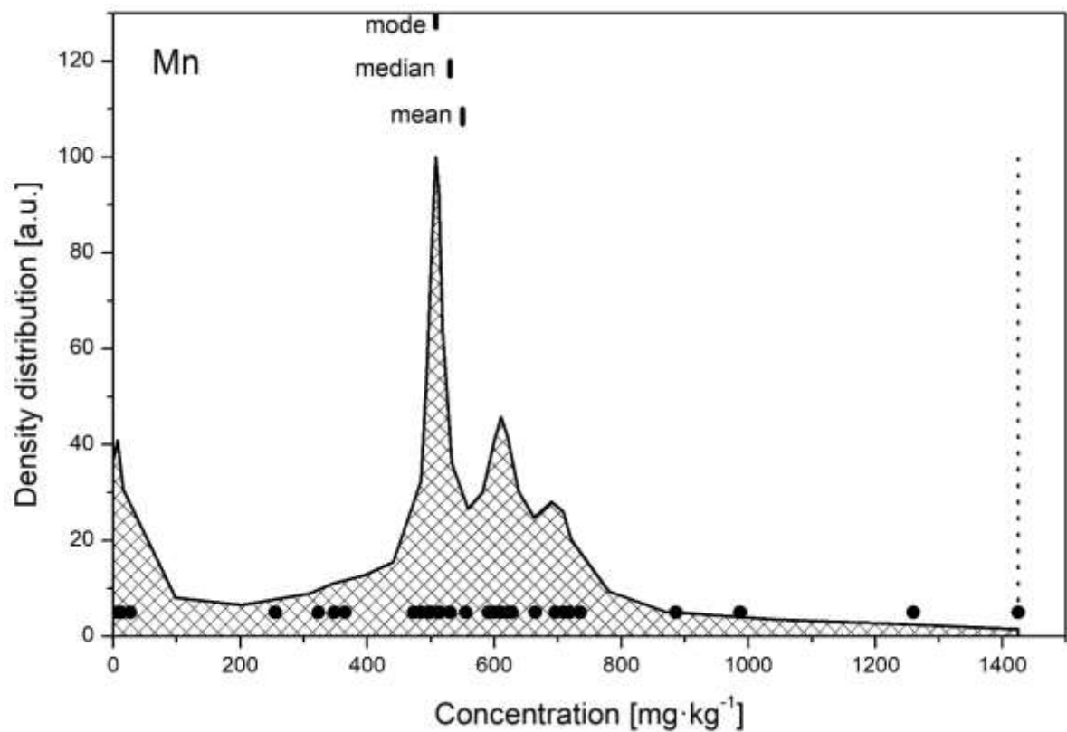
FIG. 15. The density distribution function for the analyte Mn.
