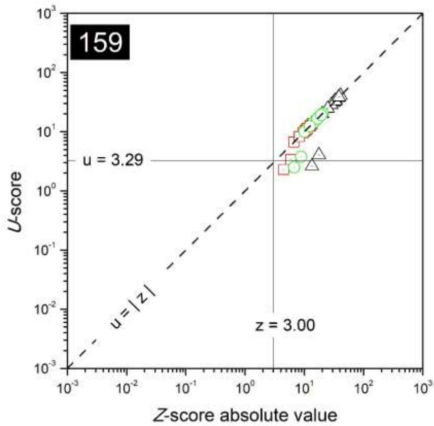
FIG. 92. Combined plots of z - and u -scores for the laboratory with code 159.
