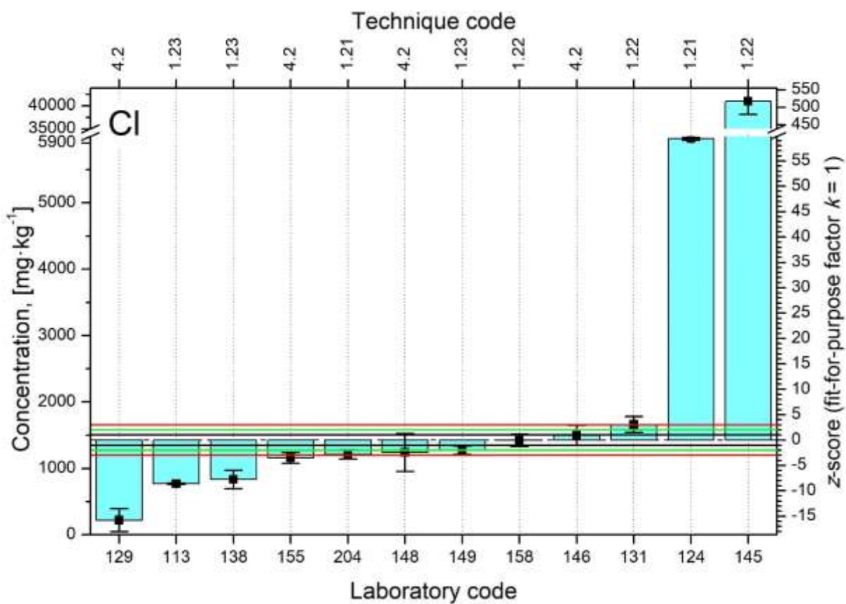
FIG. 32. Distributions of z-scores for analyte Cl.
