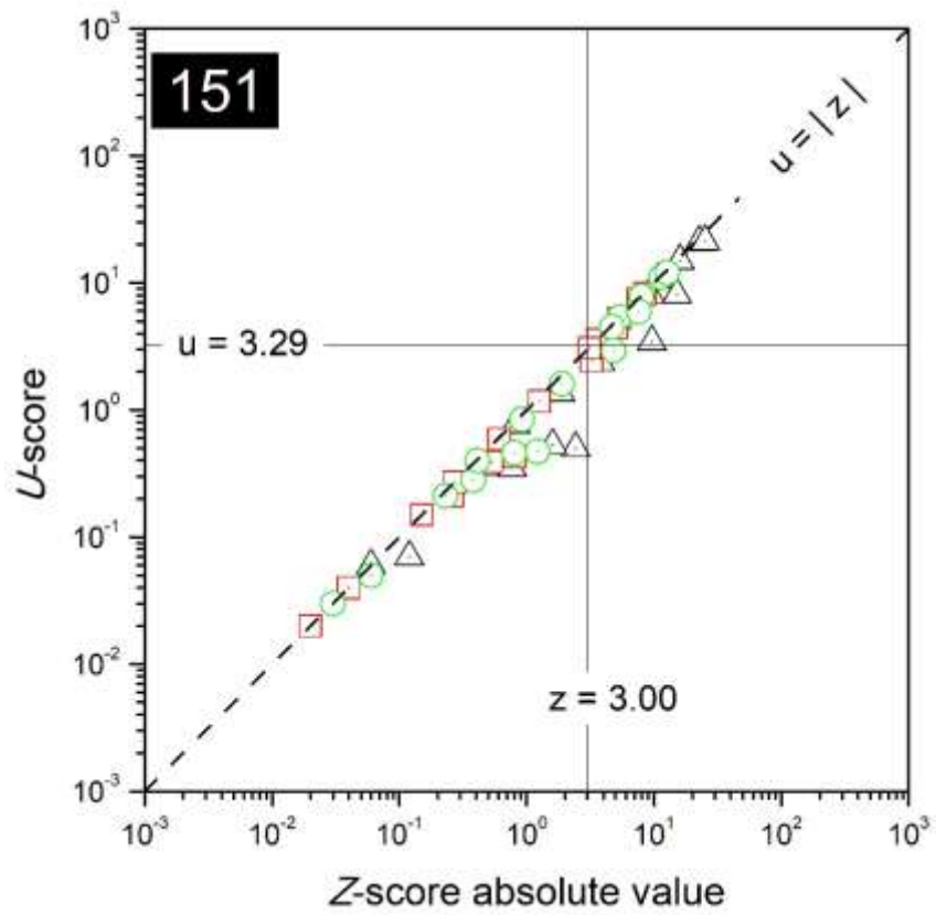
FIG. 86. Combined plots of z- and u-scores for the laboratory with code 151.
