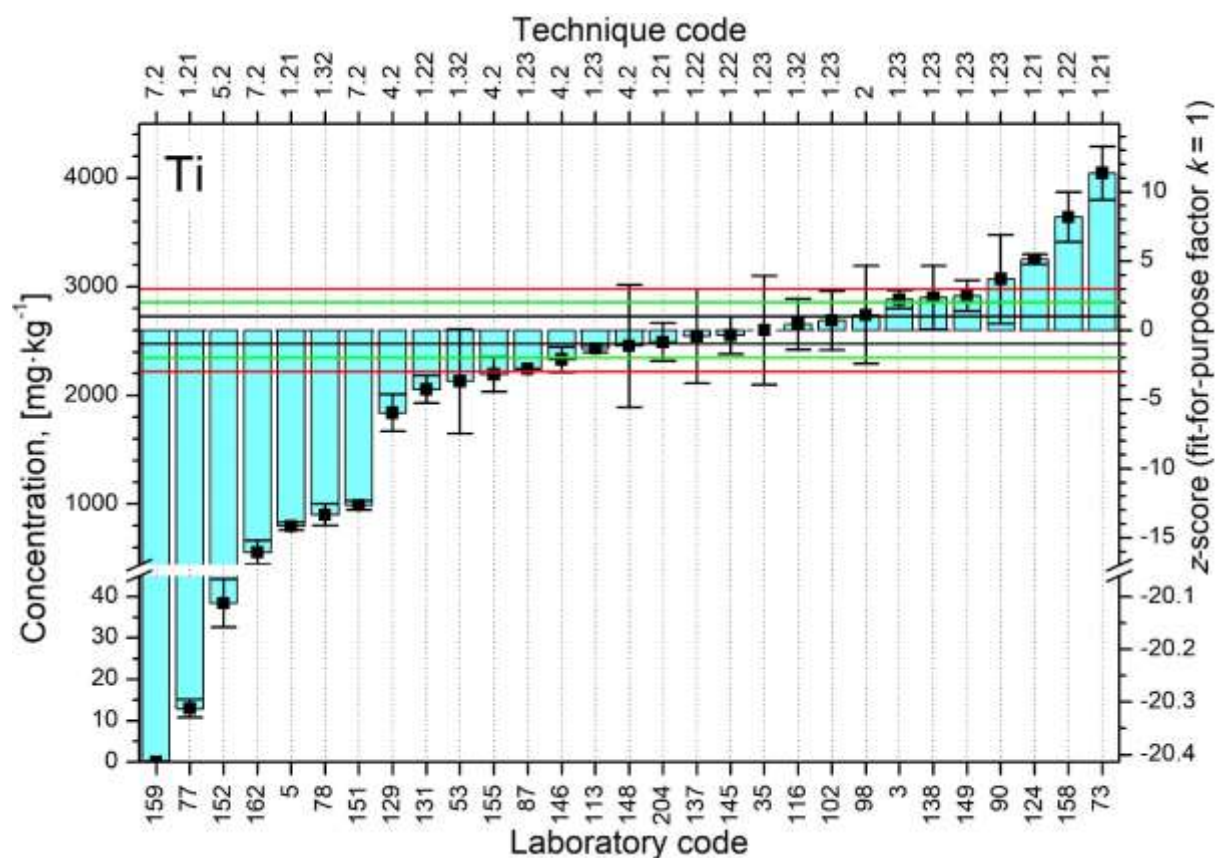
FIG. 48. Distributions of z-scores for analyte Ti.
