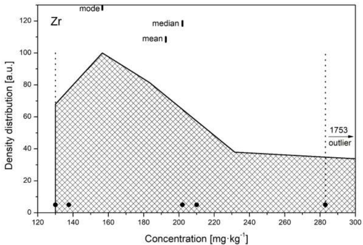
FIG. 28. The density distribution function for the analyte Zr.
