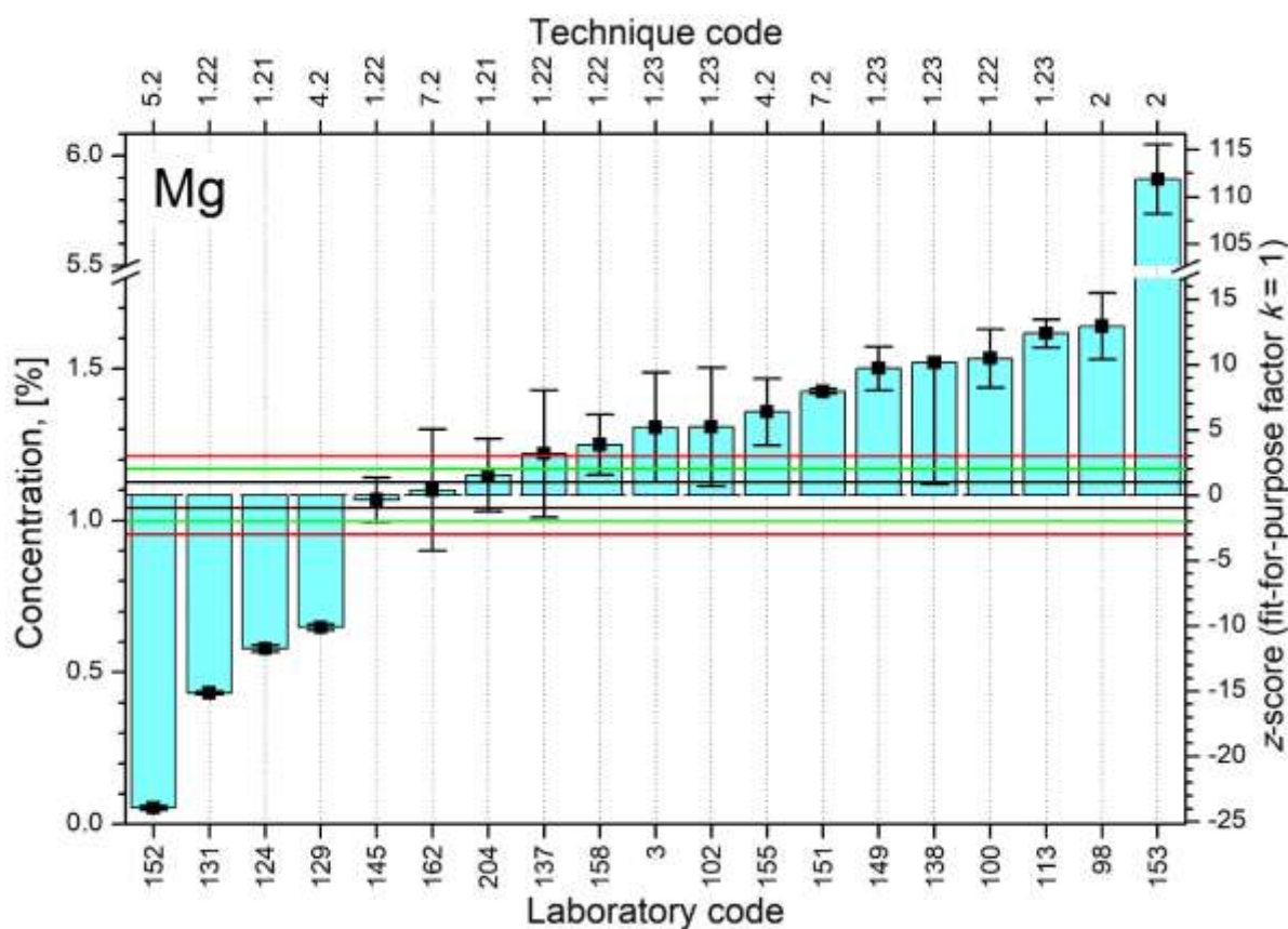
FIG. 38. Distributions of z-scores for analyte Mg.
