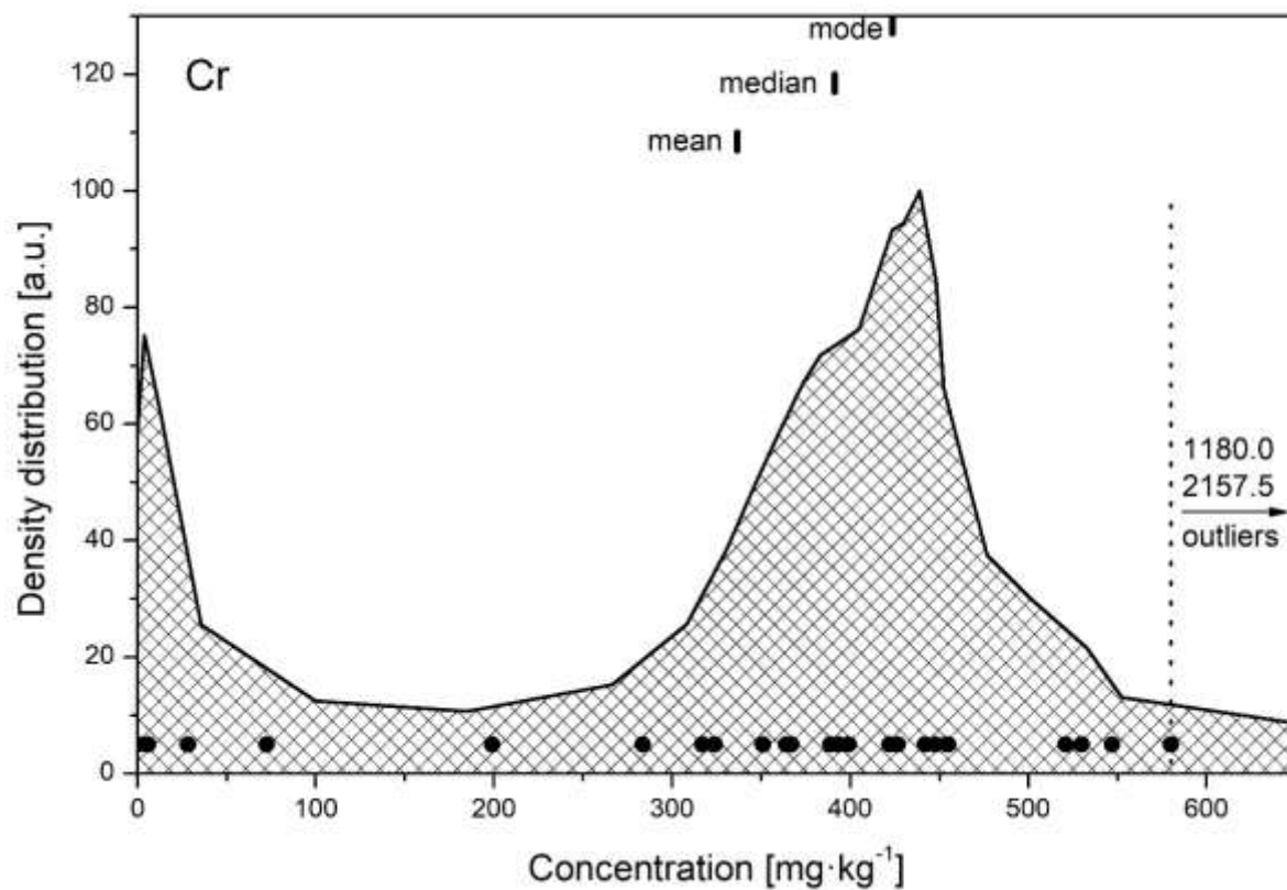
FIG. 9. The density distribution function for the analyte Cr.
