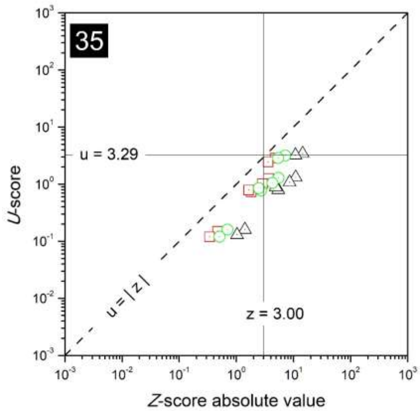
FIG. 54. Combined plots of z- and u-scores for the laboratory with code 35.
