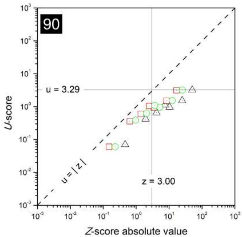
FIG. 67. Combined plots of z- and u-scores for the laboratory with code 90.
