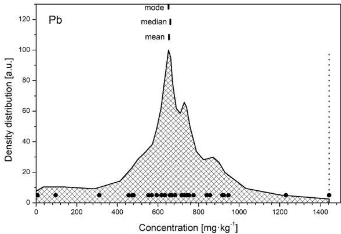
FIG. 19. The density distribution function for the analyte Pb.
