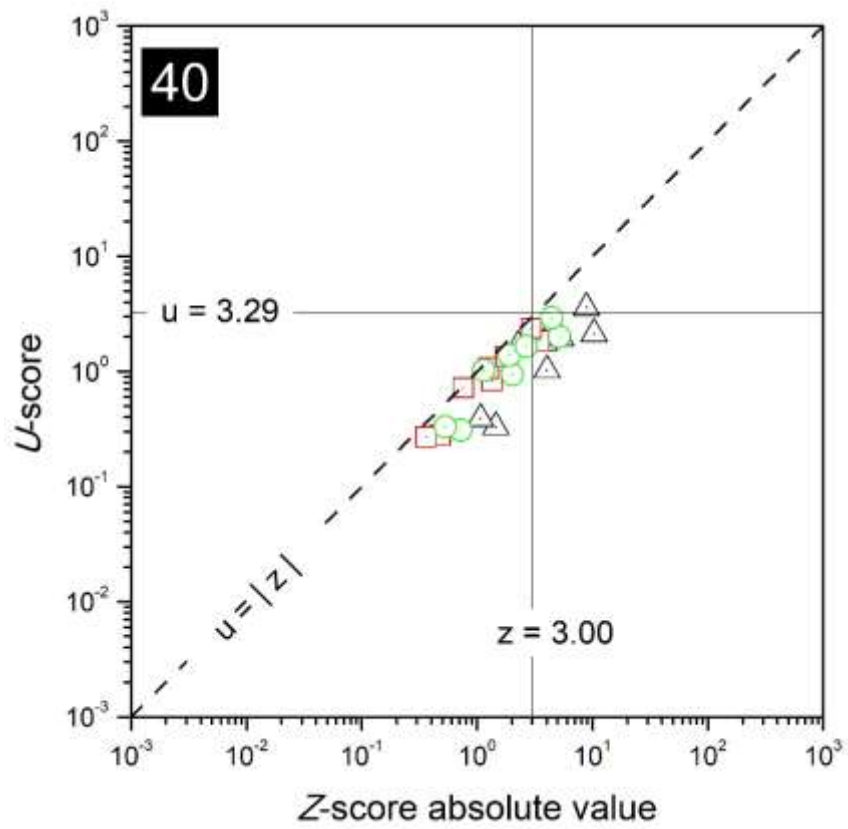
FIG. 56. Combined plots of z- and u-scores for the laboratory with code 40.
