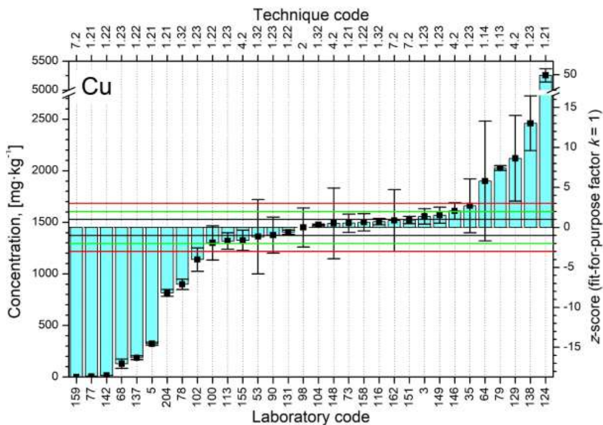
FIG. 34. Distributions of z-scores for analyte Cu.
