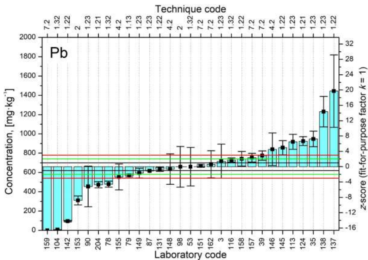
FIG. 43. Distributions of z-scores for analyte Pb.
