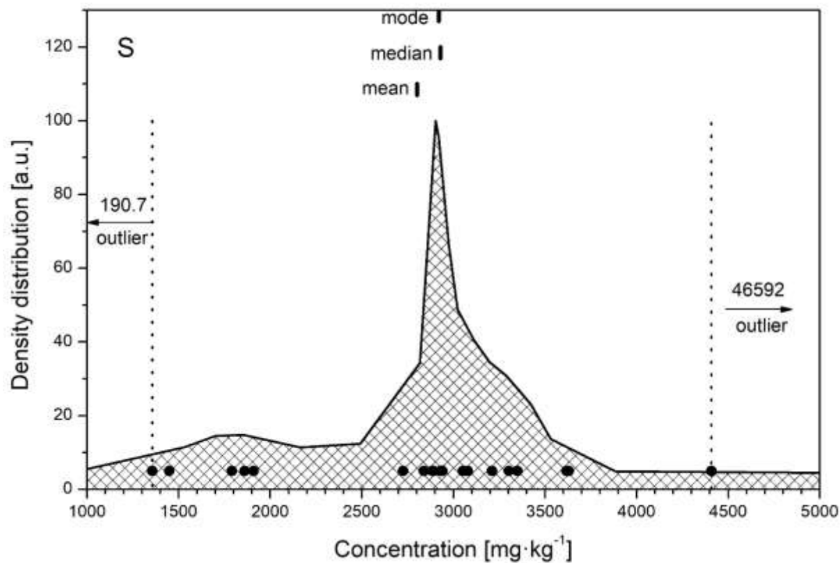
FIG. 21. The density distribution function for the analyte S.
