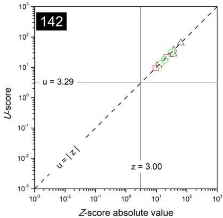
FIG. 81. Combined plots of z- and u-scores for the laboratory with code 142.
