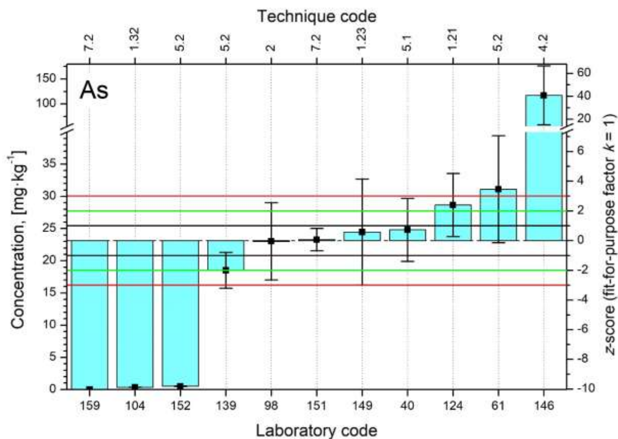
FIG. 30. Distributions of z-scores for analyte As.
