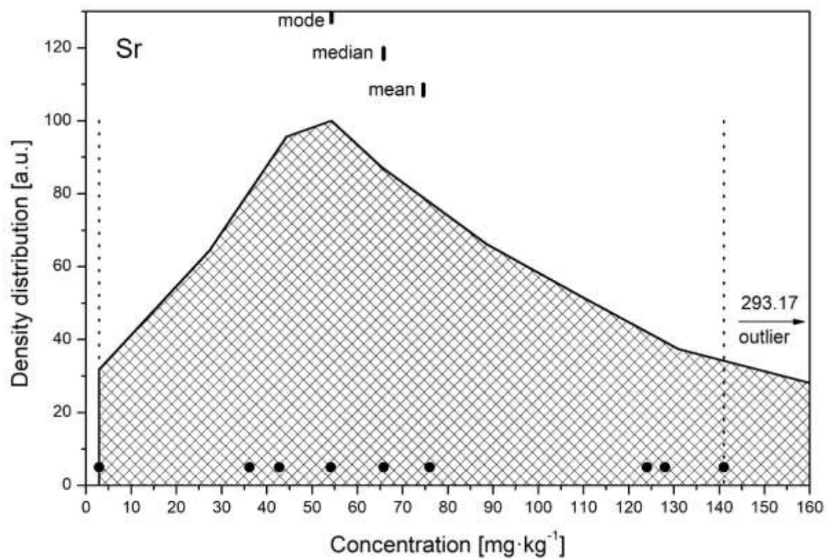
FIG. 24. The density distribution function for the analyte Sr.
