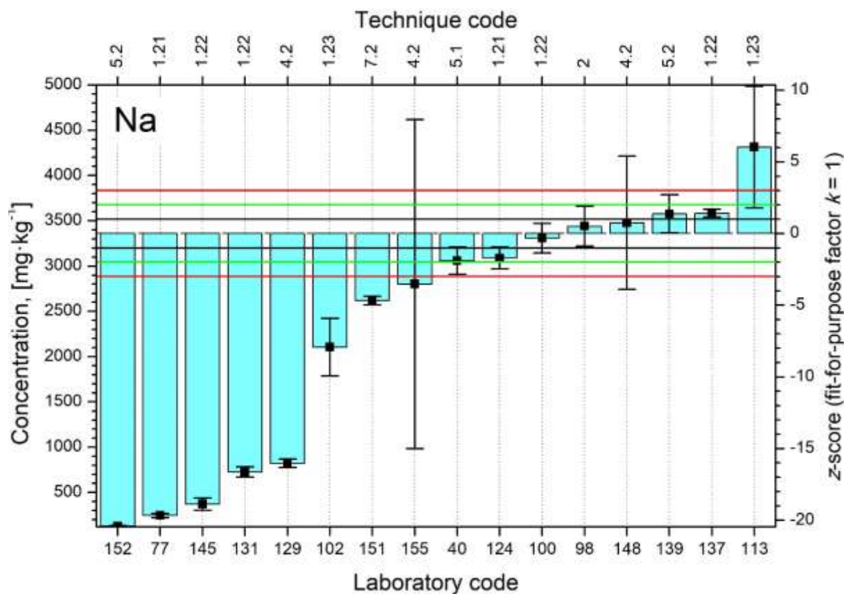
FIG. 40. Distributions of z-scores for analyte Na.
