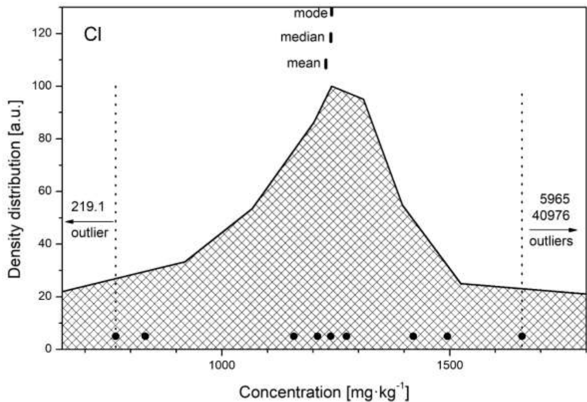
FIG. 7. The density distribution function for the analyte Cl.
