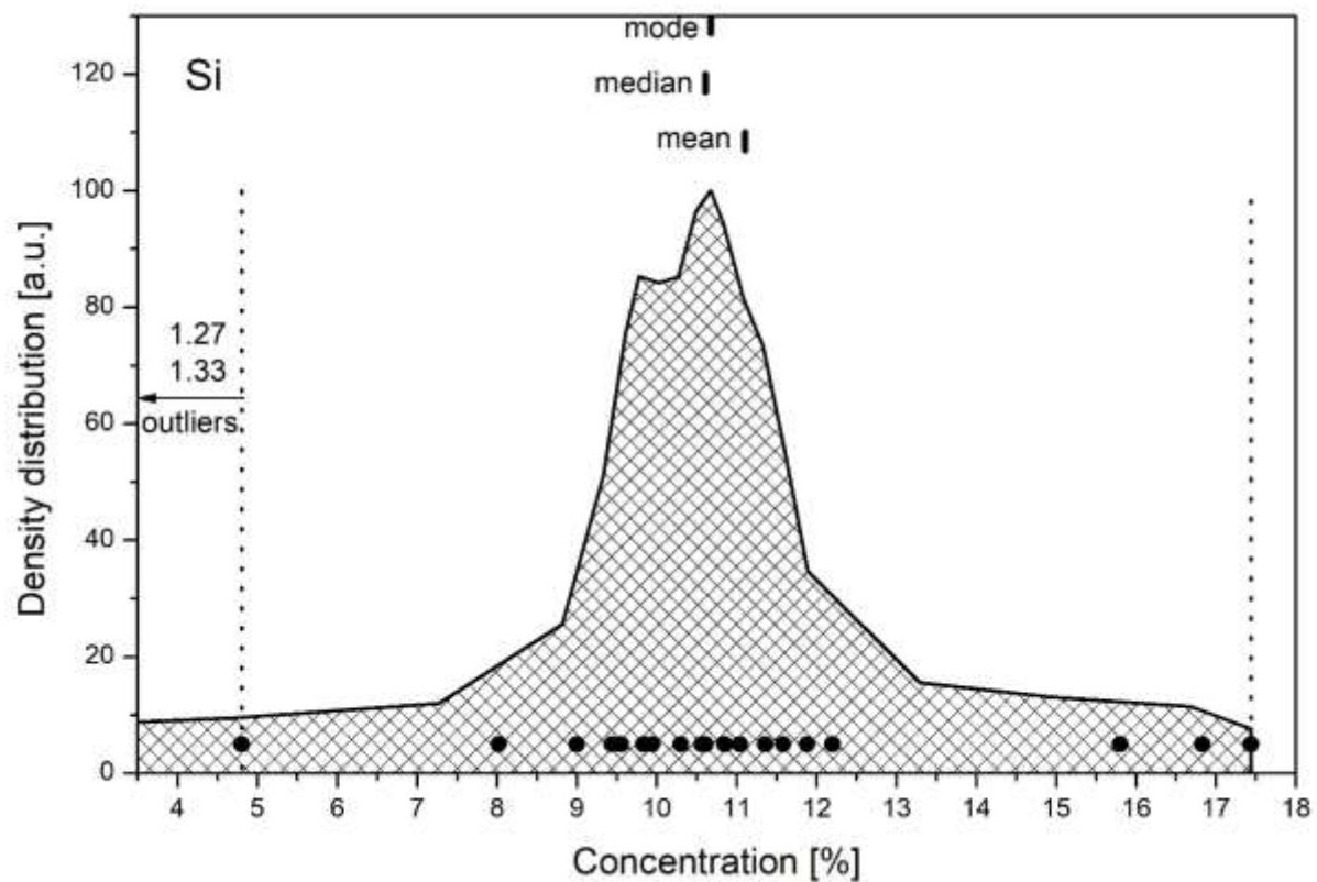
FIG. 23. The density distribution function for the analyte Si.
