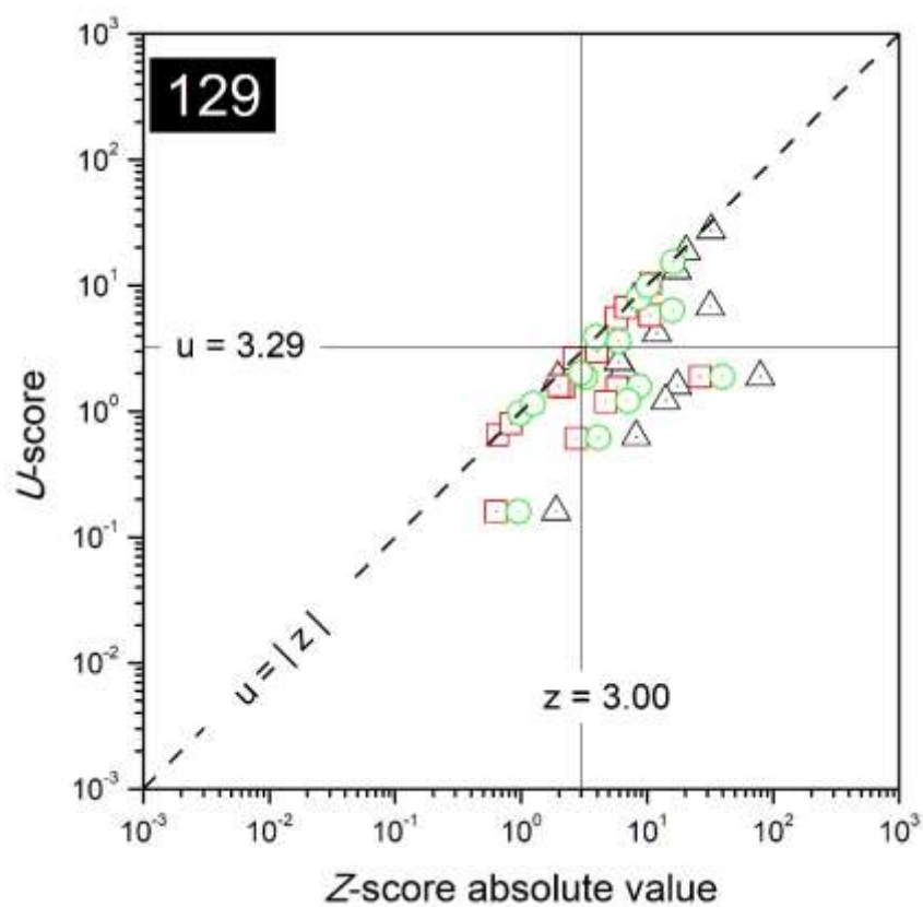
FIG. 76. Combined plots of z- and u-scores for the laboratory with code 129.
