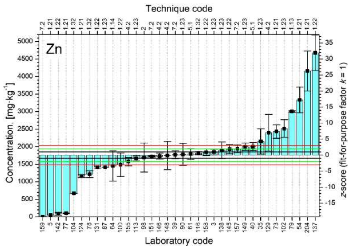
FIG. 50. Distributions of z-scores for analyte Zn.
