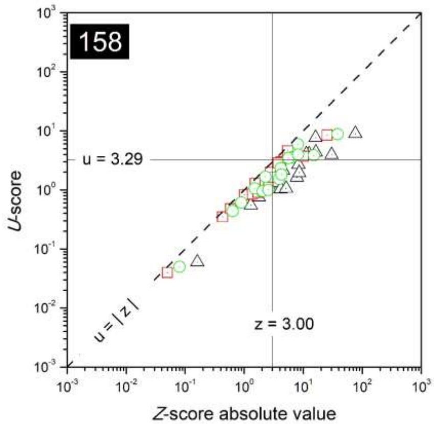
FIG. 91. Combined plots of z - and u -scores for the laboratory with code 158.
