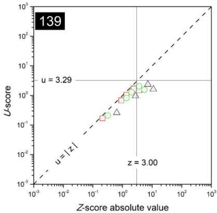
FIG. 80. Combined plots of z- and u-scores for the laboratory with code 139.
