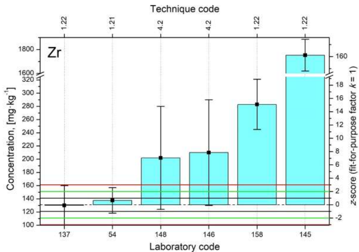
FIG. 51. Distributions of z-scores for analyte Zr.
