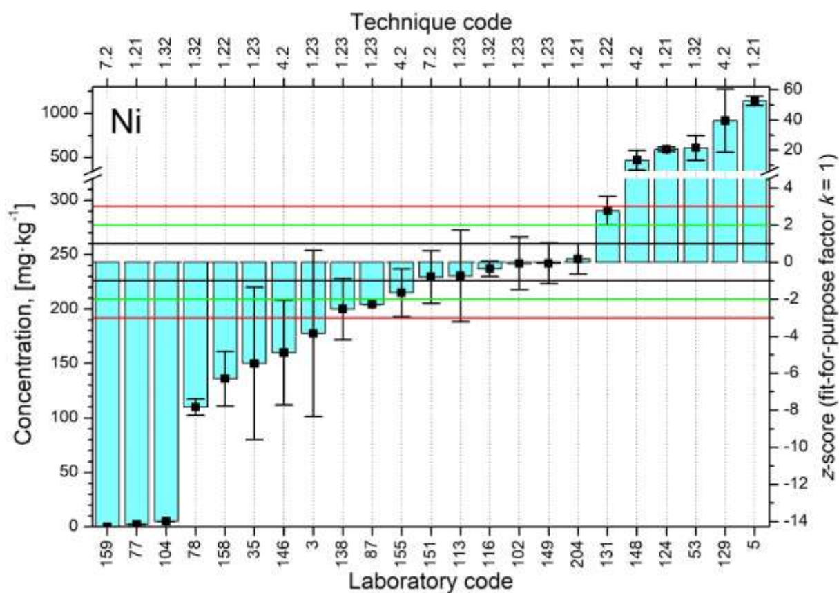
FIG. 41. Distributions of z-scores for analyte Ni.
