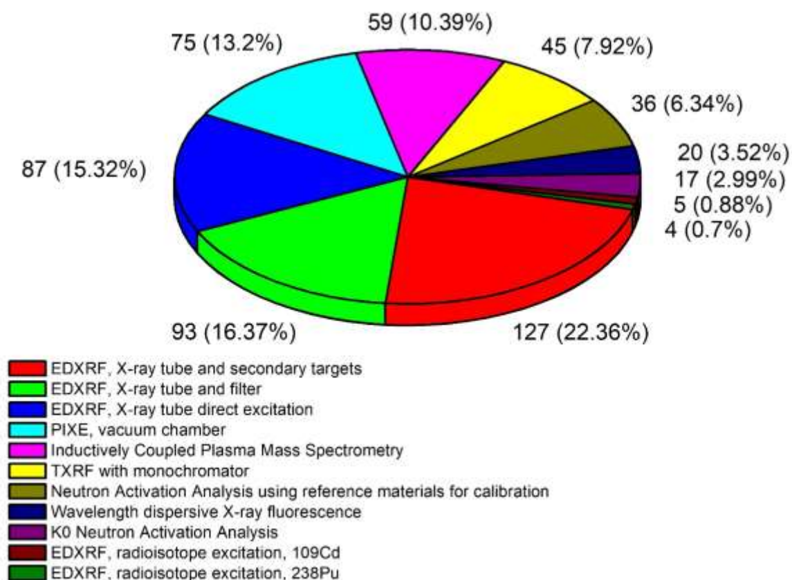
FIG. 95. Utilization of analytical techniques. For each analytical technique the number of submitted results is shown. The percent values relate to the total number of 568 submitted results.
