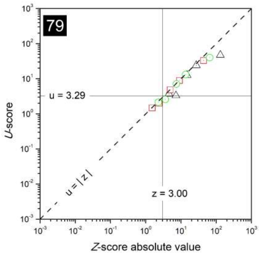
FIG. 65. Combined plots of z - and u -scores for the laboratory with code 79.
