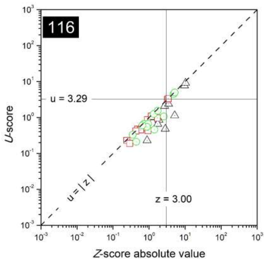
FIG. 74. Combined plots of z - and u -scores for the laboratory with code 116.
