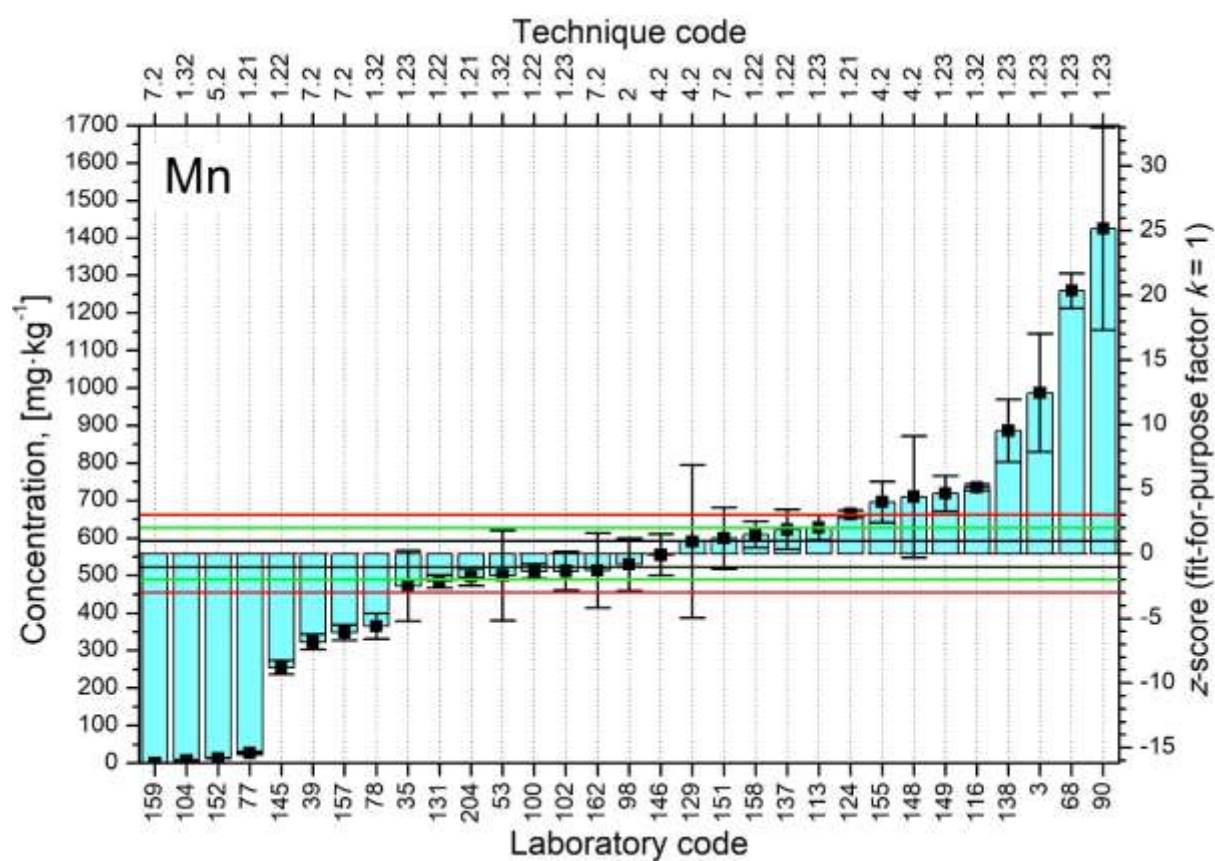
FIG. 39. Distributions of z-scores for analyte Mn.
