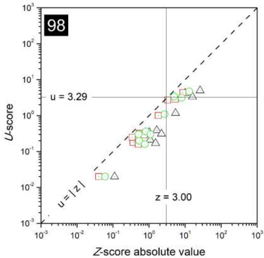
FIG. 69. Combined plots of z - and u -scores for the laboratory with code 98.
