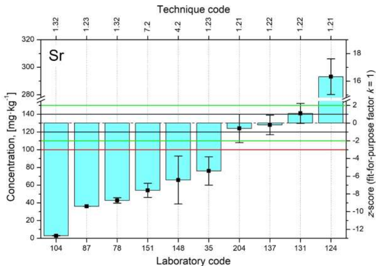
FIG. 47. Distributions of z-scores for analyte Sr.
