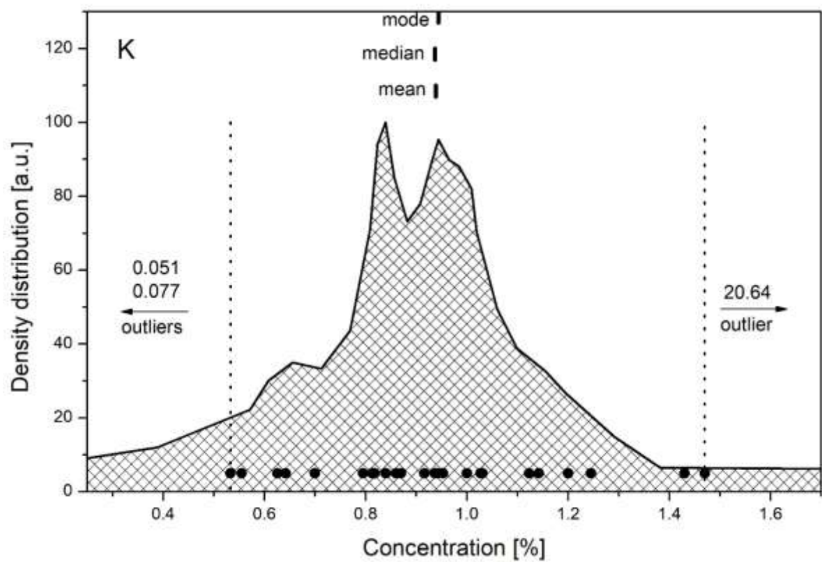
FIG. 12. The density distribution function for the analyte K.
