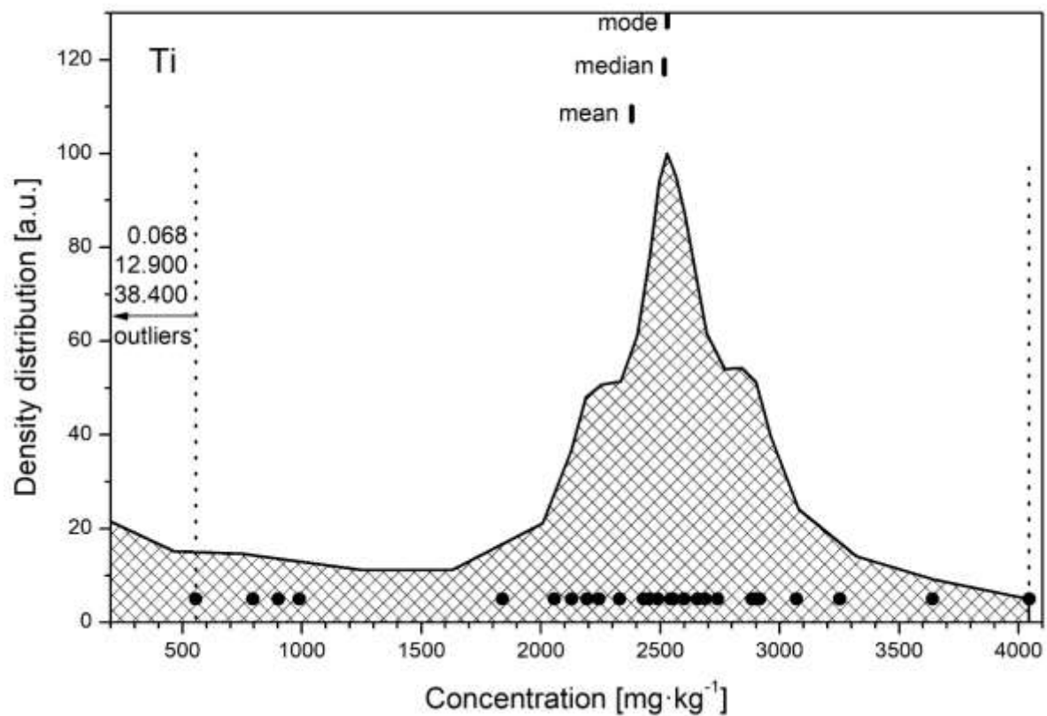
FIG. 25. The density distribution function for the analyte Ti.
