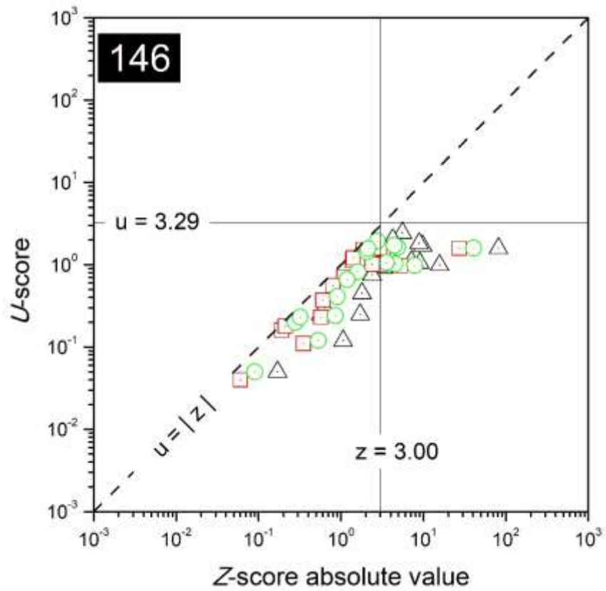
FIG. 83. Combined plots of z- and u-scores for the laboratory with code 146.
