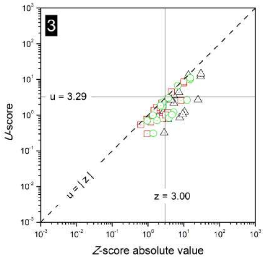
FIG. 52. Combined plots of z- and u-scores for the laboratory with code 3.
