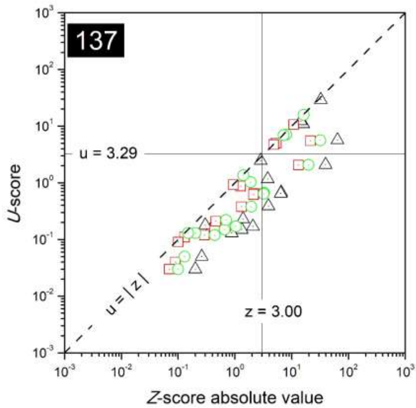
FIG. 78. Combined plots of z- and u-scores for the laboratory with code 137.
