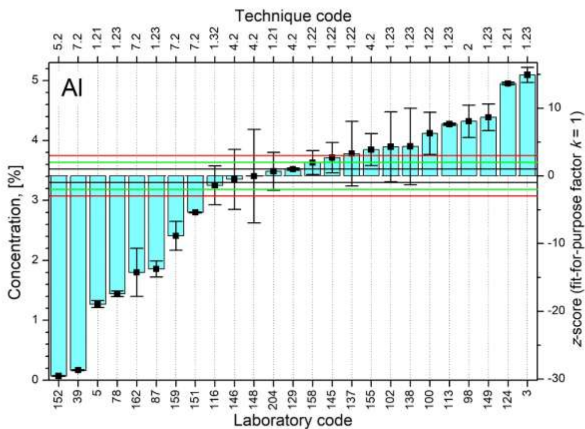
FIG. 29. Distributions of z-scores for analyte Al.
