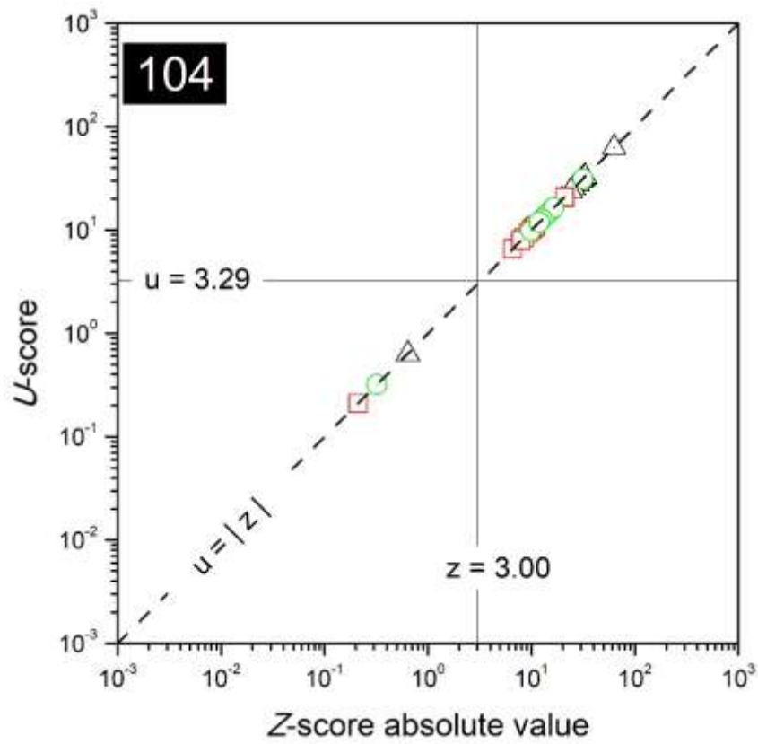
FIG. 72. Combined plots of z- and u-scores for the laboratory with code 104.
