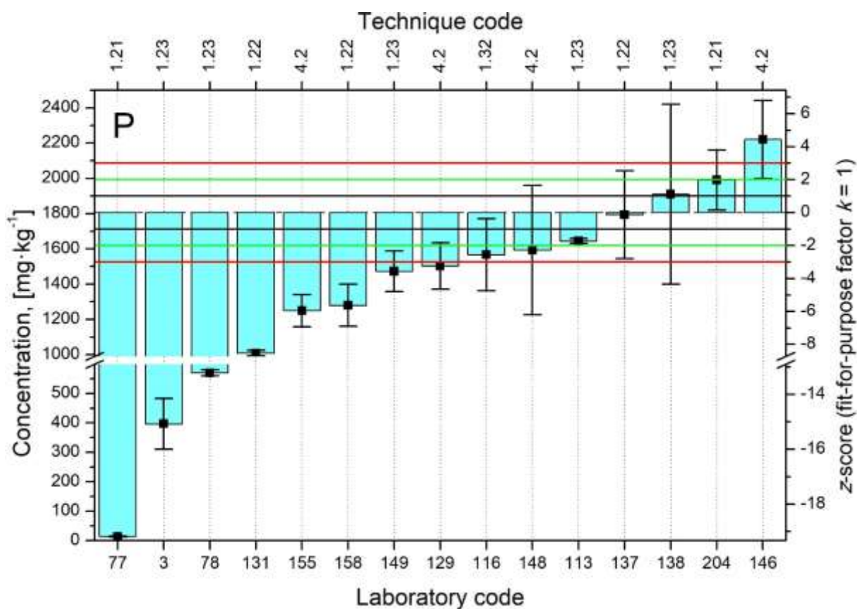
FIG. 42. Distributions of z-scores for analyte P.
