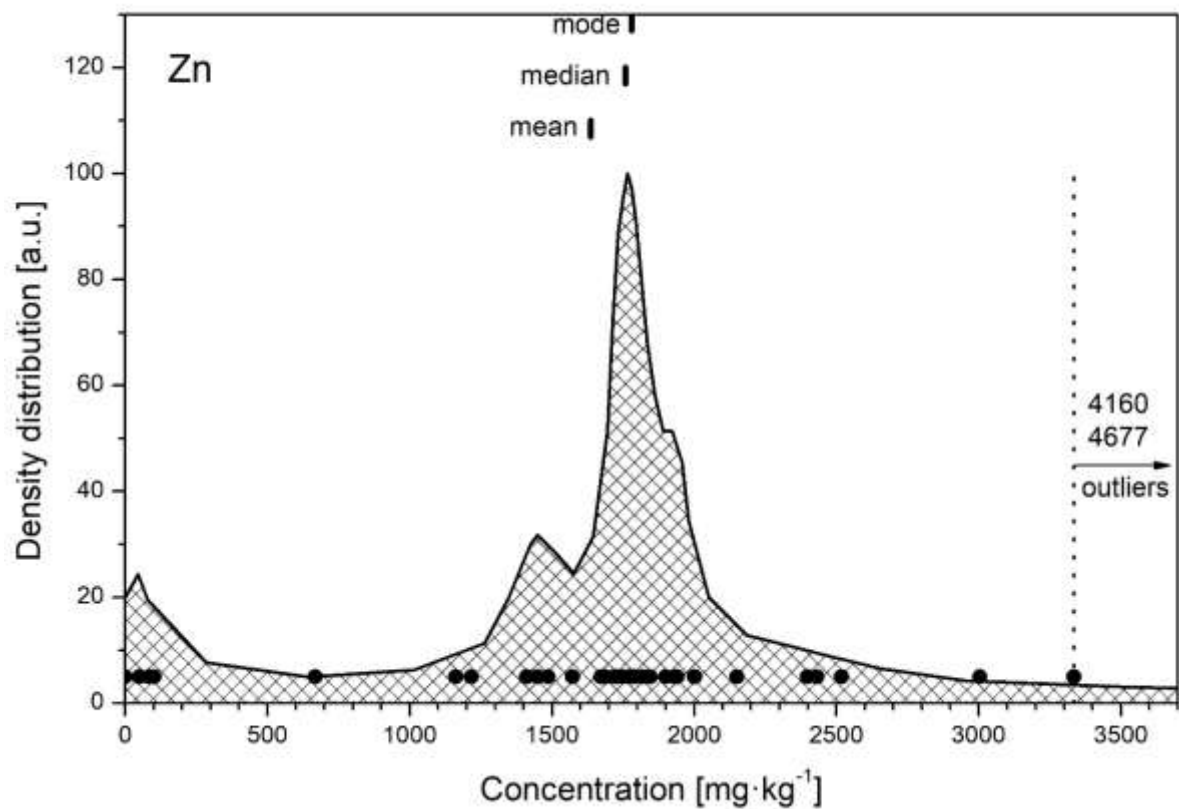
FIG. 27. The density distribution function for the analyte Zn.
