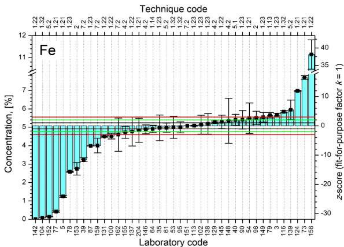
FIG. 35. Distributions of z-scores for analyte Fe.
