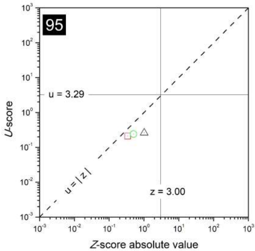
FIG. 68. Combined plots of z - and u -scores for the laboratory with code 95.
