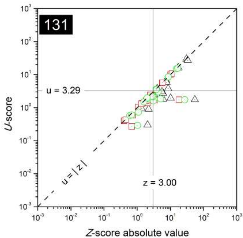
FIG. 77. Combined plots of z- and u-scores for the laboratory with code 131.
