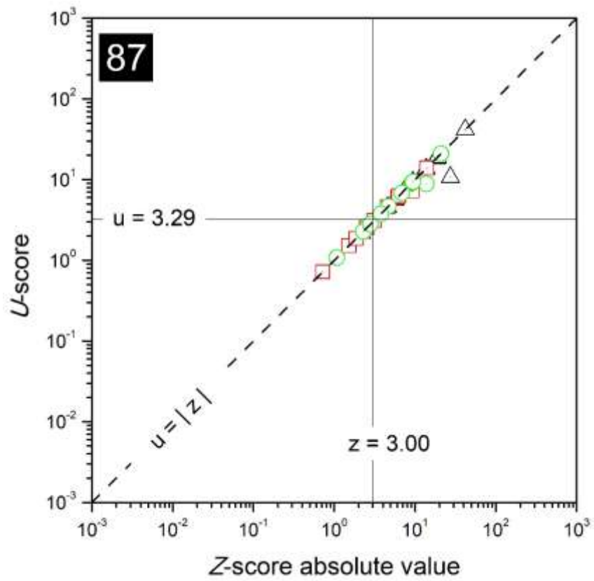
FIG. 66. Combined plots of z- and u-scores for the laboratory with code 87.
