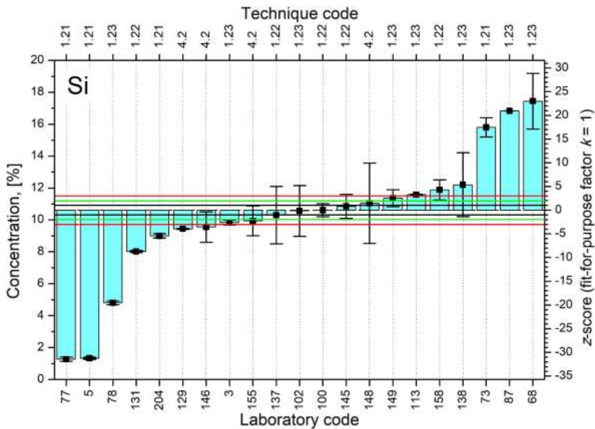
FIG. 46. Distributions of z-scores for analyte Si.
