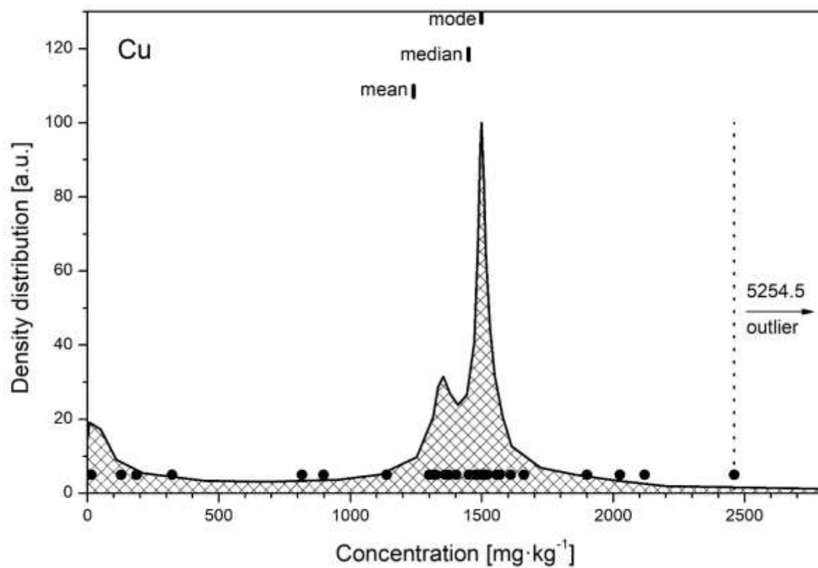
FIG. 10. The density distribution function for the analyte Cu.
