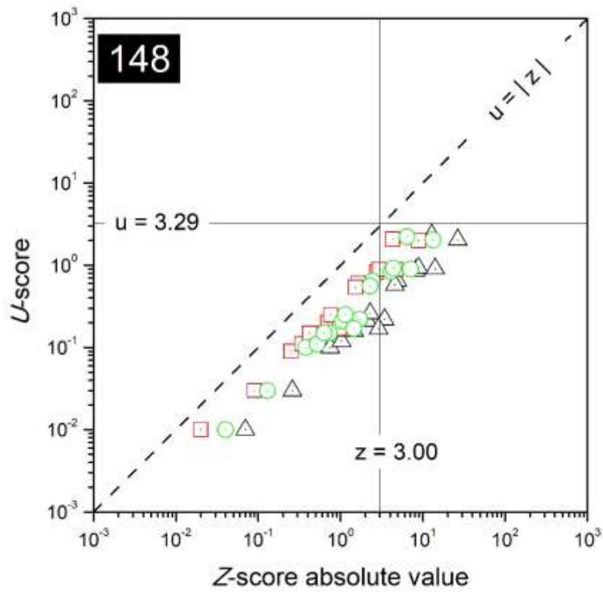
FIG. 84. Combined plots of z - and u -scores for the laboratory with code 148.
