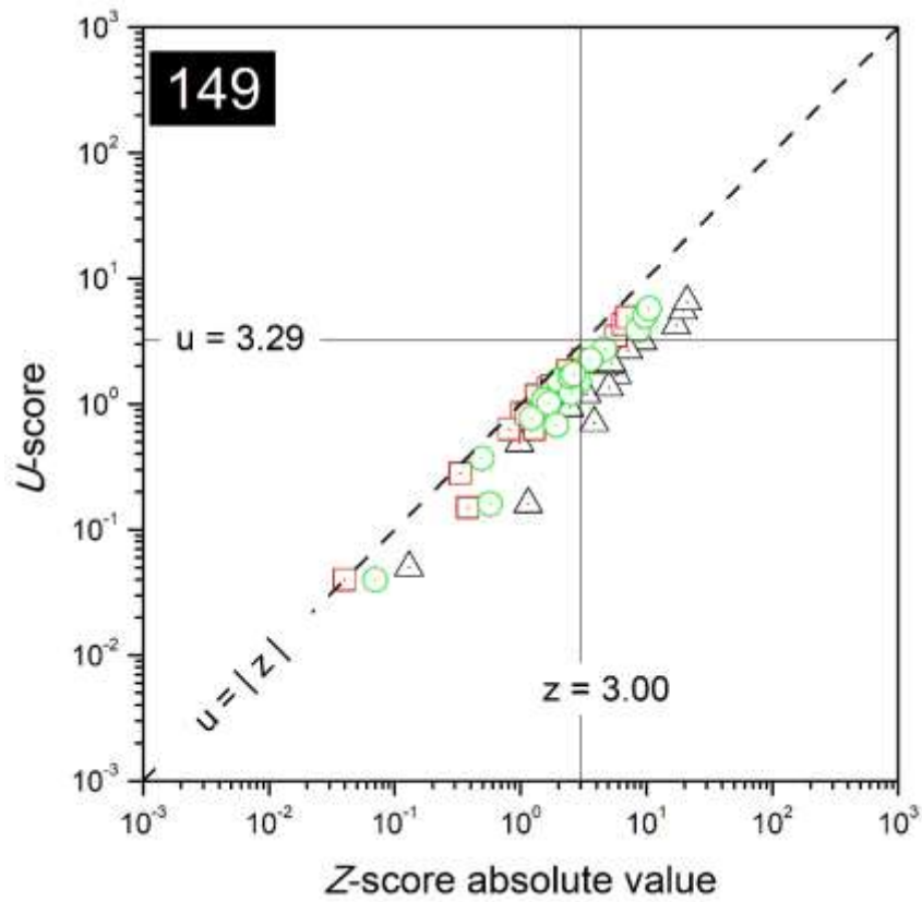
FIG. 85. Combined plots of z - and u -scores for the laboratory with code 149.
