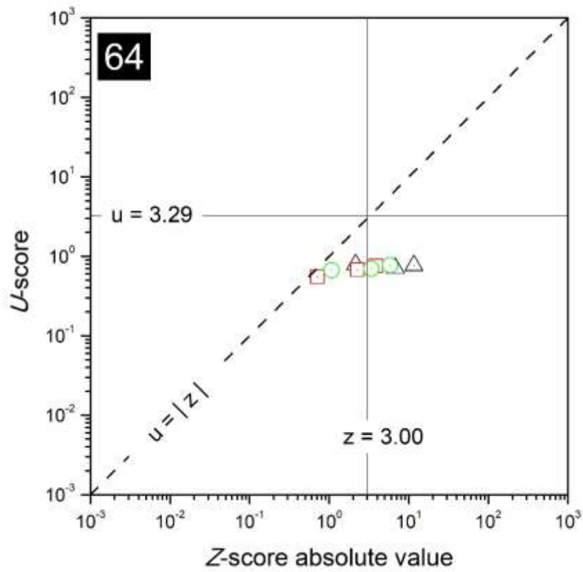
FIG. 60. Combined plots of z- and u-scores for the laboratory with code 64.
