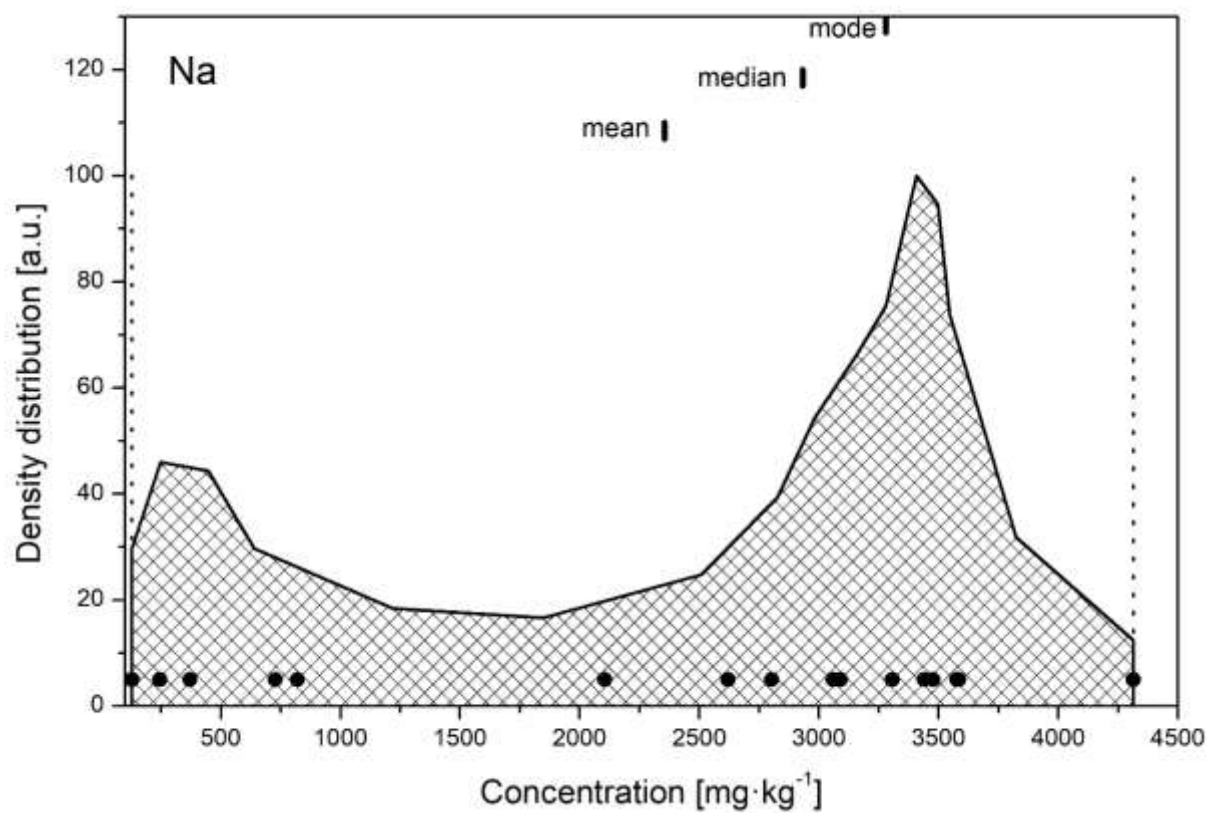
FIG. 16. The density distribution function for the analyte Na.
