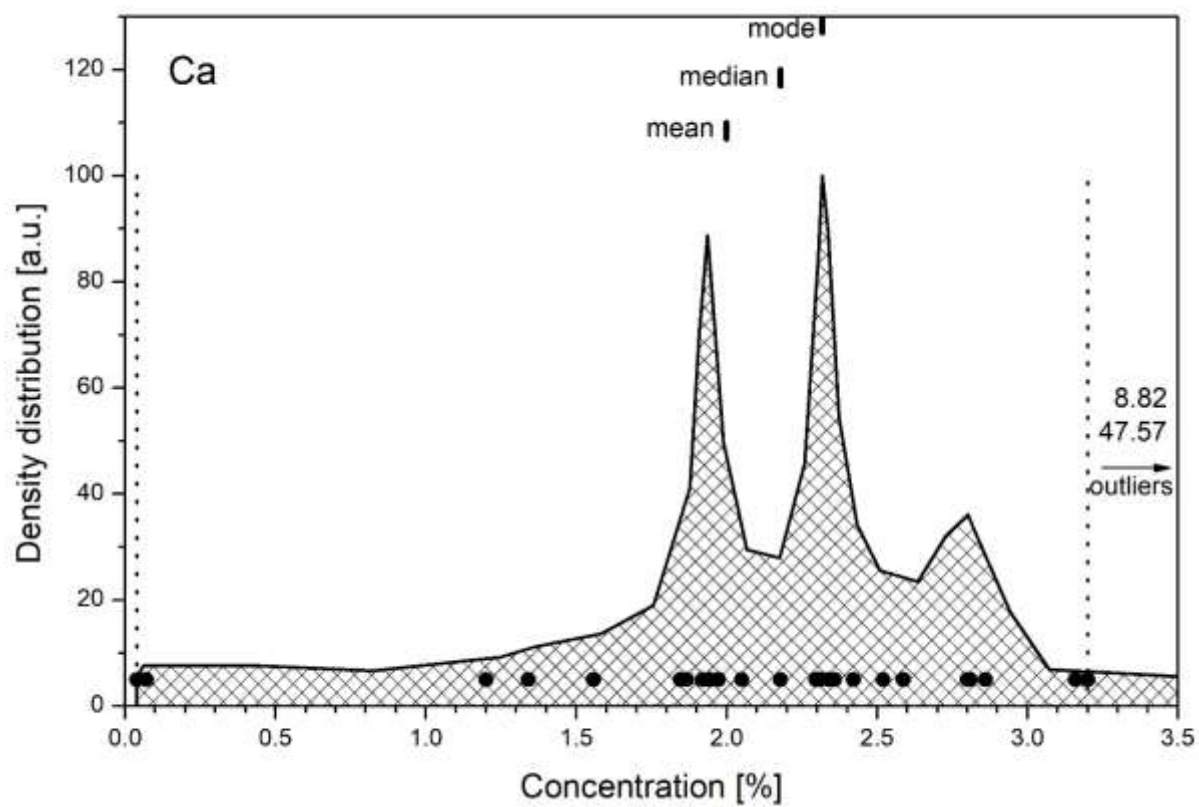
FIG. 6. The density distribution function for the analyte Ca.
