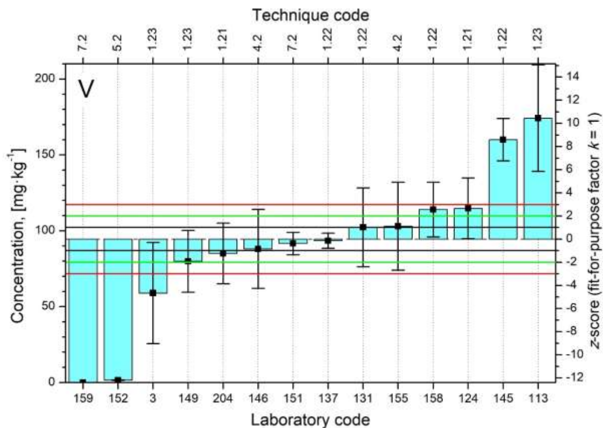
FIG. 49. Distributions of z-scores for analyte V.
