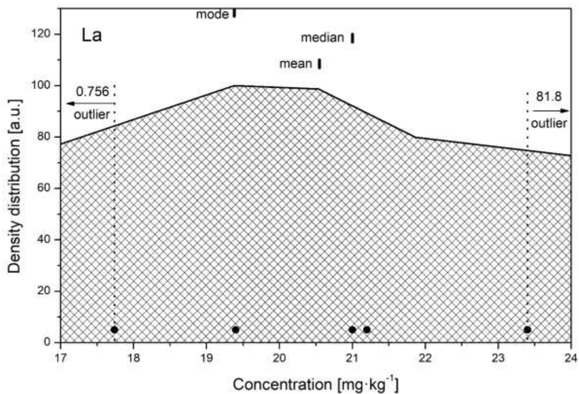
FIG. 13. The density distribution function for the analyte La.
