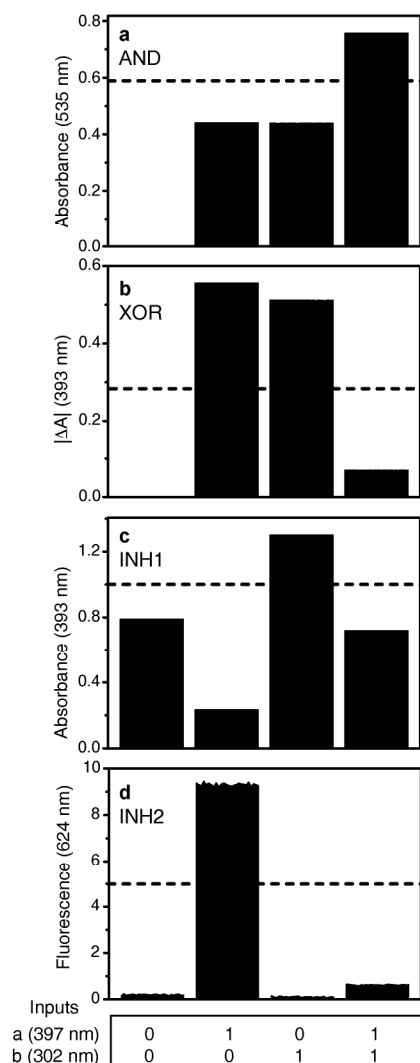
Fig. 6. Performance of arithmetic functions by triad 3 . The states of the two inputs for each column are shown at the bottom. The outputs of the various gate functions are shown in (a) (AND), (b) (XOR), (c) (INH1) and (d) (INH2). The dashed lines represent threshold values, and the top of each bar shows the actual experimental data and associated noise. The half-adder is the combination of AND and XOR, whereas the half-subtractor is XOR combined with INH1 or INH2.
