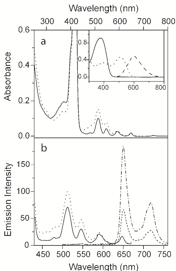
Fig. 2. (a) Absorption spectra of dyad 2 , with the fulgimide in the open form, P-FGo (□□□) and with the fulgimide in the cyclic, closed form P-FGc (•••••). The inset shows the absorption spectra of model fulgimide 1 in the open (□□□□) and cyclic (••••••) forms, and the emission spectrum of FGo (□ □ □ □). (b) Emission spectra of P-FGo (- - -) and the same sample after UV irradiation to form P-FGc (□ • □ • □ • □) with excitation at 470 nm, and corrected fluorescence excitation spectra of P-FGo (□□□□) and the same sample after UV irradiation to form P-FGo (•••••), with detection at 720 nm.
