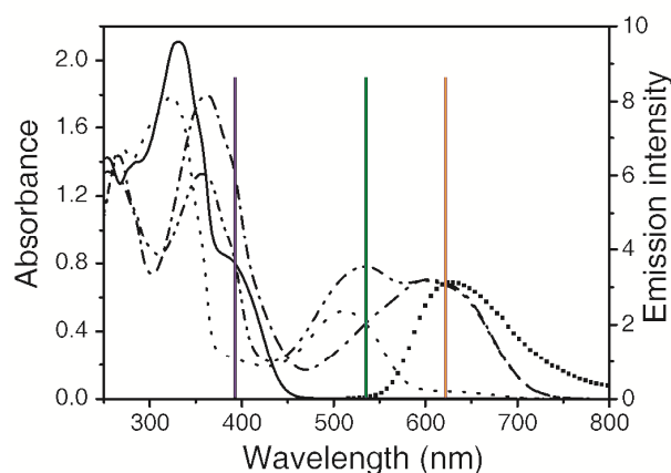
Fig. 4. Absorption and emission spectra of different forms of FG-DTE triad 3 . Solid line: thermally stable FGo-DTEo. Dotted line: FGc-DTEo. Dash-dot: FGo-DTEc. Dash-dot-dot: FGc-DTEc. Also shown is the emission from FGc in the FGo-DTEo form of the molecule (squares). The coloured vertical lines indicate wavelengths that are used as outputs for the various binary arithmetic functions of the triad.
