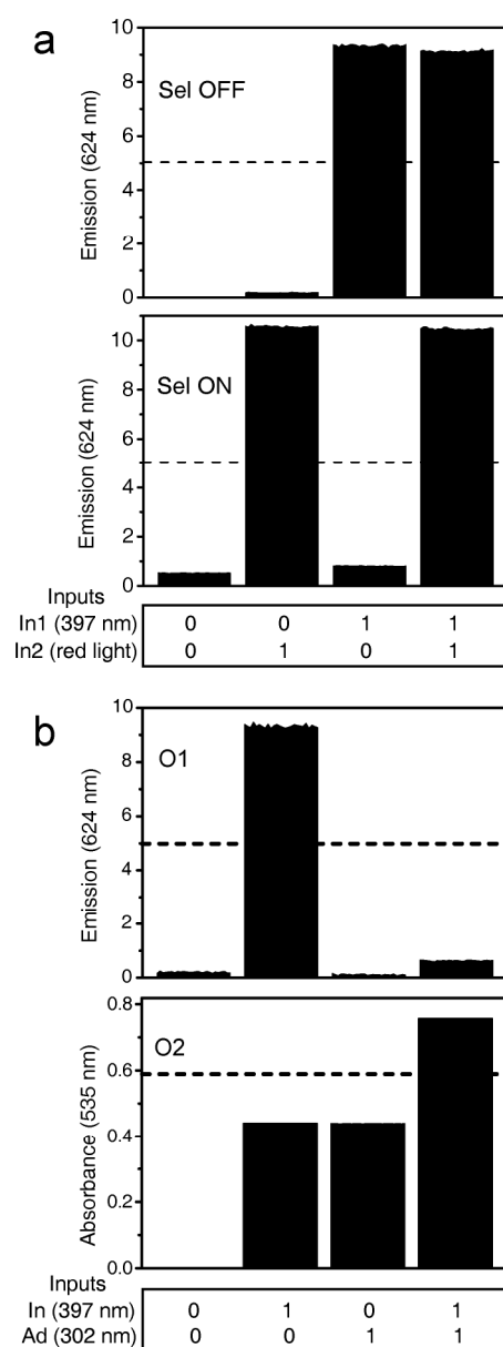
Fig. 7. (a) Triad 3 operation as a 2:1 digital multiplexer. The upper and lower sections show the output of the multiplexer with the Sel input OFF or ON under the application of the two inputs as shown at the bottom of the Figure. (b) Triad 3 as a 1:2 digital demultiplexer. The upper and lower sections show outputs O1 and O2 under the application of the data input at 397 nm when the Ad input is ON (1) or OFF (0).
