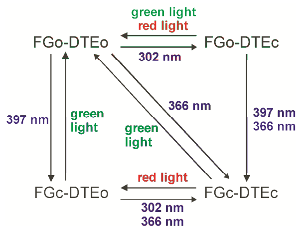
Fig. 5. Photochemical isomerizations among the 4 isomers of 3 that are relevant for the logic operations discussed. Green light signifies ( 460 < \lambda < 590 nm) and red light indicates \lambda > 615 nm.
