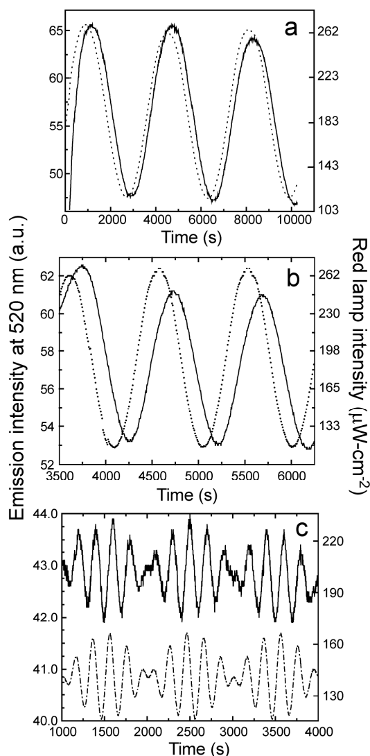
Fig. 10. Performance of hexad 4 as a molecular photonic “triode” tube. In each section, the solid curve shows the intensity at 520 nm of emission from the BPEA fluorophores. The broken curves show the intensity of the modulating red light beam. (a) Frequency modulation with a sine wave having a period of 3600 s. (b) Frequency modulation with a sine wave having a period of 960 s. (c) Amplitude modulation with the product of 2 sine waves having periods of 200 s and 2000 s.
