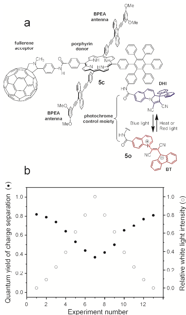
Fig. 11. (a) Pentad 5 , which functionally mimics photosynthetic regulation in cyanobacteria. In 5c , the DHI photochrome has no effect on the photoinduced electron transfer behaviour of the remainder of the molecule. In 5o , the open, betaine form of the photochrome quenches the porphyrin excited singlet state, and reduces the yield of charge separation to 1%. (b) Performance of 5 . Thirteen experiments are shown along the abscissa. The solid circles report the quantum yield of photoinduced electron transfer for the solution of 5 after irradiation with white light at different intensities (hollow circles). As irradiation with white light increases, the quantum yield decreases.
