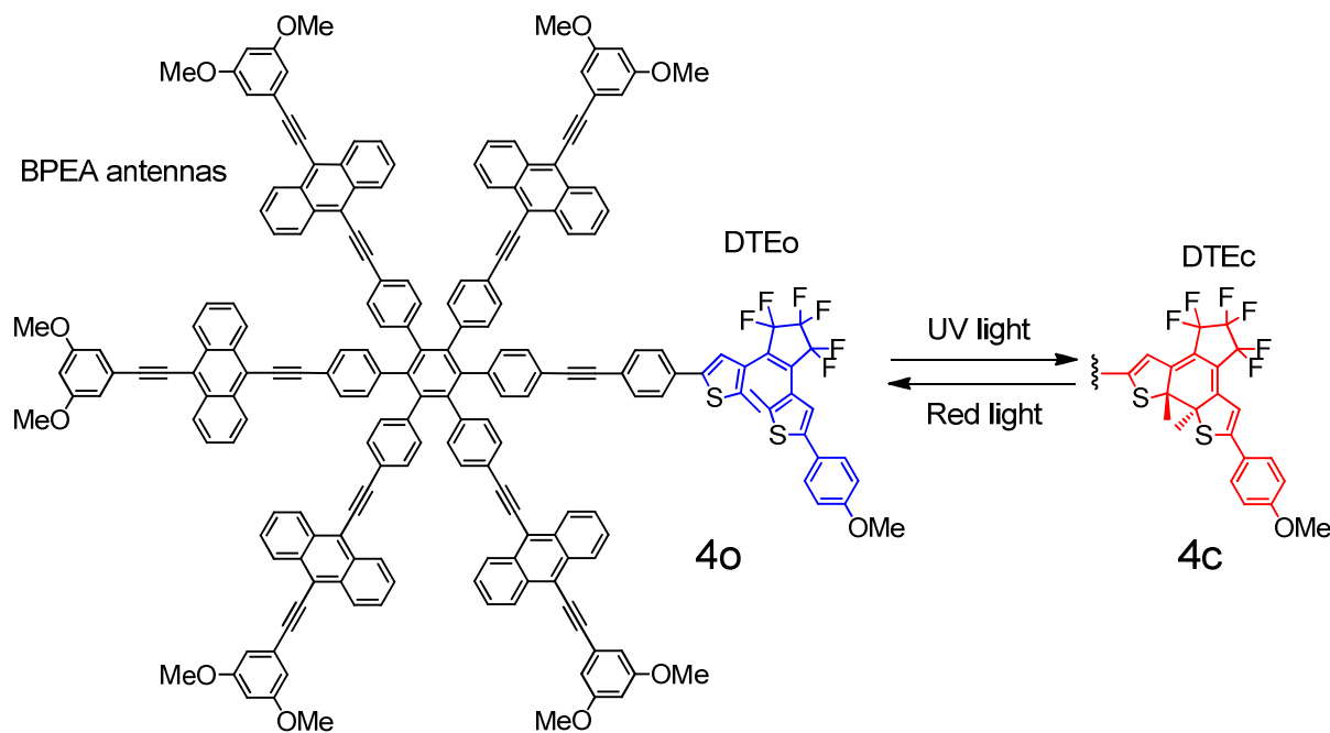
Fig. 9. Molecular “triode” 4 . In 4o , the dithienylethene photochrome is in the open form, which absorbs only UV light. In 4c , the dithienylethene is in the closed, cyclic form that absorbs in the red region.
