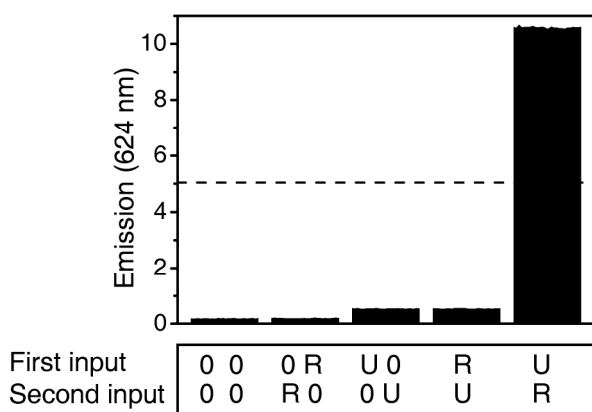
Fig. 8. Triad 3 as a keypad lock. Shown is the output of the lock (fluorescence at 624 nm) that results from sequential application of the inputs in the ON (R = red light >615 nm, U = UV light at 366 nm) or OFF (0) states. Note that an output above the threshold (dashed line) is only obtained if the U input is applied first, and the R input second.
