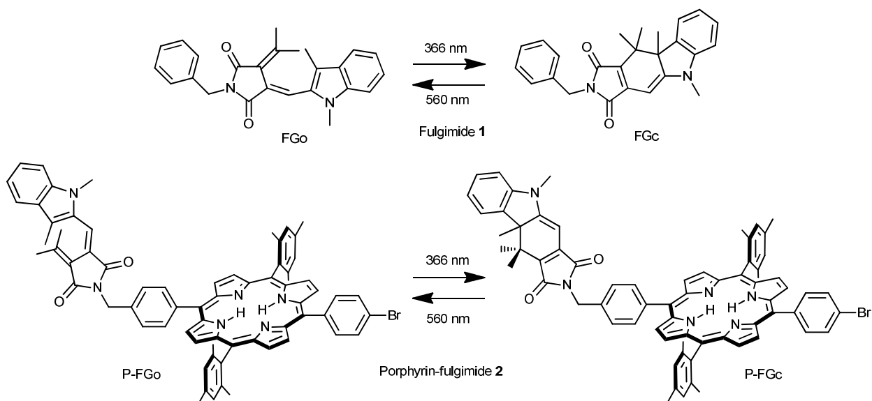
Fig. 1. Structures of fulgimide photochrome 1 and porphyrin-fulgimide dyad 2 . Each molecule is shown with the photochrome in the open (FGo) and closed (FGc) forms, and wavelengths for photoisomerization between the two forms of each molecule are indicated.
