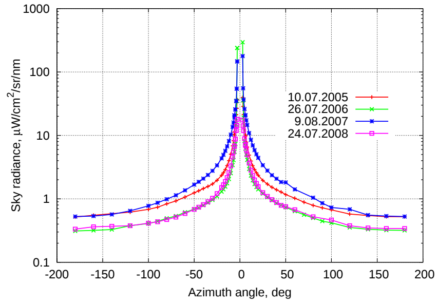
Figure 6.4: Almucantar sky radiance at Tõravere, 870 nm.
