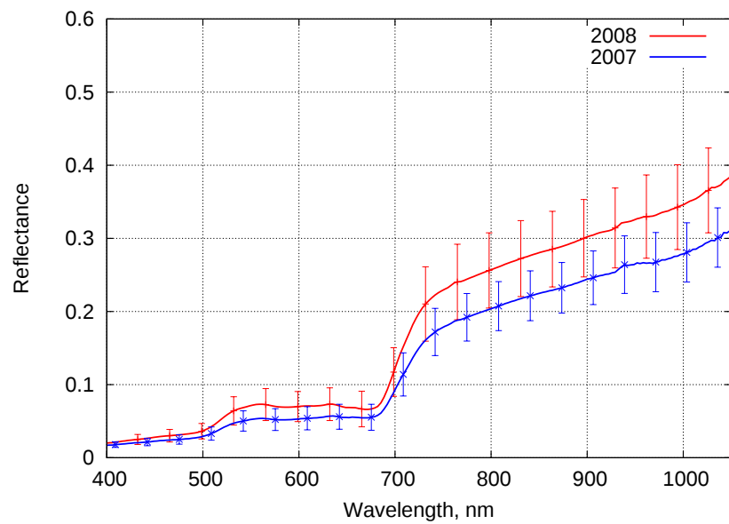
Figure 6.46: Average reflectance of understorey vegetation in the spruce stand. Error bars show the standard deviation of nine mean reflectance at LAI points L1-L9.
