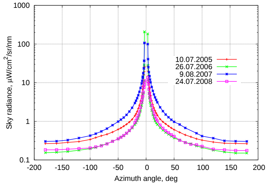
Figure 6.3: Almucantar sky radiance at Tõravere, 1020 nm.
