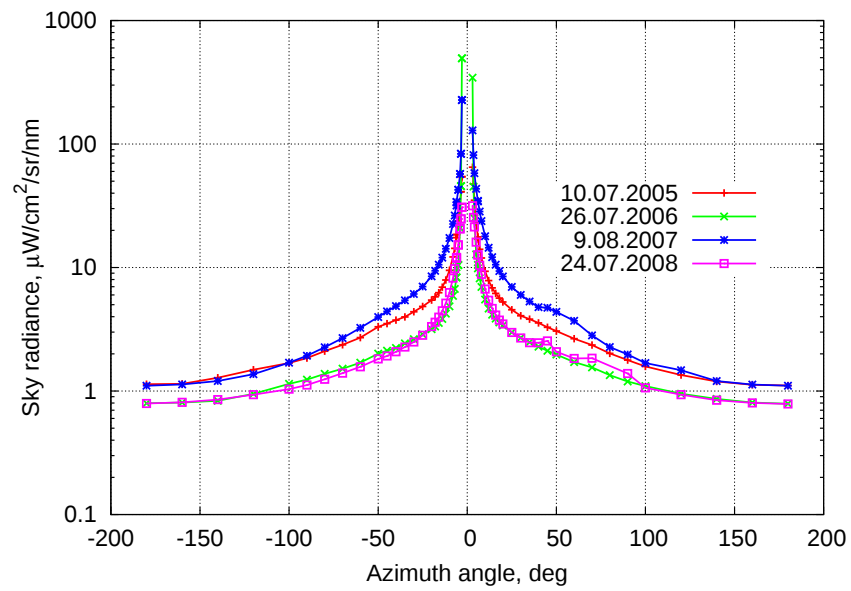
Figure 6.5: Almucantar sky radiance at Tõravere, 675 nm.
