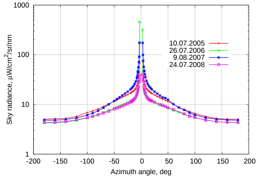
Figure 6.6: Almucantar sky radiance at Tõravere, 440 nm.
