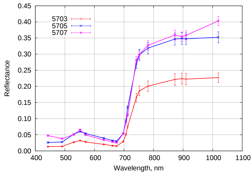
Figure 6.48: Average top-of-canopy directional reflectance of the spruce stand from CHRIS images.
