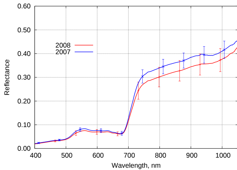
Figure 6.35: Average reflectance of understorey vegetation in the pine stand. Error bars show the standard deviation of nine mean reflectance at LAI points L1-L9.
