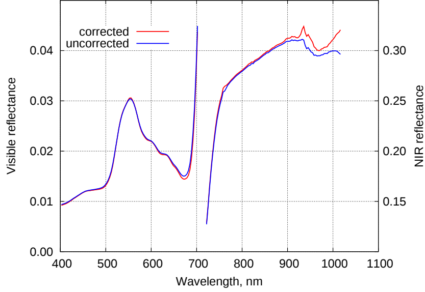
Figure 5.1: Stray light and aliasing correction of a reflectance spectrum.
