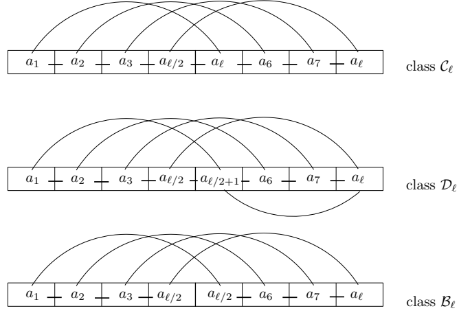
Figure 10: The classes \mathcal{B}_\ell, \mathcal{C}_\ell , and \mathcal{D}_\ell .
