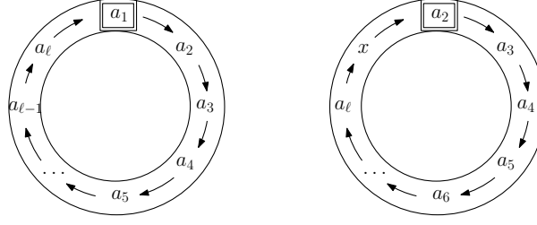
Figure 3: The disc representation of a vertex u = a_1 a_2 \dots a_{\ell-1} a_{\ell} of CK(d, \ell) and its neighbor v = a_2 a_3 \dots a_{\ell} x , that is, (u, v) is an arc in CK(d, \ell) .
