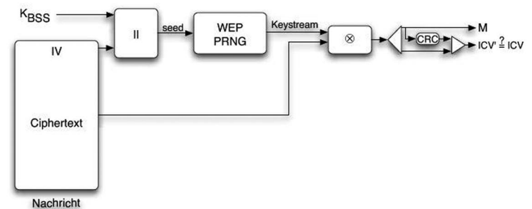
Abb. 27: WEP-Entschlüsselung
