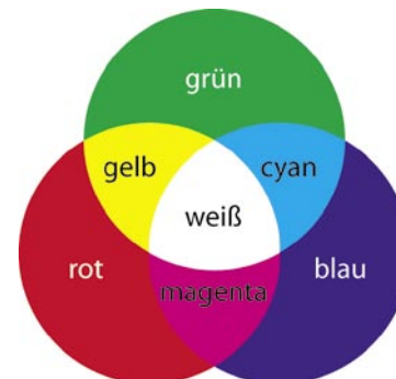
Abb. 44: Additive Farbsynthese
