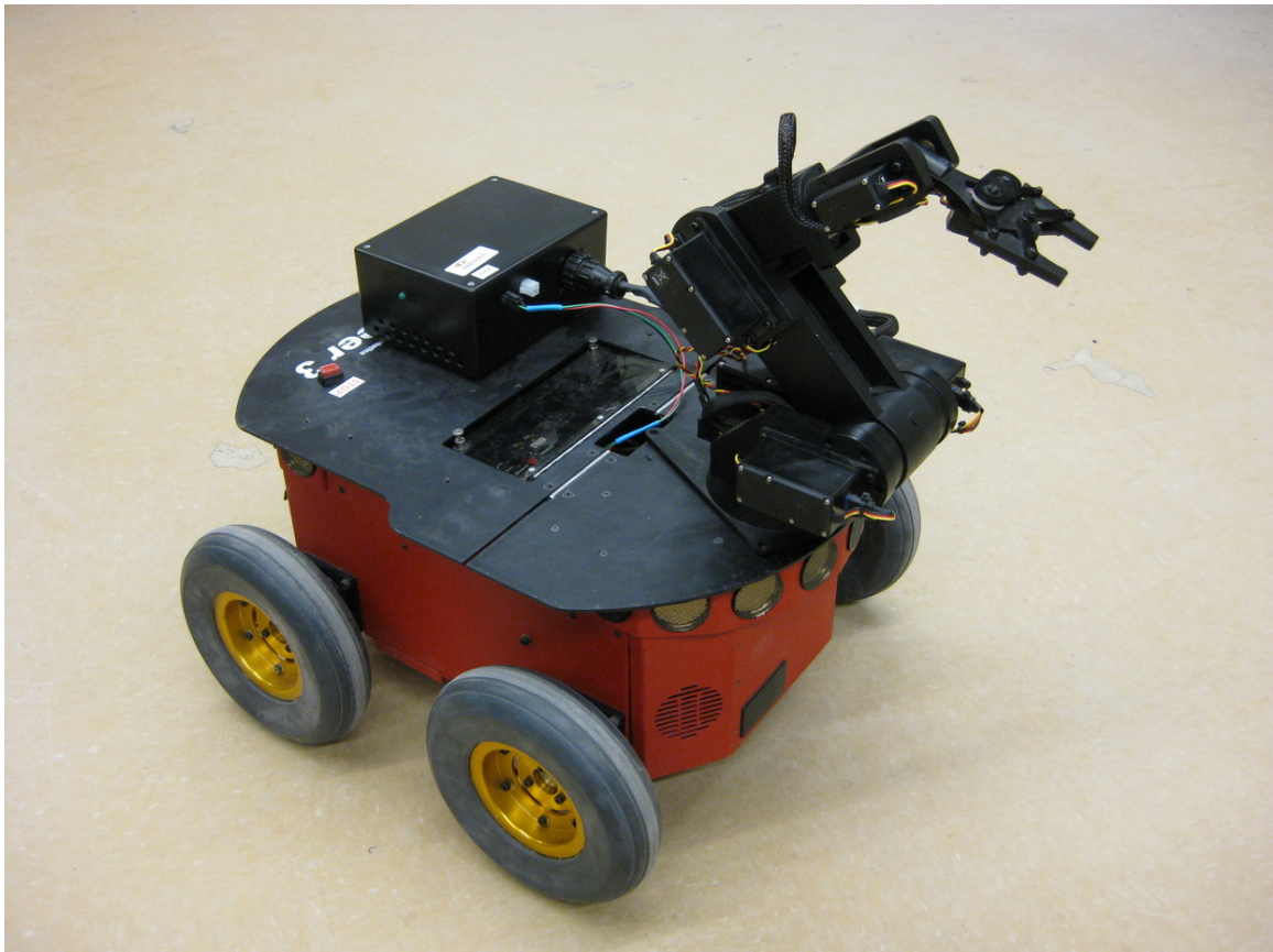
Figure 60 The Pioneer 3-AT robot has four motors and four unsteered wheels; on each side a pair of motors drives a pair of wheels through a single belt.
