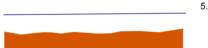
Plane bed
