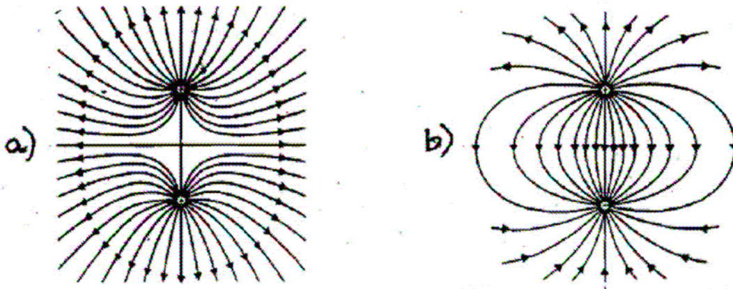
Figure 9.1 - Two examples of electric fields created by two equal charges.
