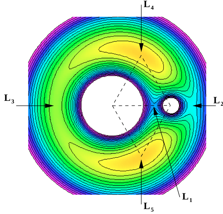
Figure 2: A countour plot of the generalised potential.
