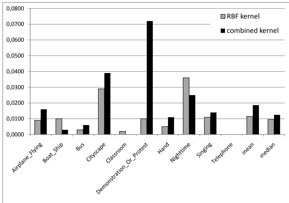
Fig. 1. Comparison of infAP of the two kernels on the 10 concepts of the light run.
