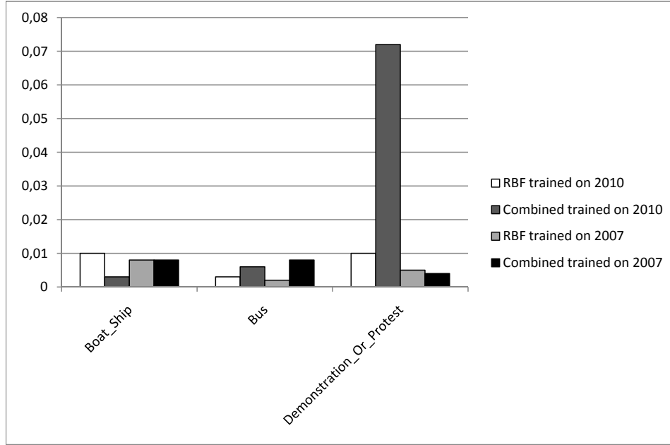
Fig. 2. Comparison of infAP of the three shared concepts for the different kernels trained on 2007 and 2010 data sets.
