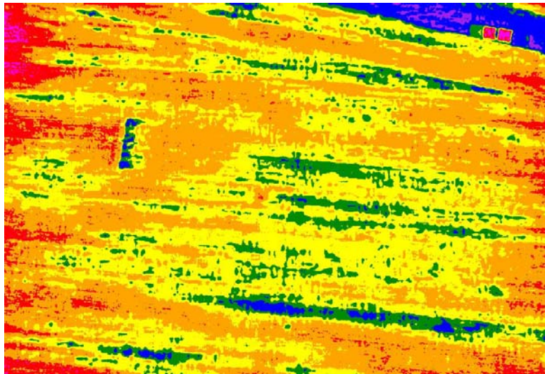
Figure 5. Variation of green normalized difference vegetation index (GNDVI). The amount of vegetation is shown by the color (purple 0.00-0.50, blue 0.50-0.57, green 0.57-0.64, yellow 0.64-0.71, orange 0.71-0.78, red 0.78-0.85, magenta 0.85-1.00). Higher values of GNDVI occur around the edges of the photograph because of lens vignetting and more oblique view angles.
