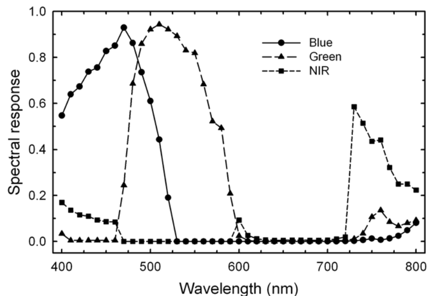
Figure 3. Relative spectral calibration of the Fuji FinePix S3 Pro UVIR camera for the blue, green, and red/NIR channels. A custom red-blocking filter was used to block photons (610 to 720 nm) from the red/NIR channel, so only NIR photons were detected.
