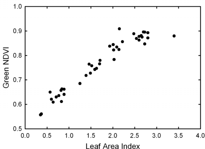
Figure 6. Relationship of GNDVI with leaf area index (LAI) in winter wheat. For LAI from 0 to 2.5 \text{ m}^2 \text{ m}^{-2} , the regression equation is \text{GNDVI} = 0.5 + 0.16 \text{ LAI} , with an R^2 of 0.85.
