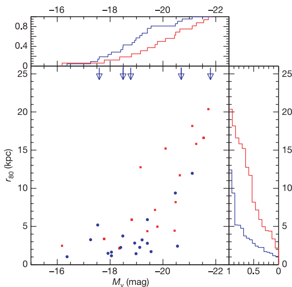
Figure 4 | A comparison of the absolute magnitude and size distributions of the GRB and supernova hosts. In the main panel, the core-collapse supernova hosts are represented as red squares, and the LGRB hosts as blue circles. The absolute magnitudes of the hosts are shown on the x axis, and the lengths of the semi-major axes of the hosts on the y axis. The plot is then projected onto the two side panels where a histogram is displayed for each host population in each of the dimensions—absolute magnitude and semi-major axis. Shown as blue arrows are the absolute magnitudes of GRB hosts with z < 1.2 that have been detected from the ground but have not yet been observed by HST. These hosts are only included in the absolute magnitude histogram. The hosts of GRBs are both smaller and fainter than those of supernovae.
