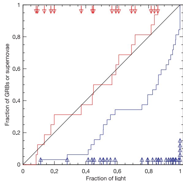
Figure 3 | The locations of the explosions in comparison to the host light. For each object, an arrow indicates the fraction of total host light in pixels fainter than or equal to the light in the pixel at the location of the transient. The cumulative fraction of GRBs or supernovae found at a given fraction of the total light is shown as a histogram. The blue arrows and histogram correspond to the GRBs, and the red arrows and histogram correspond to the supernovae. Were the GRBs and supernovae to track the light identically, their histograms would follow the diagonal line. Whereas the supernova positions do follow the light within the statistical error, the GRBs are far more concentrated on the brightest regions of their hosts. Thus although the probability of a supernova exploding in a particular pixel is roughly proportional to the surface brightness of the galaxy at that pixel, the probability of a GRB at a given location is effectively proportional to a higher power of the local surface brightness.
