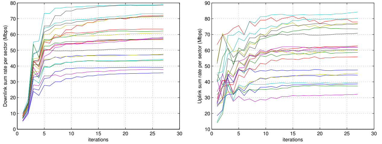
Fig. 5. Convergence of downlink (left) and uplink (right) per-sector sum rates in each of the 21 sectors with dynamic spectrum allocation and coordinated beamforming. Each iteration is either a joint user scheduling and beamforming step, or a power allocation step. Each beamforming step consists of fixed 3 inner downlink transmit beamformer and power iterations and 5 outer downlink receive beamformer updates (for a total of 15 iterations.) Each power allocation step involves up to 10 iterations. The proportional fairness weights are also updated at the same time.
