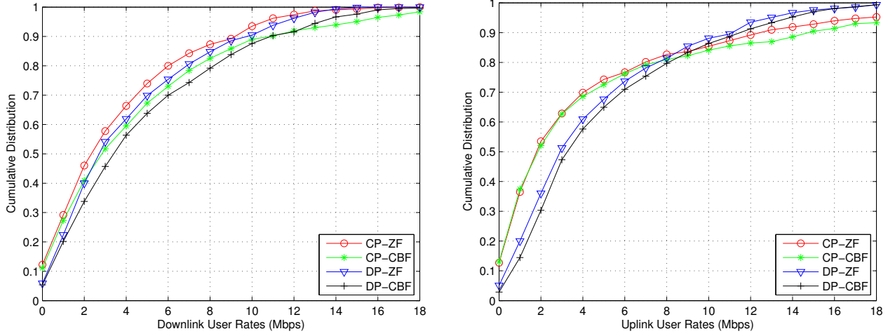
Fig. 4. Cumulative distribution function of user rates with dynamic power spectrum adaptation (DP) vs constant power (CP), and coordinated beamforming (CBF) vs zero-forcing (ZF). Cell diameter is 2.8km
