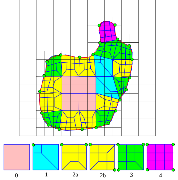
Figure 7: Top row - an example of adaptive quad mesh generation in 2D. Each green point represents a minimizer point of a cell to be refined, and the red curve represents the real isocontour. Bottom row - the decomposition templates of Method 3 shown in Figure 3.
