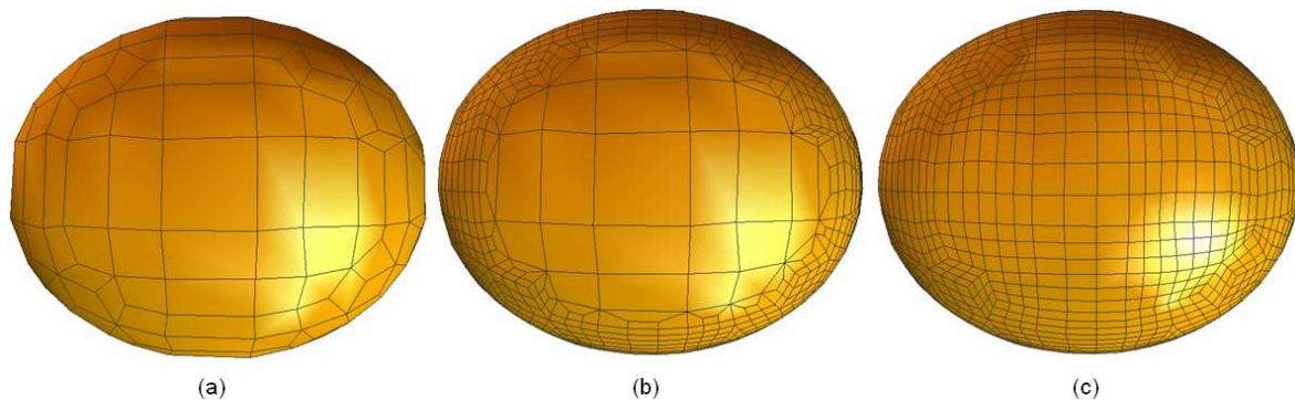
Figure 21: Quadrilateral meshes of a bubble model. (a) - the uniform mesh at a chosen starting level; (b) - an adaptive mesh controlled by finite element solutions (deformation); (c) - a mesh generated by refining all the elements in (a).
