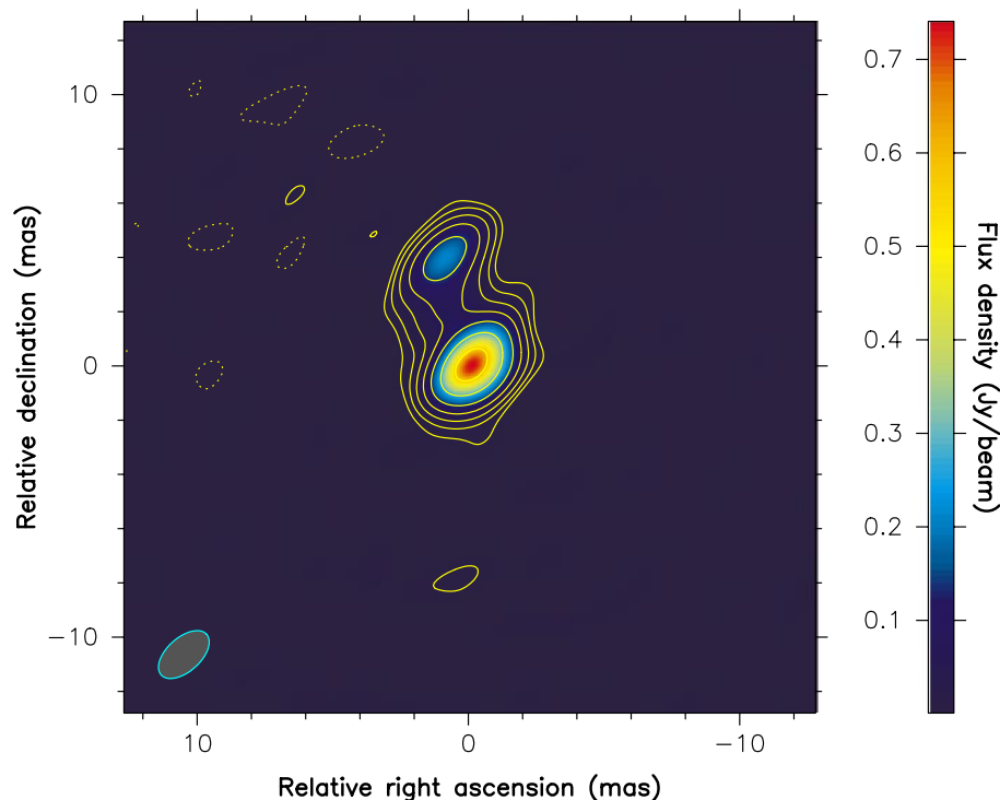
Fig. 3. A 1.6-GHz image of the quasar 1548+056 made from an observation with HALCA (using the Goldstone and Usuda tracking stations) and from telescopes in Australia, China, and Japan. The synthesized beam is 2.3 mas by 1.3 mas (FWHM) at a position angle of -48.2^\circ . The residual noise level in the image is 3.6 mJy per beam (rms). The contours are at -1, 1, 2, 4, 8, 16, 32 , and 64 times 9 mJy per beam. At the distance of the quasar, 1 mas corresponds to 18.6 light-years.
