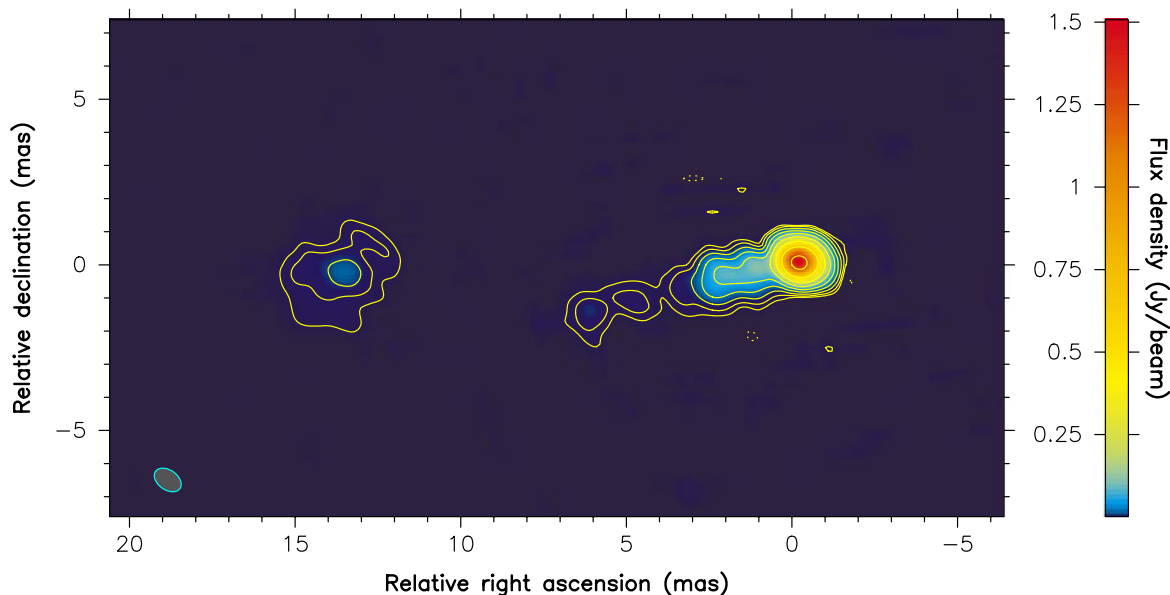
Fig. 4. A 1.6-GHz image of the high-redshift quasar 0014+813 made from an observation on 16 September 1997 with HALCA (using the Goldstone, Green Bank, and Tidbinbilla tracking stations), telescopes of the European VLBI Network, and the Green Bank 43-m telescope. The synthesized beam is 2.0 mas by 0.98 mas (FWHM) at a position angle of 6.2^\circ . The residual noise level in the image is 0.9 mJy per beam (rms). The contours are at -1, 1, 2, 4, 8, 16, 32 , and 64 times 3 mJy per beam. At the distance of the quasar, 1 mas corresponds to 15.1 light-years.
