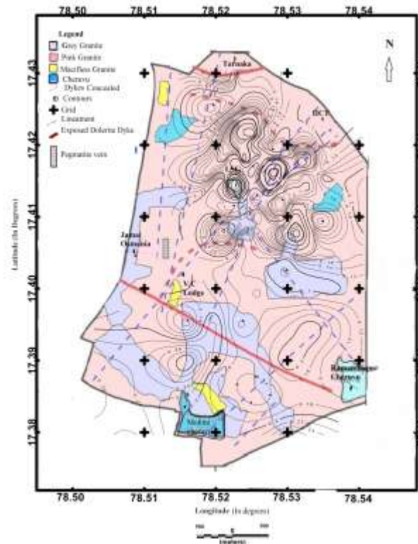
Fig.4. Porosity contour map of the study area
