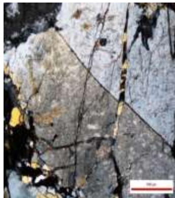
Fig.7. Thin section near Microbiology Department
