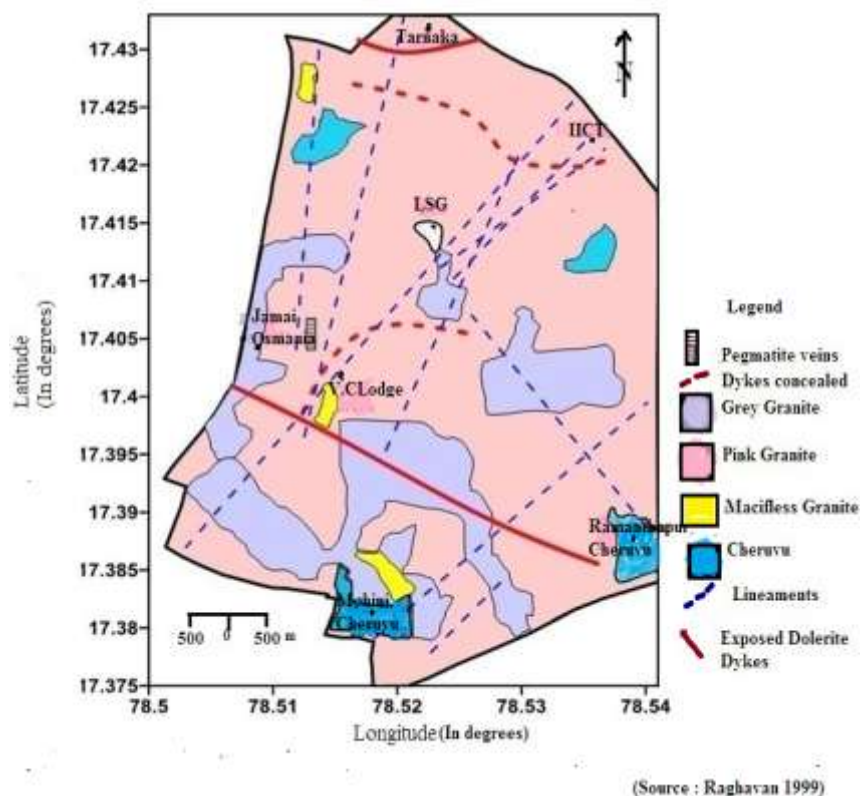
Fig.1. Geology map of the study area
