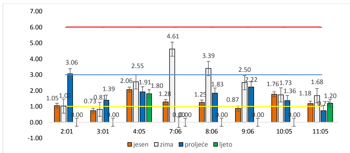
Figure 3. Graphic representation of Cd contamination factors in sediment
