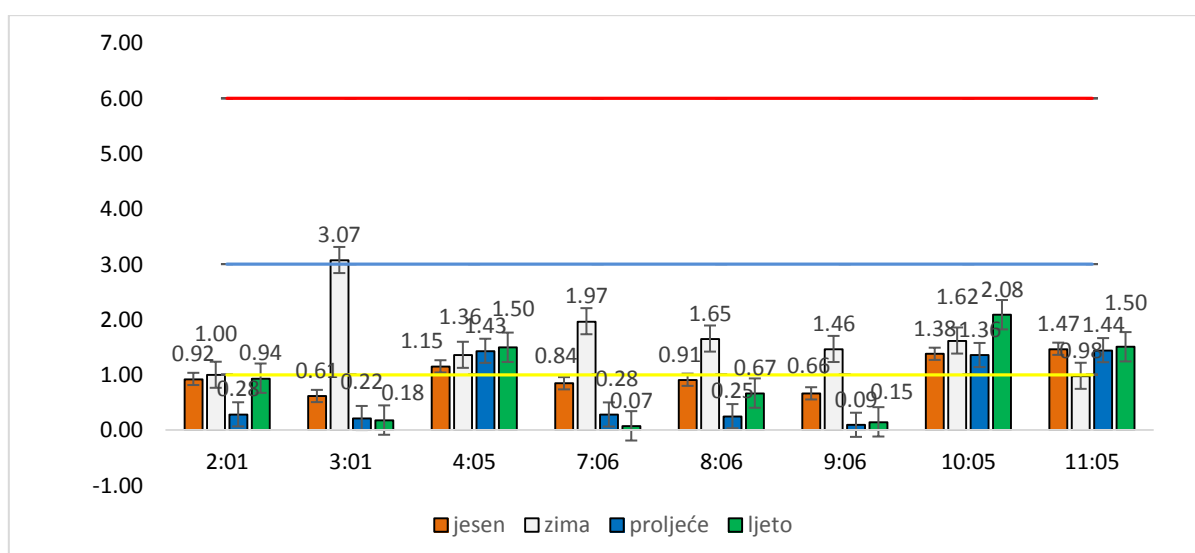
Figure 6. Graphical representation of contamination factors for Mn in sediment
