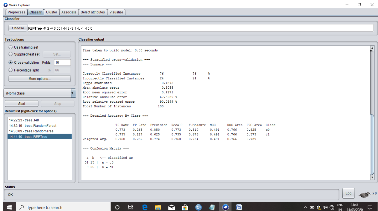
Fig 3. Reptree output
