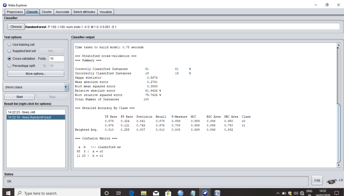
Fig 2. Random Forest Output
