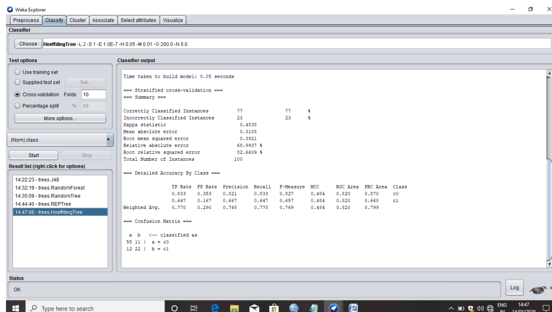
Fig 5. Hoeffding Tree Output
