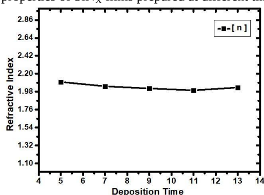
Fig.4. Effect of the deposition times of the SiN x film on refractive index.
