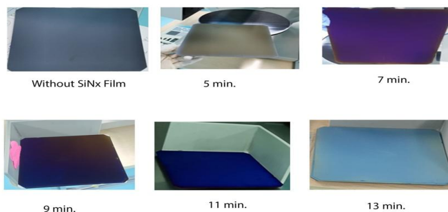
Fig. 6. Effect of the deposition time on the homogeneity of the SiN x films deposited on monocrystalline silicon solar cells.
