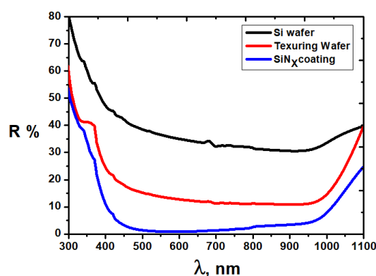
Fig.9. Reflectance of a planar monocrystalline Si wafer, a textured monocrystalline Si wafer, and a textured Si wafer coated with a SiN x film.
