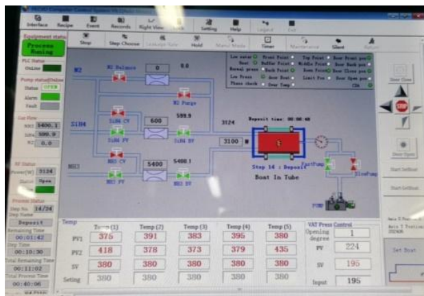
Fig.2. SiN x film deposition parameters setting in PECVD equipment.
