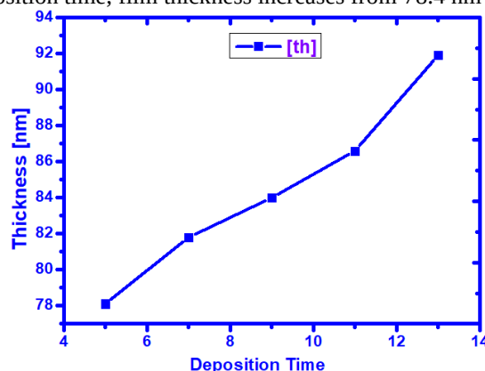
Fig. 3 Effect of deposition times on the deposited SiN x films thickness.
