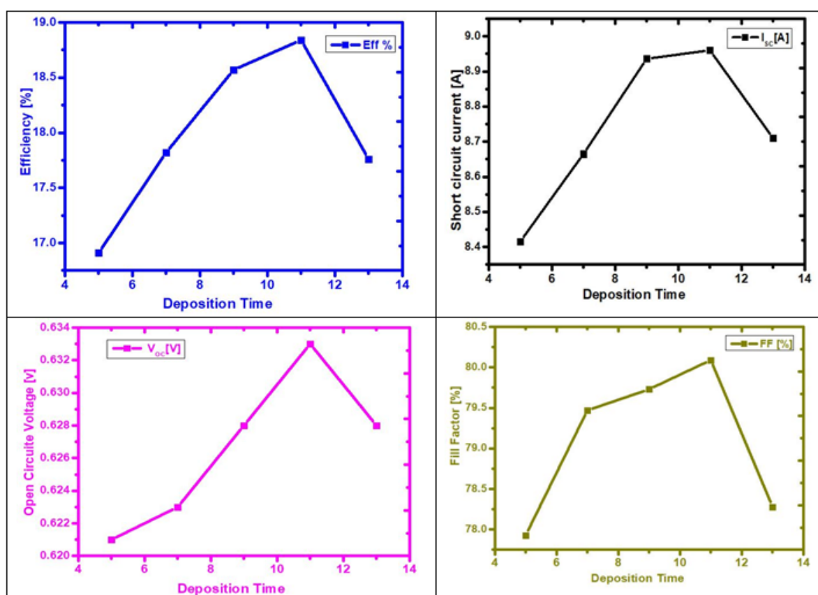
Fig. 8. Dependence of the solar cells parameters on the SiN x film deposition time.
