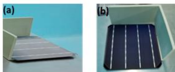
Fig.10. The image of monocrystalline Si solar cells (a) without SiN x film (b) with SiN x film.
