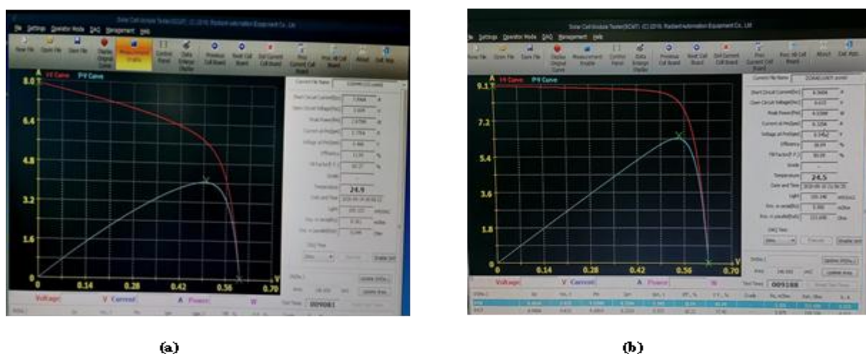
Fig.11. I-V and P-V curves of the solar cell (a) without SiN x film and (b) with SiN x film.
