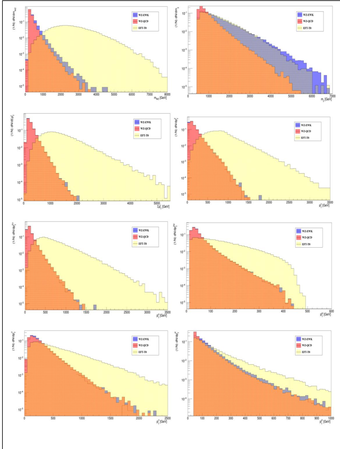
Figure 2: Kinematical variables used as input to the ML models. From top left to right m_{WZ} , m_{jj} , \Sigma p_T^l , p_T^Z , p_T of the highest p_T (leading) lepton, p_T of the second highest p_T (sub-leading) lepton, p_T of the leading jet ( p_T^{j1} ) and p_T of the sub-leading jet ( p_T^{j2} ). Shape comparison between the SM QCD and EWK produced W^\pm Zjj processes and the one with non-zero Wilson coefficient for the O_{T0} operator.
