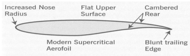
Fig.1: super critical aerofoil
