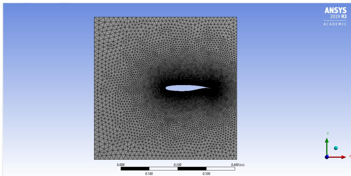
Fig.6: mesh generation
