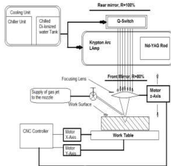
Fig.2 Schematic Representation of DPSS Nd:YAG Laser system Setup
