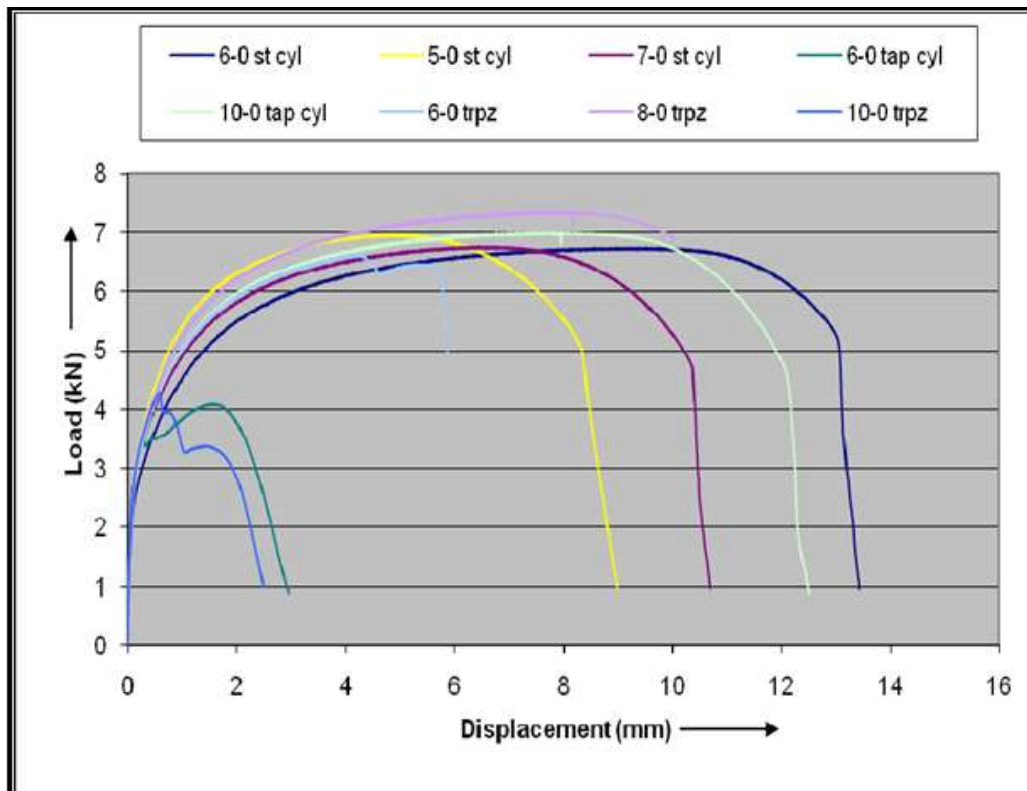
Figure 4.2: Tensile testing results of the FSW tools.
