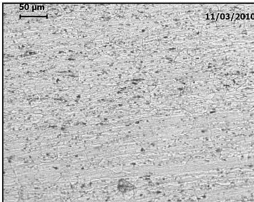
Figure 4.8: HAZ microstructure of 10 mm probe diameter trapezoidal tool.
