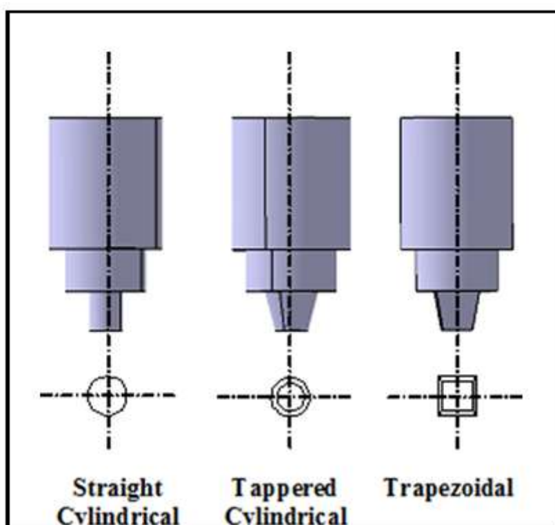
Figure 1.4: Tool Probe Profiles.
