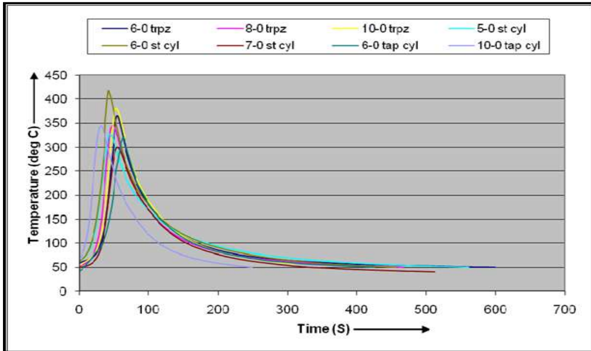
Figure 4.3: Temperature distribtuion results.
