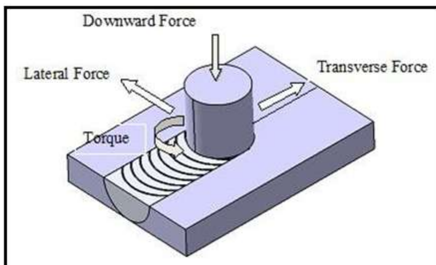
Figure 1.3: Forces acting on FSW Tool.
