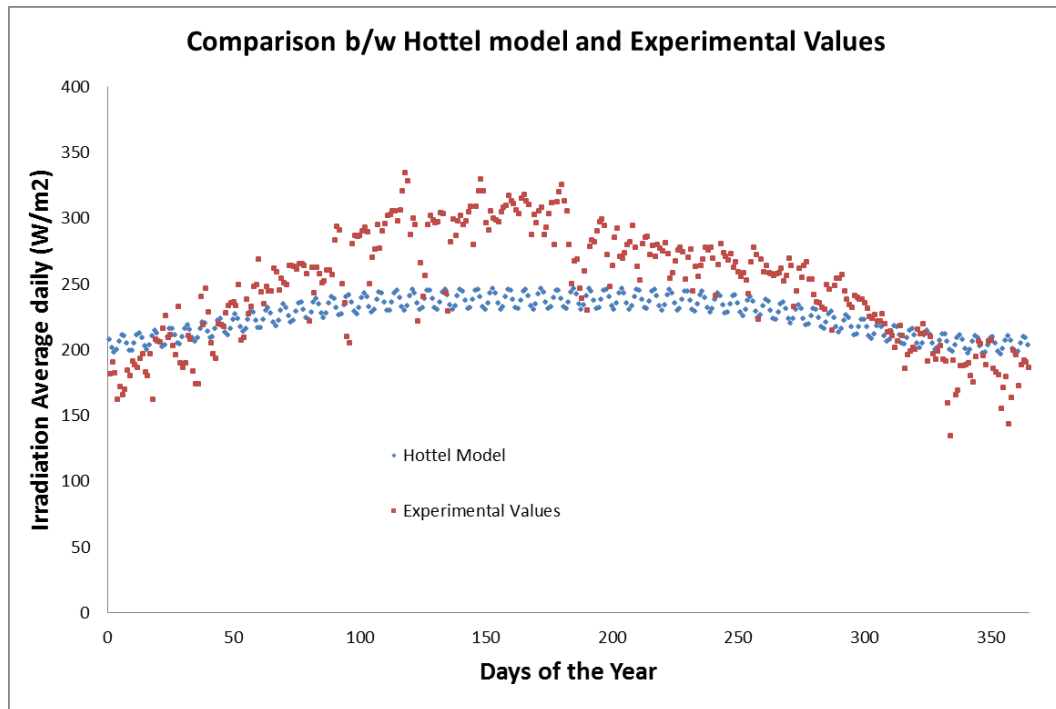
Fig.2 Comparison between Hottel's model and Experimental values
