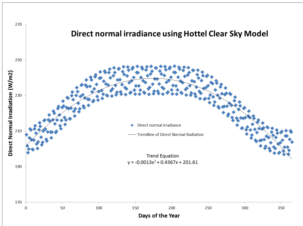
Fig.1 Hottel Clear sky Model for Jeddah
