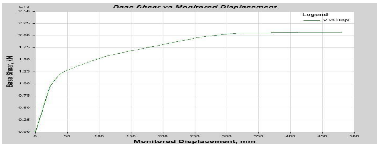
Fig 3.1 Push-Over curve of the model 3 bare frame G+3 building
