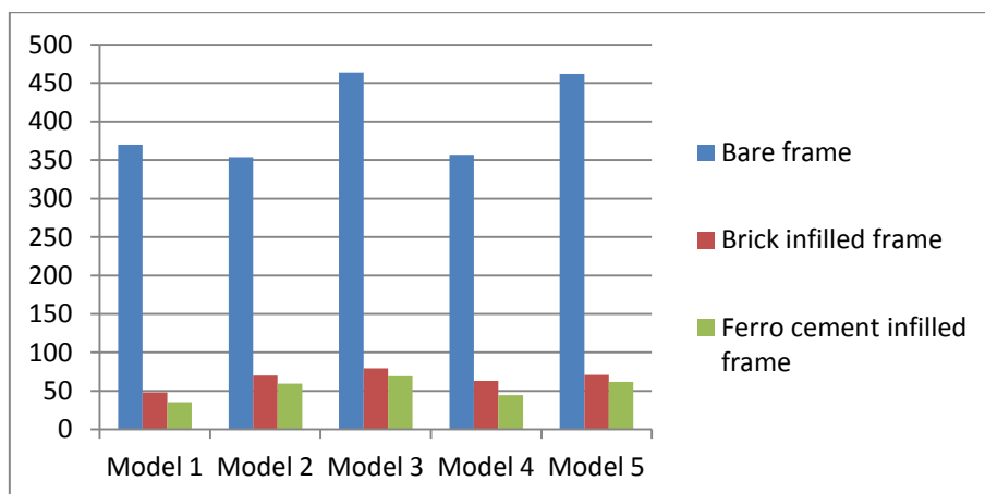
DISPLACEMENT GRAPH OF G+3 IN mm
