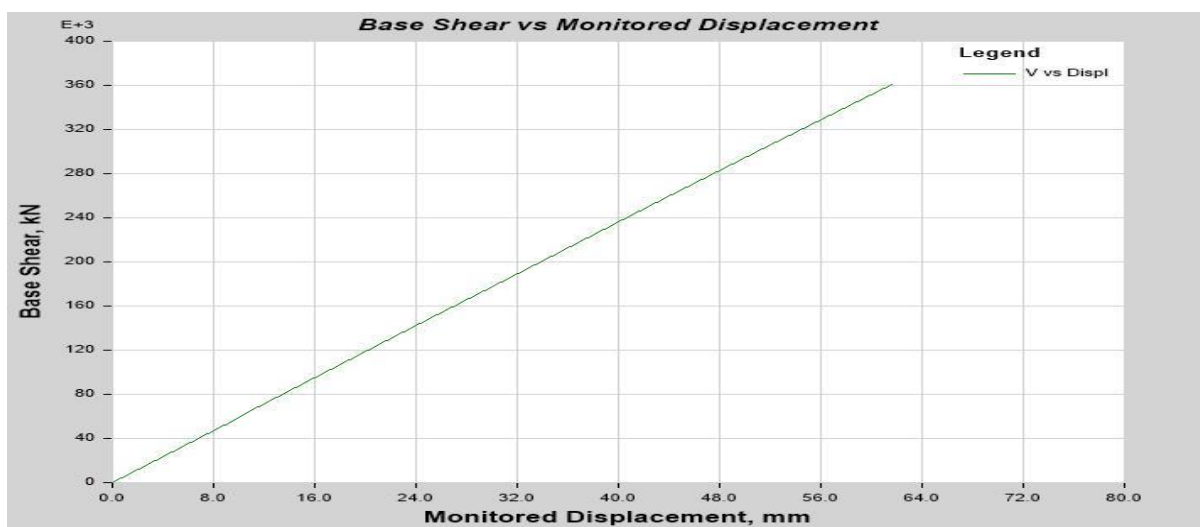
Fig 3.6 Push-Over curve of the Ferro cement infilled frame G+3 building model 5
