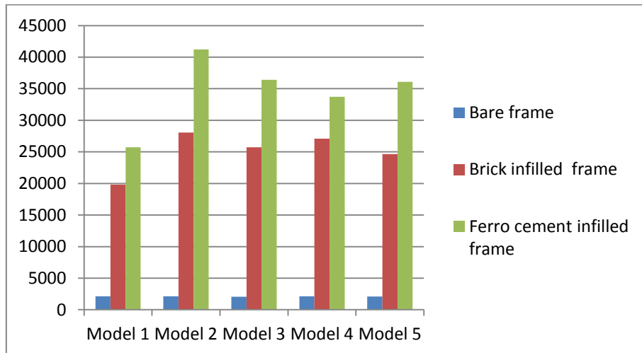
BASE SHEAR GRAPH OF G+3 IN kN
