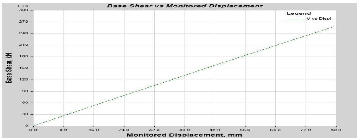
Fig 3.3 Push-Over curve of the brick infilled frame G+3 building model 3
