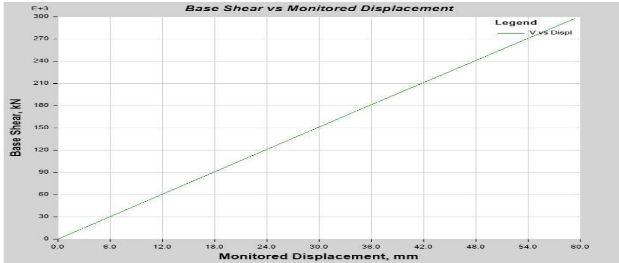
Fig 3.8 push-Over curve of the Ferro cement infilled frame G+9 building model 5
