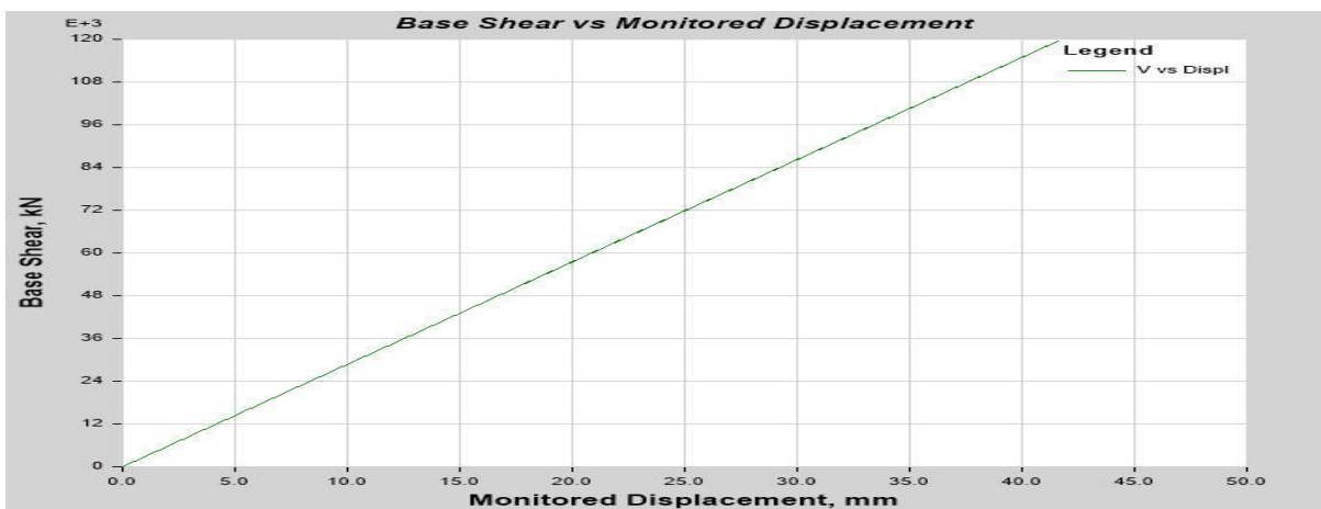
Fig 3.4 Push-Over curve of the brick infilled frame G+9 building model 3
