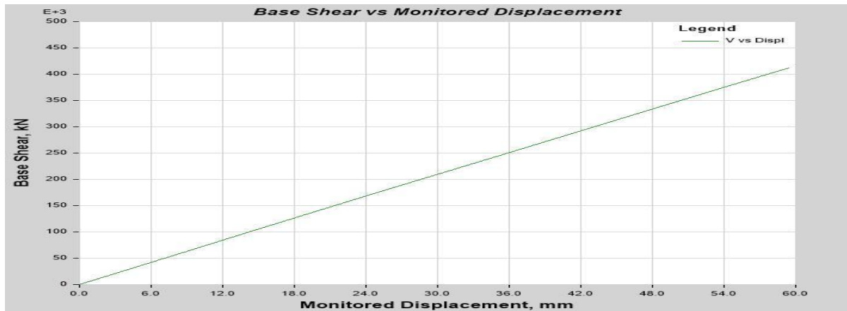
Fig 3.5 Push-Over curve of the Ferro cement infilled frame G+3 building model 3
