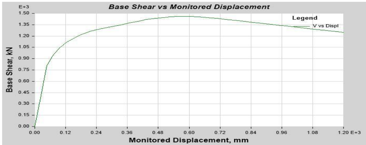
Fig 3.2 Push-Over curve of the model 3 bare frame G+9 building
