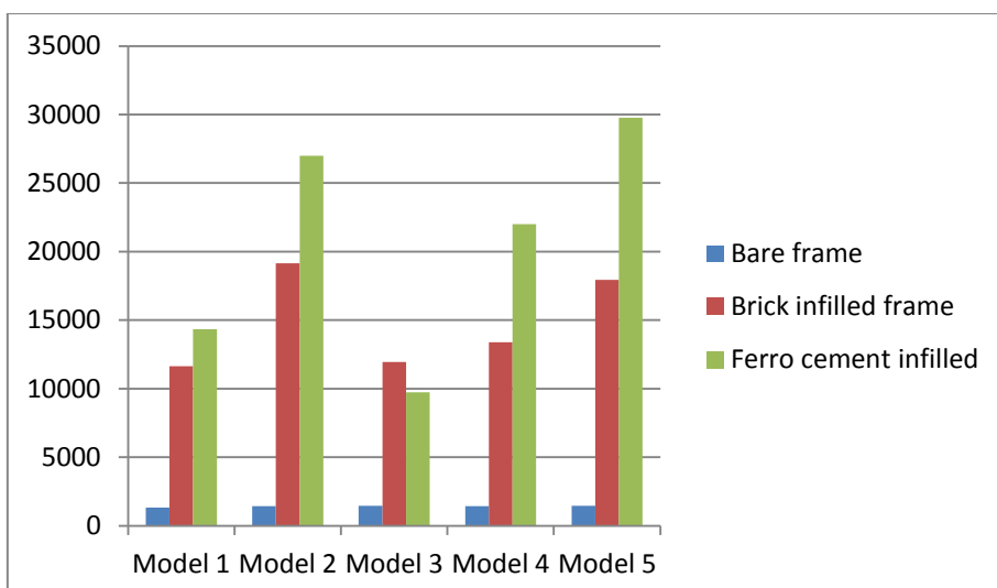
BASE SHEAR GRAPH OF G+9 IN kN
