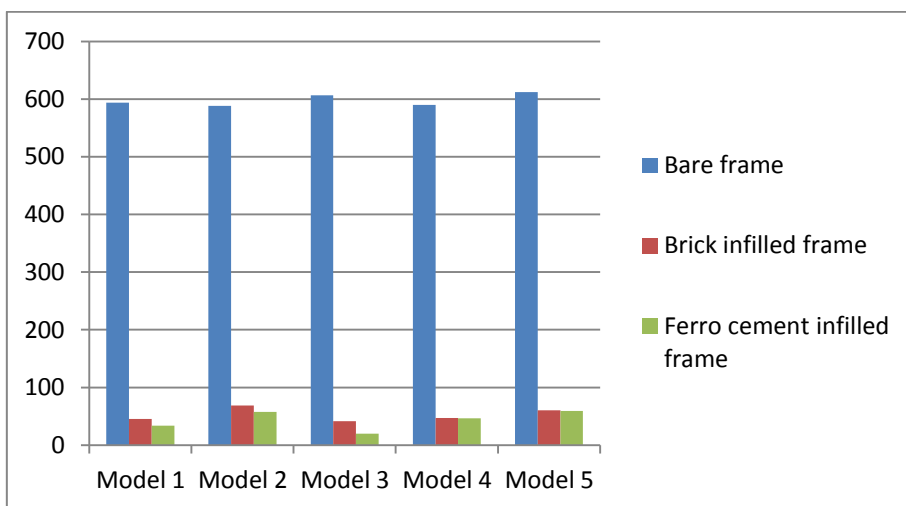
DISPLACEMENT GRAPH OF G+9 IN mm
