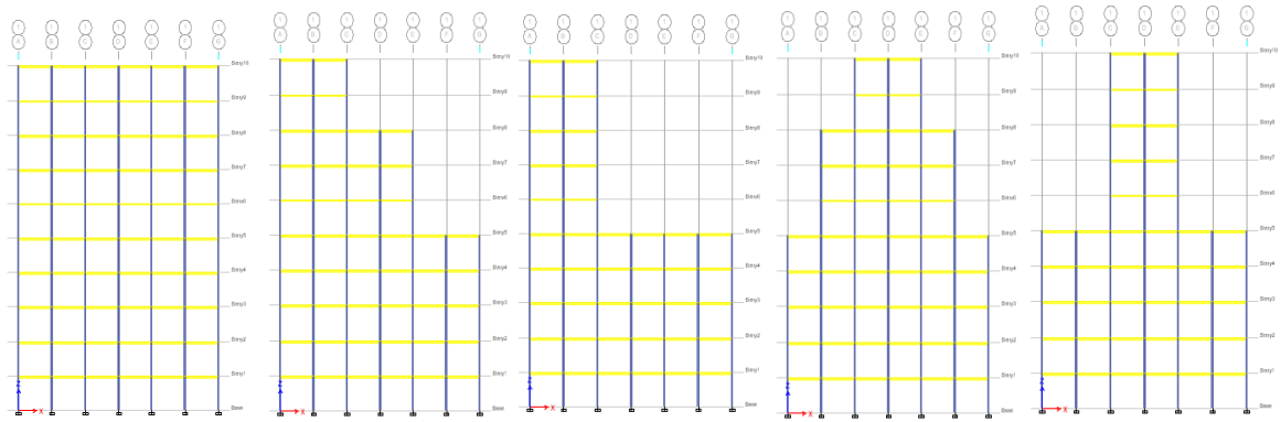
Fig 2.5 G+9 Bare frame Elevation view
