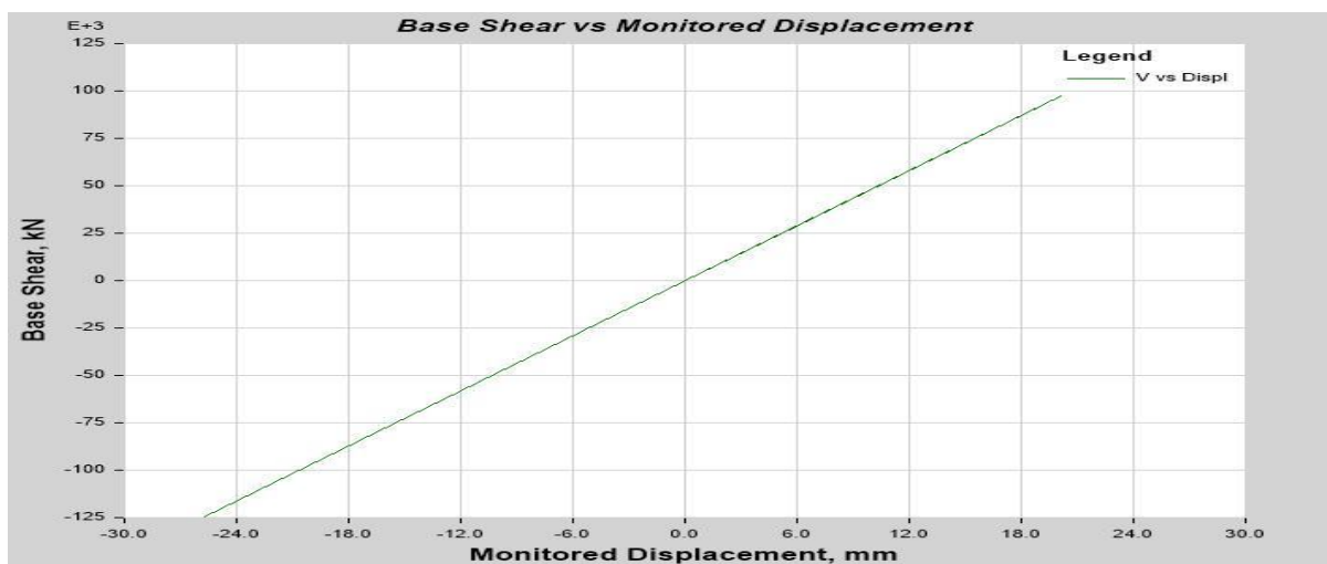
Fig 3.7 Push-Over curve of the vertical Ferro cement frame G+9 building model 3
