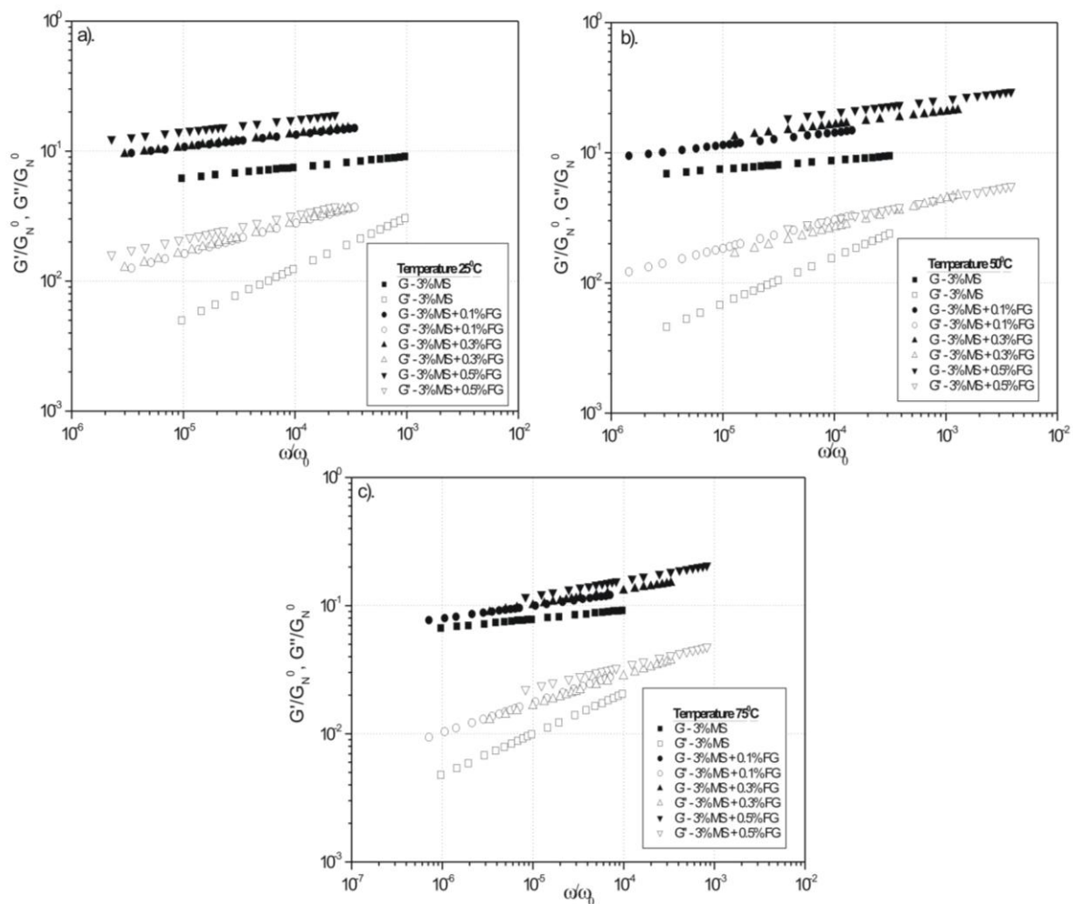
Fig. 5. Reduced curves of maize starch and flaxseed gum mixture at changing flaxseed gum concentration.
