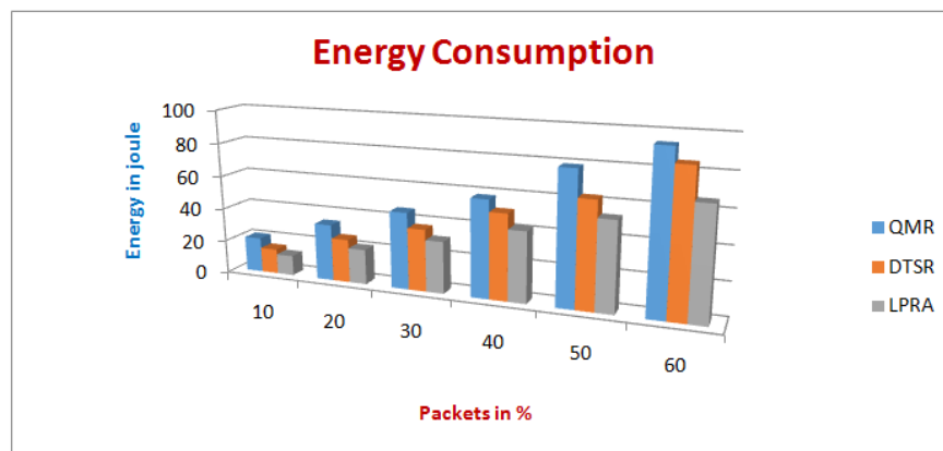
Fig 6: Comparison of Energy consumption on network
