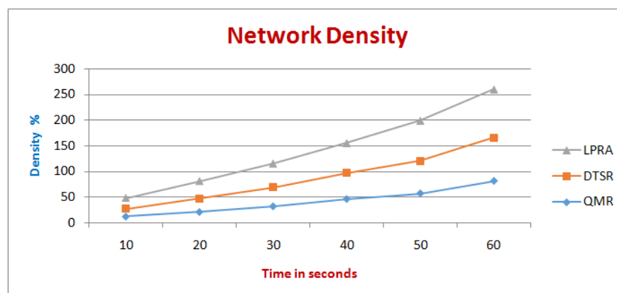
Fig 7: Network density model on network
