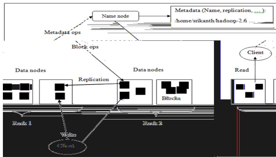
Figure 2. HDFS Architecture
